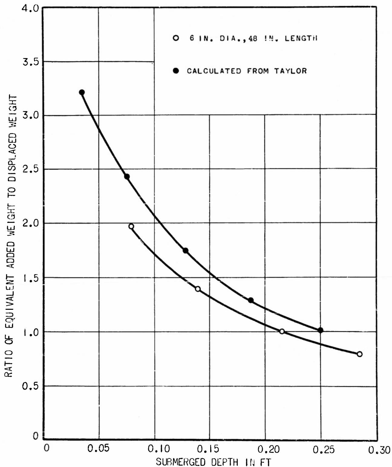
FIG. 20. RATIO OF EQUIVALENT ADDED WEIGHT TO DISPLACED WEIGHT AND SUBMERGENCE FOR SEMICIRCULAR PONTON
