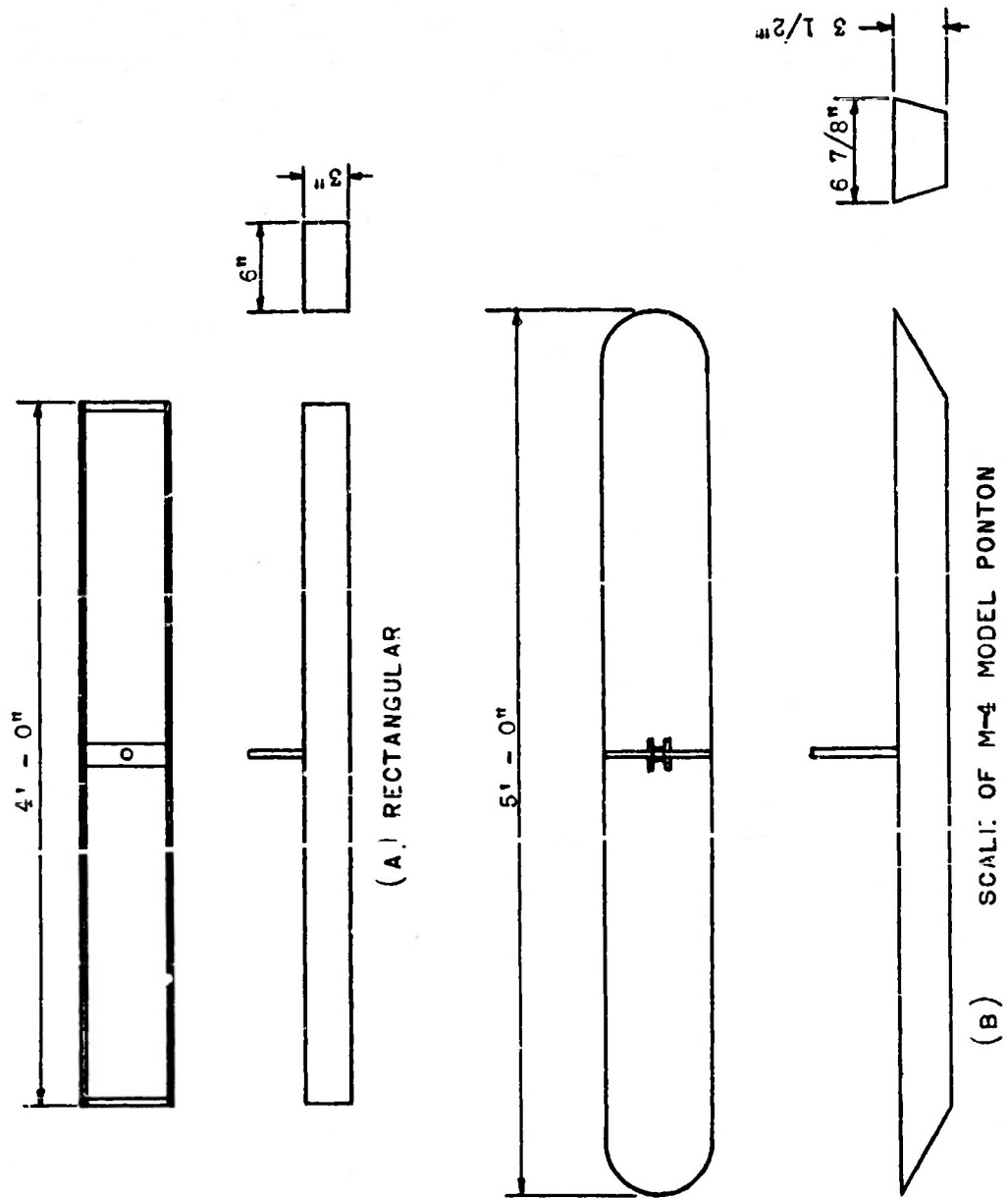
FIG. 5 MODEL PONTONS
