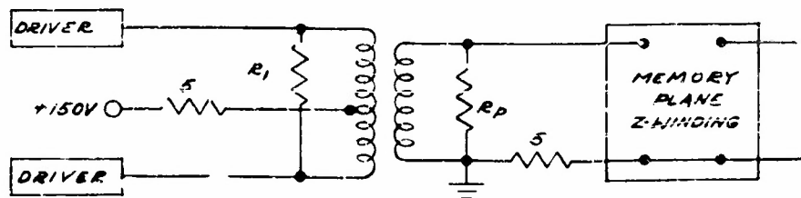
FIG. 3 ELECTRICAL CIRCUIT FOR FIG. 5-B
