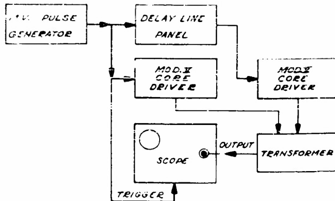
FIG. 2 TEST SET-UP
