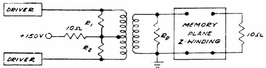
FIG. 2 TEST SET-UP
