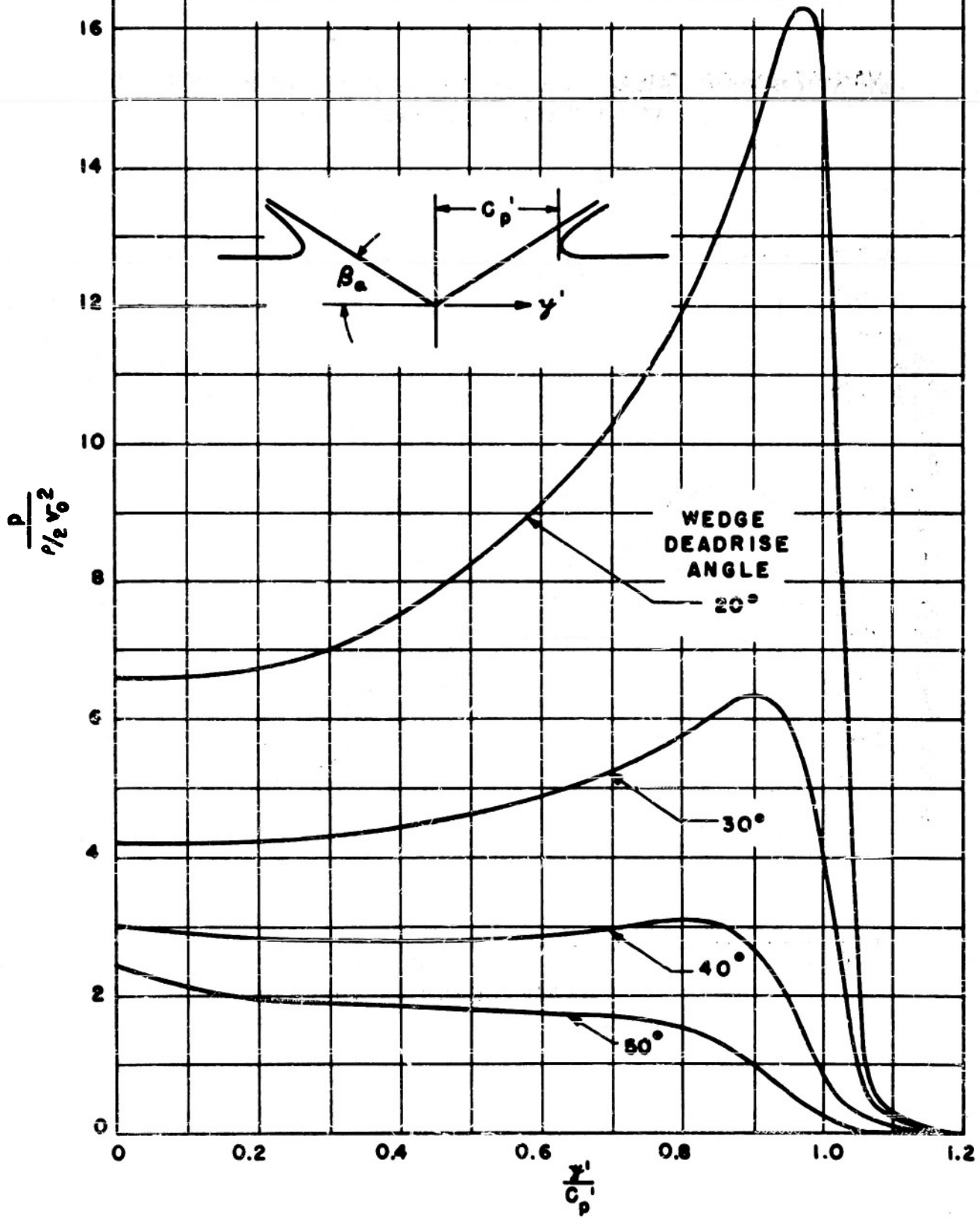
FIGURE 12 PRESSURE DISTRIBUTION OVER IMMERSED WEDGE (CURVES REPRODUCED FROM REFERENCE 1)
