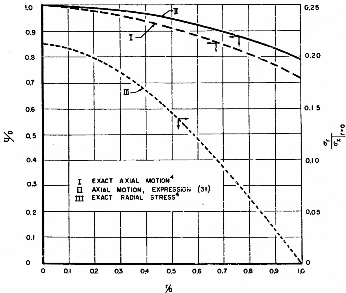
Fig. 2 - Variation of longitudinal motion and radial stress with radius for a/\Lambda = 0.196 .
