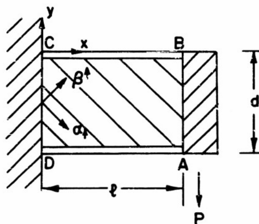
Fig. 11 Tension-field beam with no stiffeners
