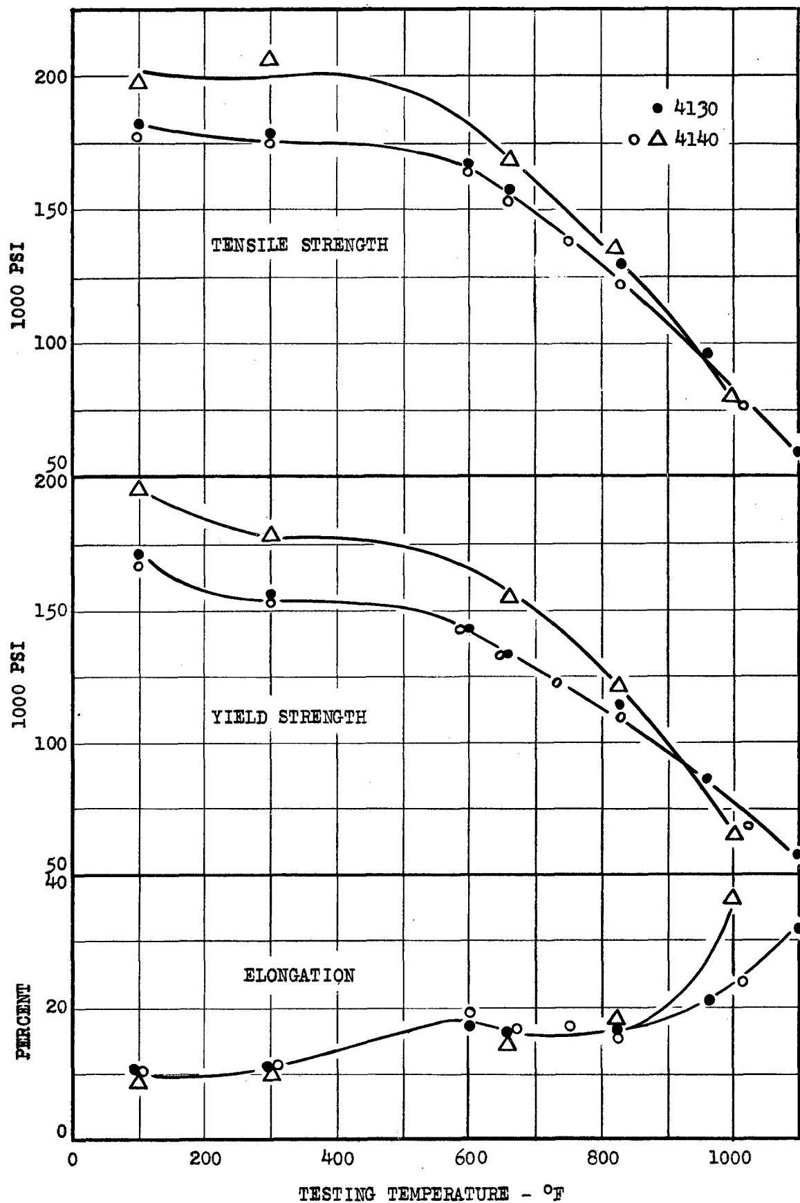
FIG. 45 SHORT-TIME TENSION CHARACTERISTICS OF 4130 AND 4140 STEEL AT ELEVATED TEMPERATURES. (DATA BY NORTH AMERICAN)
