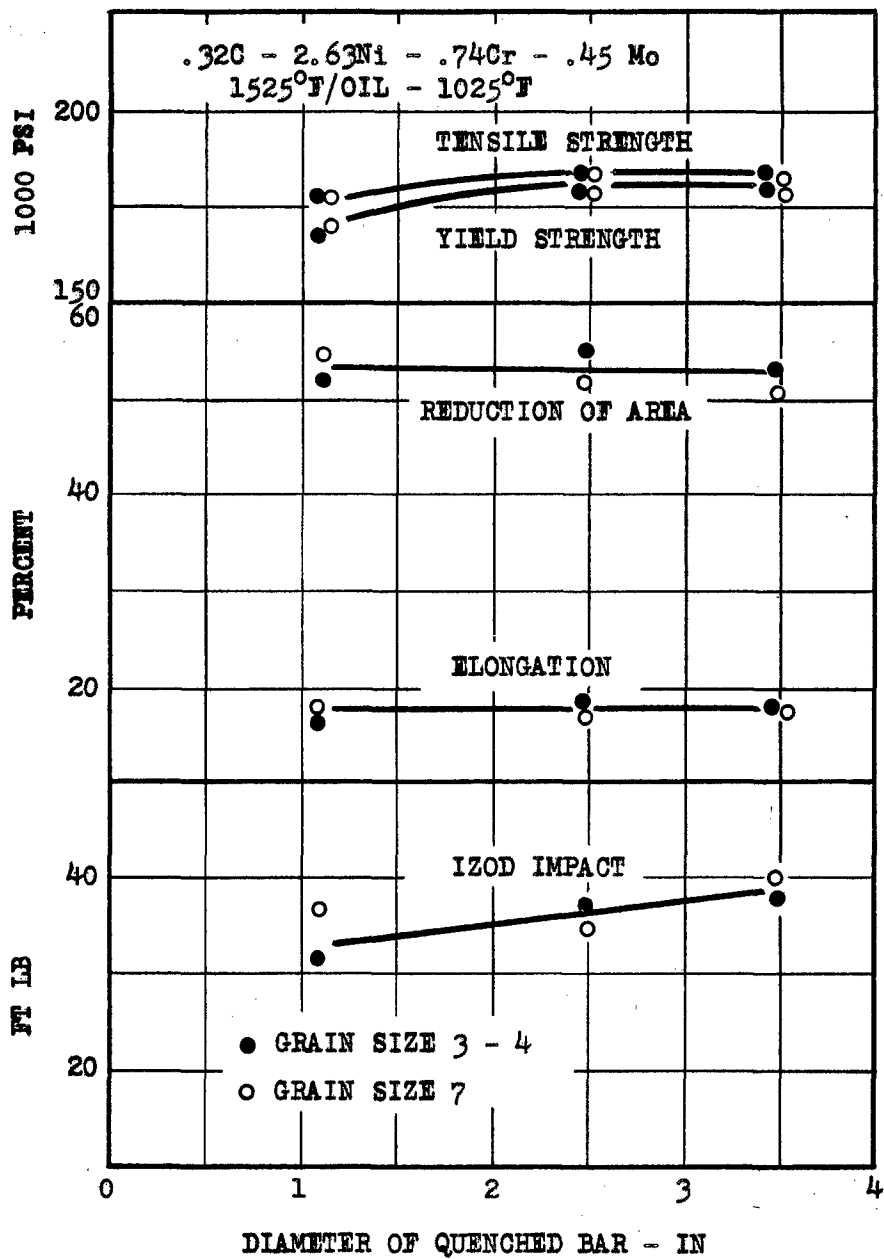
FIG. 28 EFFECT OF AS-QUENCHED SECTION SIZE AND AUSTENITIC GRAIN SIZE ON TENSION CHARACTERISTICS OF A DEEP-HARDENING NICKEL-CHROMIUM-MOLYBENDUM STEEL. (DATA BY SWINDEN, BOLSOVER 1936)
