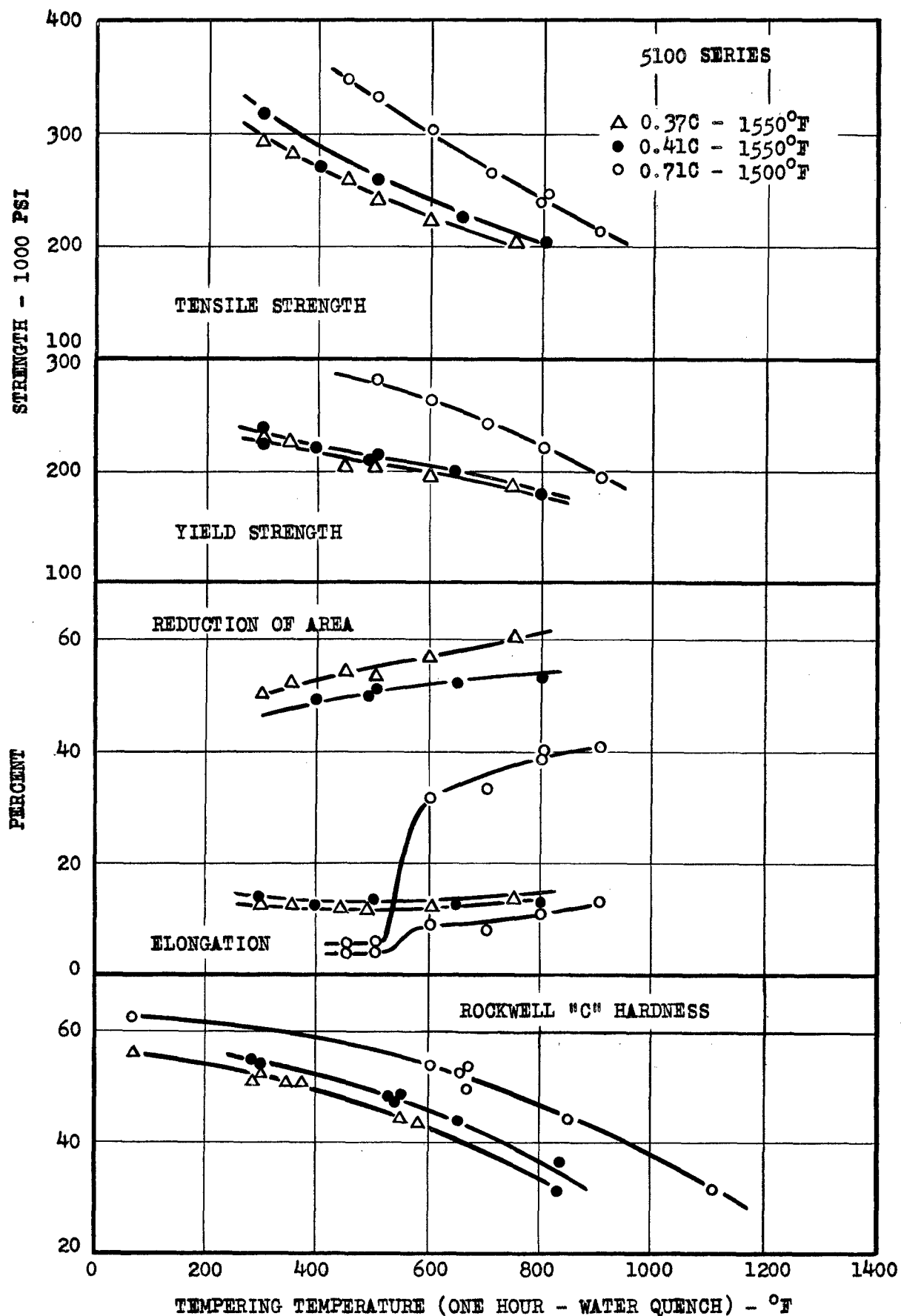
FIG. 14 EFFECT OF TEMPERING TEMPERATURE ON TENSION CHARACTERISTICS OF BRINE-AND-CAUSTIC-SODA-QUENCHED 5100 STEELS.
