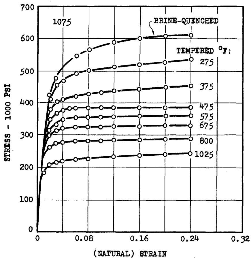
FIG. 56 COMPRESSION TEST DATA FOR 0.75% CARBON ALLOY STEEL. (MARKUS, MC GAUGHEY 1948)
