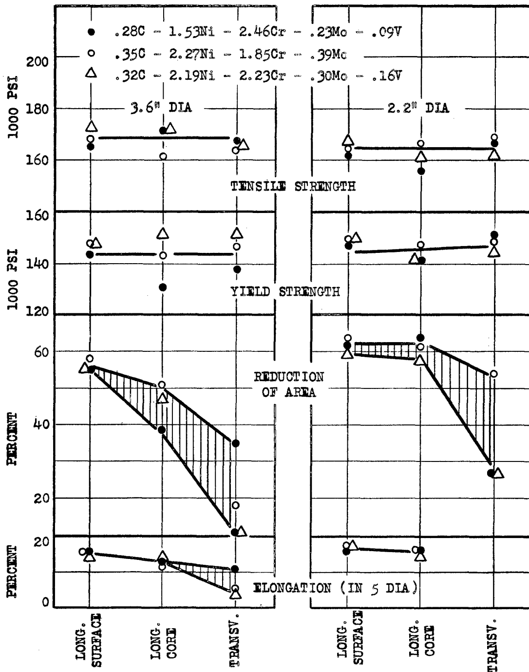
FIG. 22 EFFECT OF POSITION AND DIRECTION OF TEST BAR ON TENSION CHARACTERISTICS OF THREE DEEP-HARDENING LOW-ALLOY STEELS. (DATA BY POMP, KRISCH 1942)
