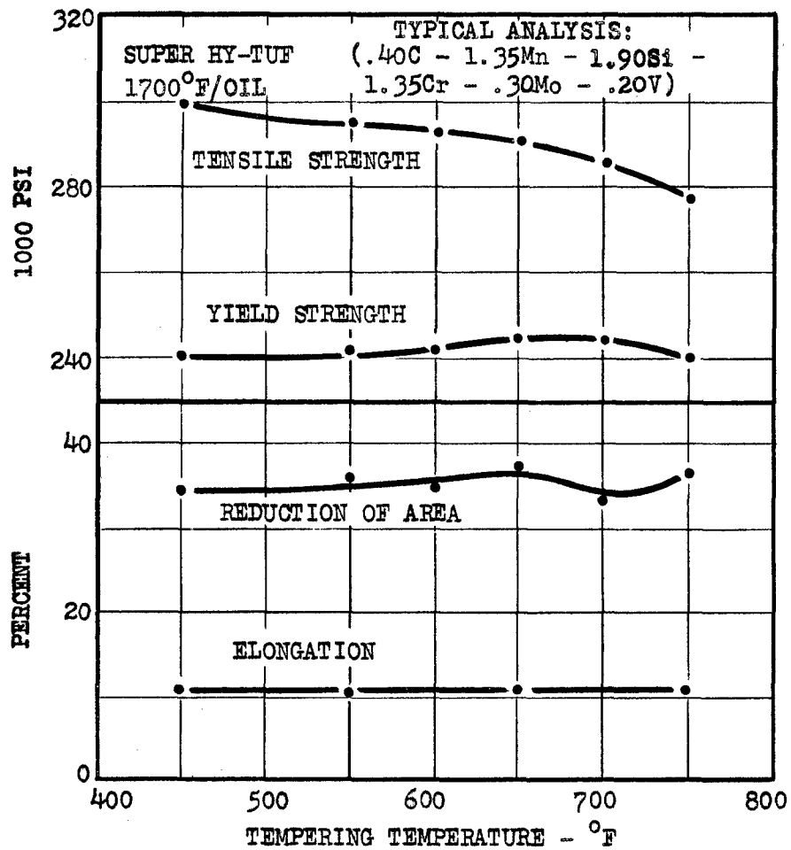
FIG. 10-e EFFECT OF TEMPERING TEMPERATURE ON THE TENSION CHARACTERISTICS OF A LOW-ALLOY STEEL. (CRUCIBLE STEEL)
