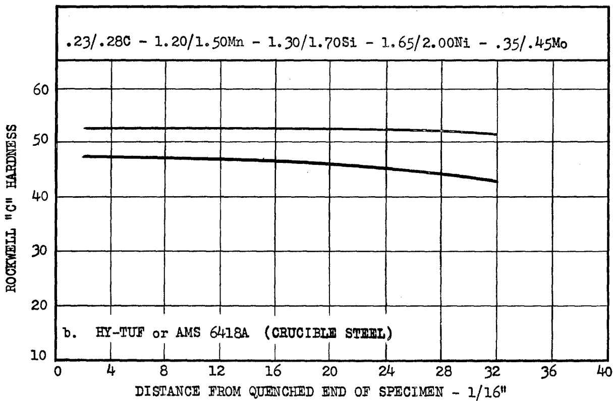
FIG. 4a-b SOME HARDENABILITY DATA FOR RECENTLY DEVELOPED AIRCRAFT STEELS.
