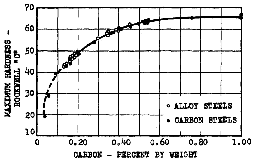
FIG. 7 IDEAL RELATION BETWEEN AS-QUENCHED HARDNESS AND CARBON CONTENT.
