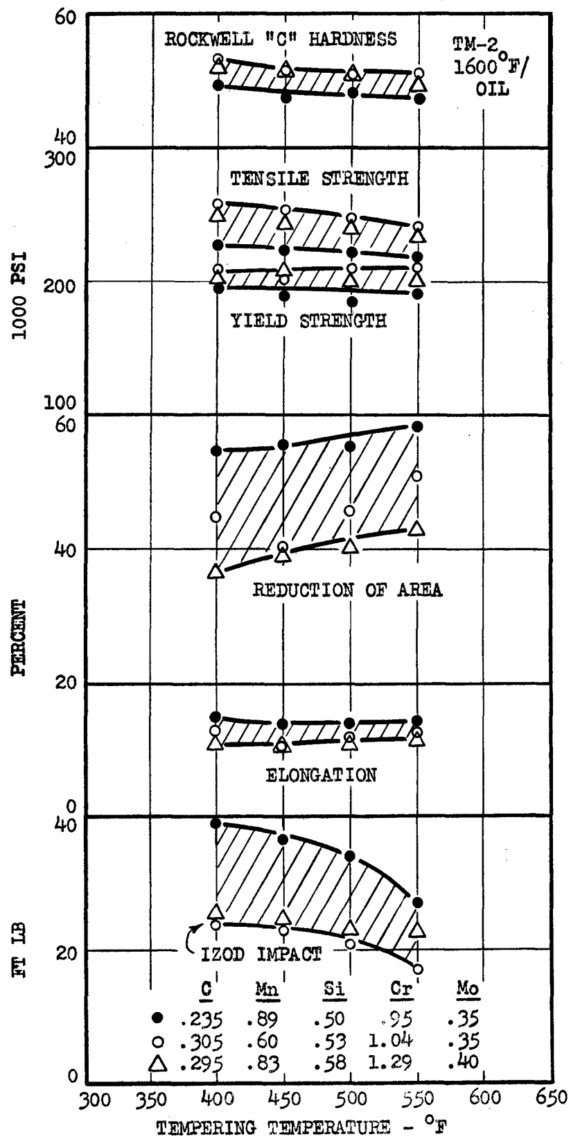
FIG. 10-c EFFECT OF TEMPERING TEMPERATURE ON THE TENSION CHARACTERISTICS OF A LOW-ALLOY STEEL. (TIMKEN)
