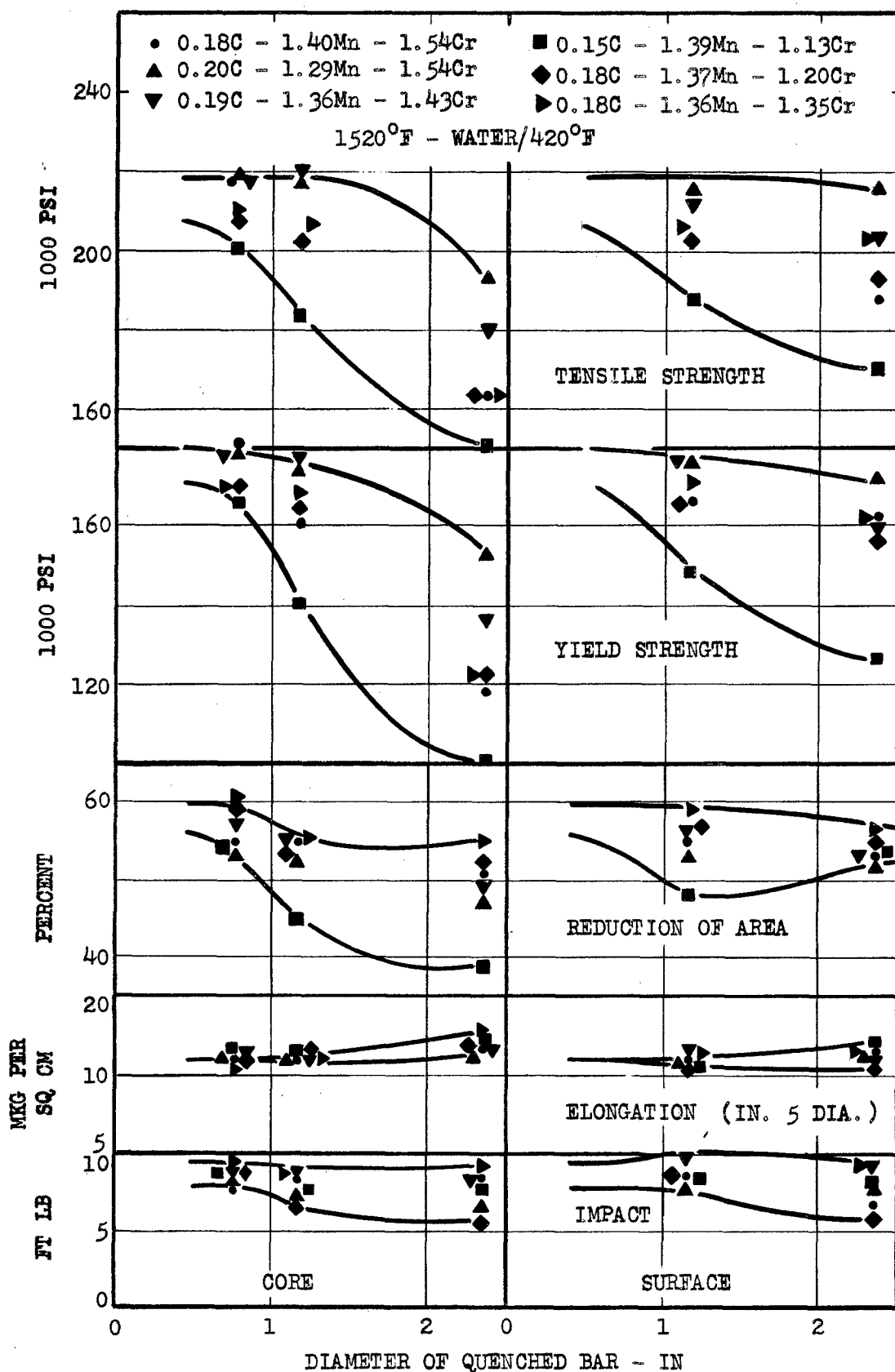
FIG. 30 EFFECT OF AS-QUENCHED SECTION SIZE ON TENSION CHARACTERISTICS OF SIX HEATS OF A LOW-ALLOY STEEL FROM DIFFERENT PRODUCERS.
