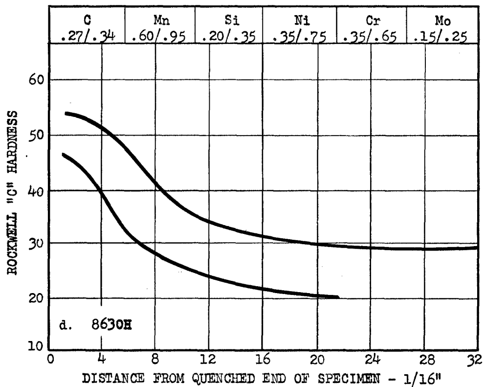
FIG. 3c-d HARDENABILITY BANDS FOR SOME STANDARD AIRCRAFT STEELS. (AISI)
