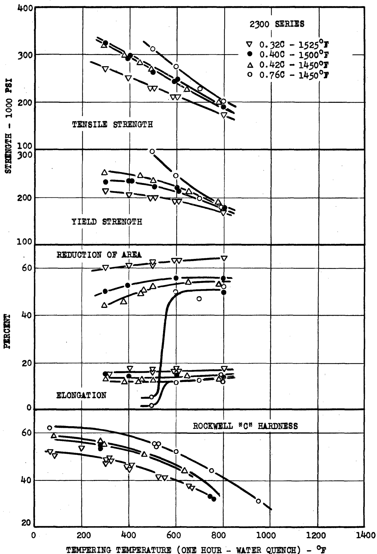
FIG. 15 EFFECT OF TEMPERING TEMPERATURE ON TENSION CHARACTERISTICS OF BRINE-AND-CAUSTIC-SODA-QUENCHED 2300 STEELS.
