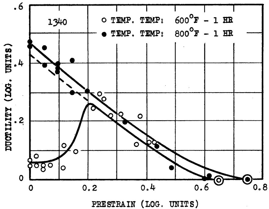
FIG. 54 EFFECT OF TEMPERING TEMPERATURE ON THE RELATION BETWEEN PRESTRAINING AT ROOM TEMPERATURE AND DUCTILITY AT -320°F.
