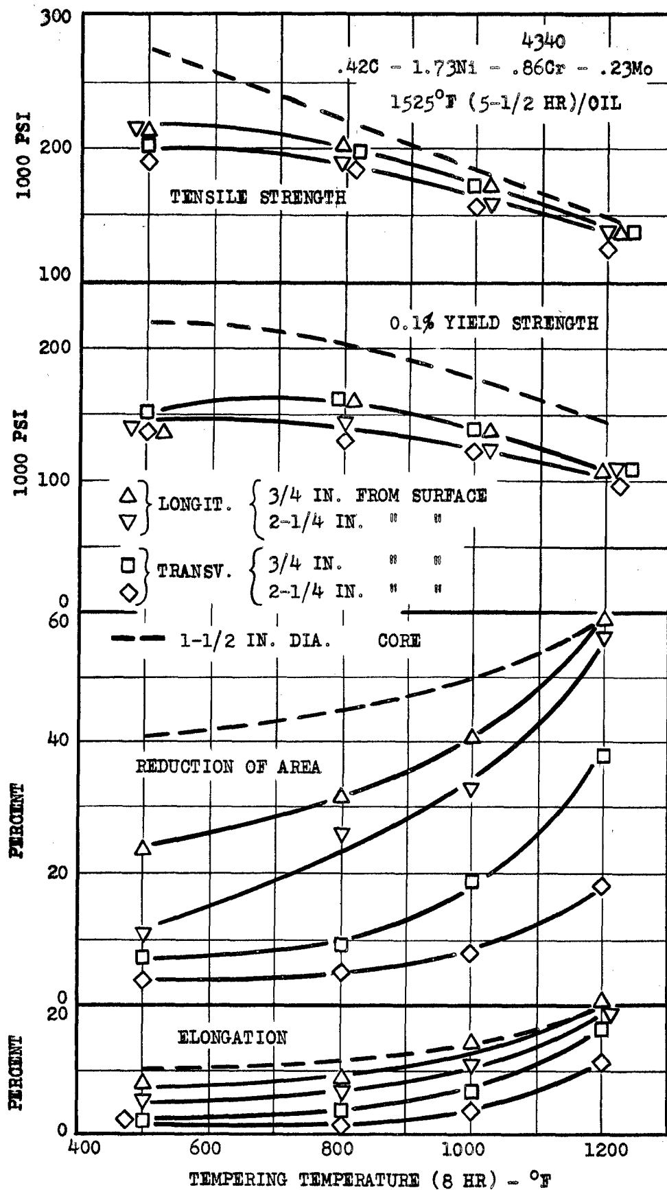
FIG. 25 TENSION CHARACTERISTICS OF A HEAT-TREATED 6 IN. SQUARE 4340 STEEL BILLET.
