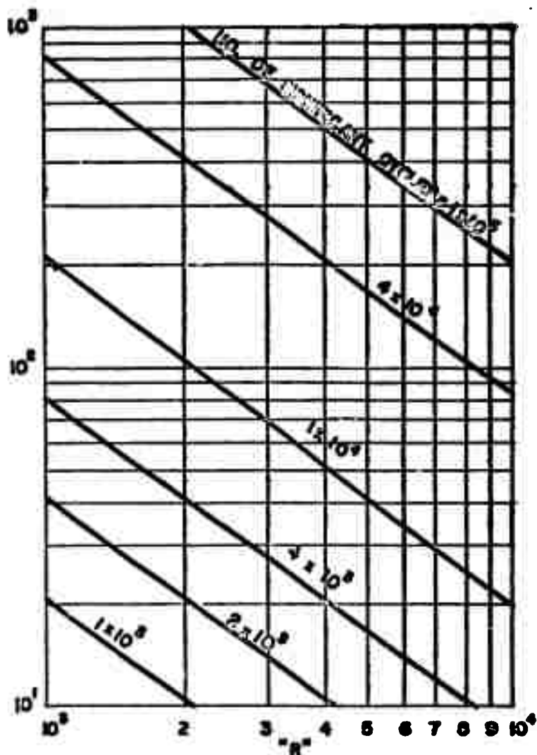
FIGURE 13C. TOTAL NUMBER OF SWEEPS IN VIBRATION TEST FOR VARIOUS VALUES OF PARAMETER R AND SIGNIFICANT CYCLES.
