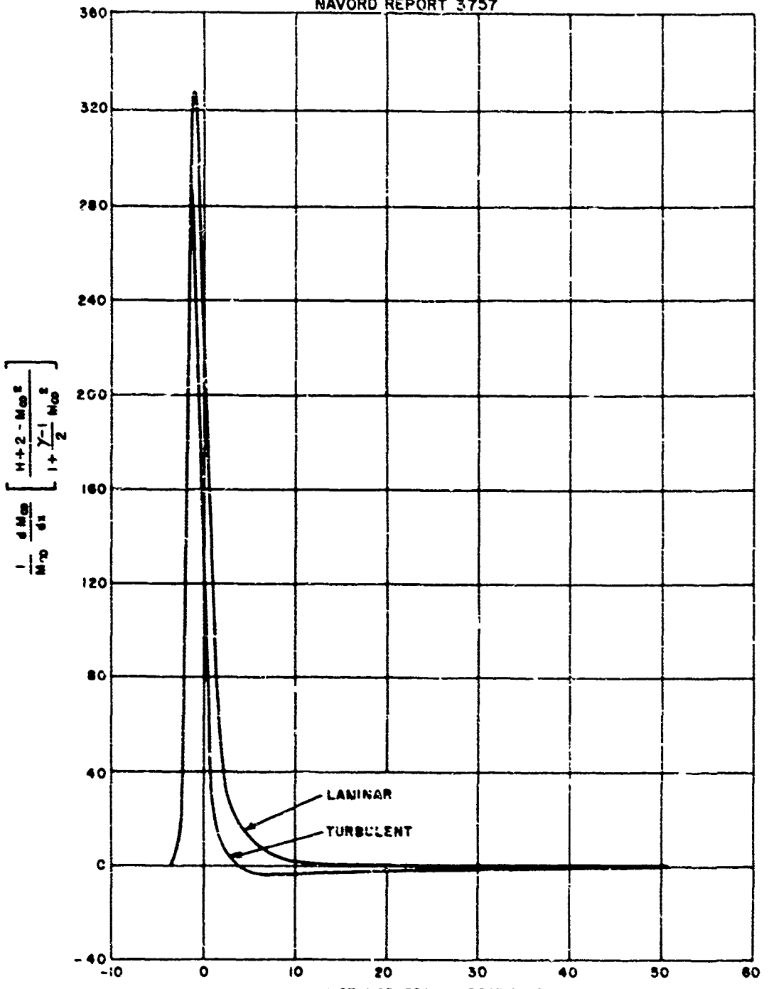
FIG. 6 VARIATION OF \frac{1}{M^2} \frac{dM}{dx} \left[ \frac{H+2-M^2}{1+\frac{\gamma-1}{2}M^2} \right]
