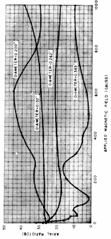
FIGURE 6 MICROWAVE PROPERTIES OF FERRIMIC A-106, WITH DIAMETER AS PARAMETER TEMPERATURE = 21°C (73°F) FREQUENCY = 9600 MC LENGTH = 3.00"
