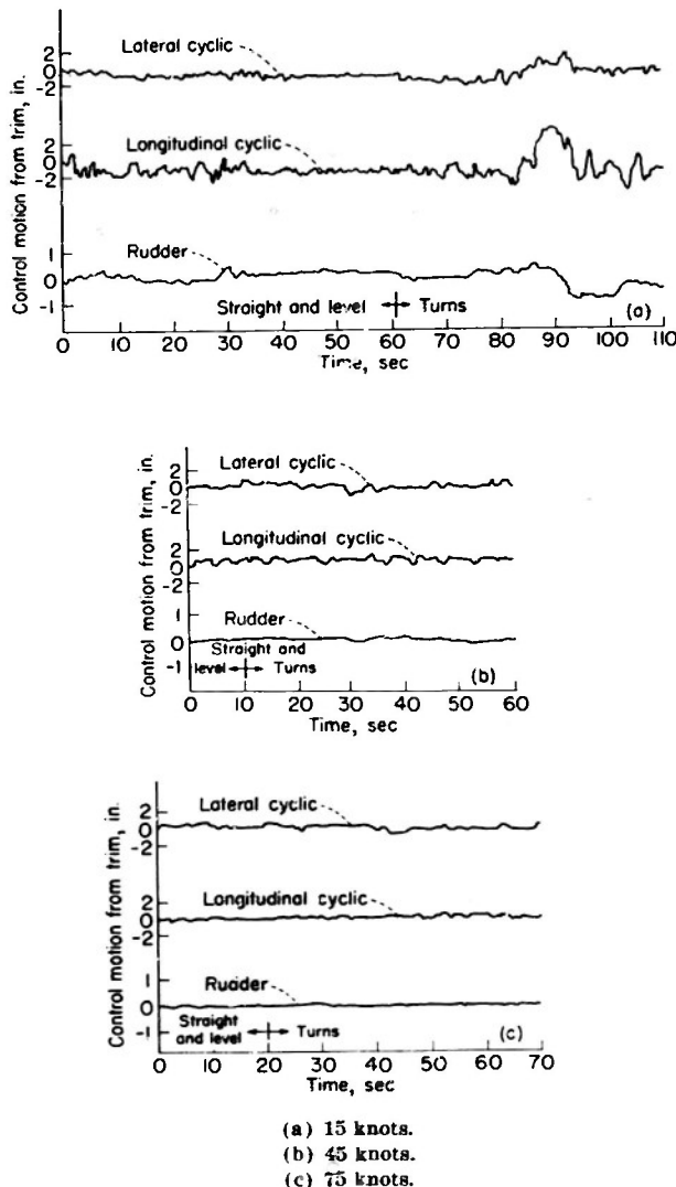
FIGURE 8.—Comparison of control motion at various airspeeds during level-flight-plus-turn maneuvers, tail-on configuration.
