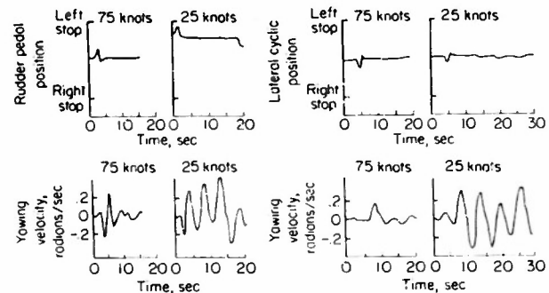
FIGURE 7.—Oscillations resulting from control displacements at two different airspeeds.
