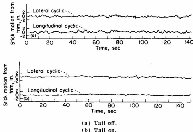
FIGURE 5.—Comparison of cyclic control motion, tail on and tail off, during level-flight-plus-turn maneuver at 75 knots.
