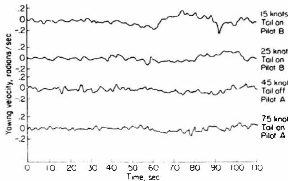
FIGURE 6.—Yawing-velocity variations during level-flight-plus-turn maneuvers.
