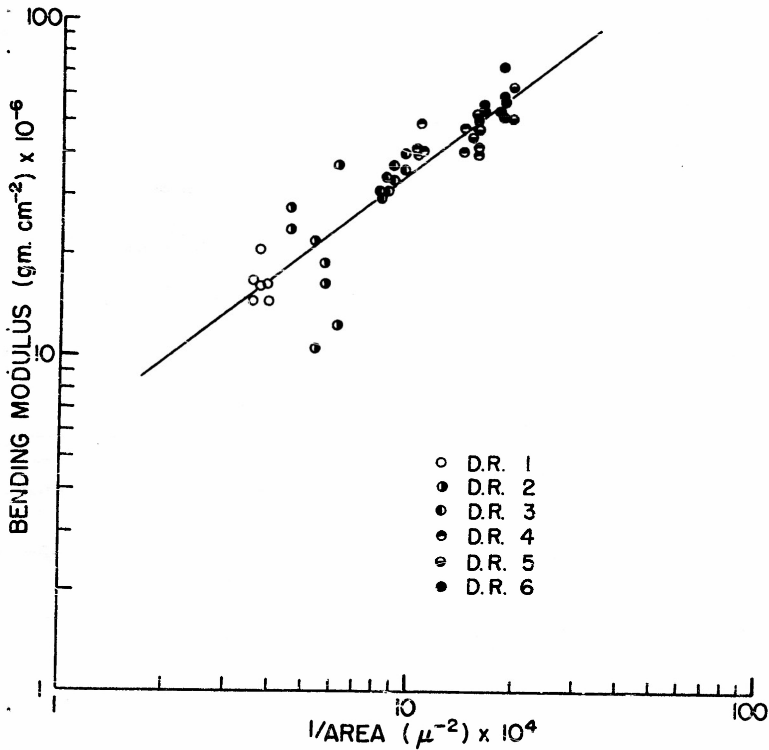
Fig. 9. Bending modulus of nylon 66 vs. reciprocal cross-sectional area of filaments at various draw ratios.
