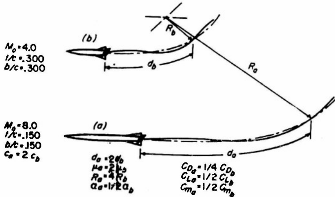
FIGURE 3.—Related wing-body combinations at hypersonic speeds.
