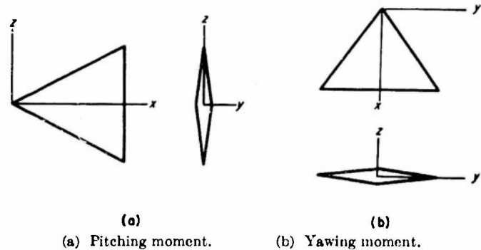
FIGURE 2.—Bodies excluded from similarity considerations as applied to pitching and yawing moments.
