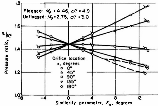
FIGURE 8.—Variation of pressure ratio, P/P_0 , with K_a , for two cones tested at K_t = 0.91 .
