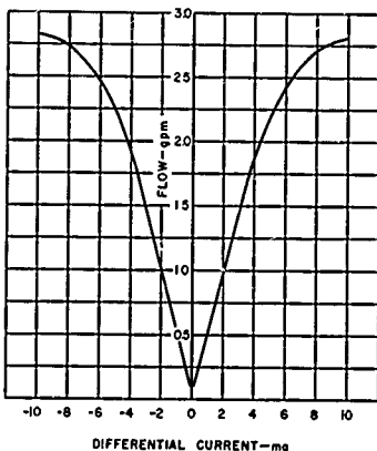
Figure 7. Typical Flow Characteristics, SV-9C Valve
