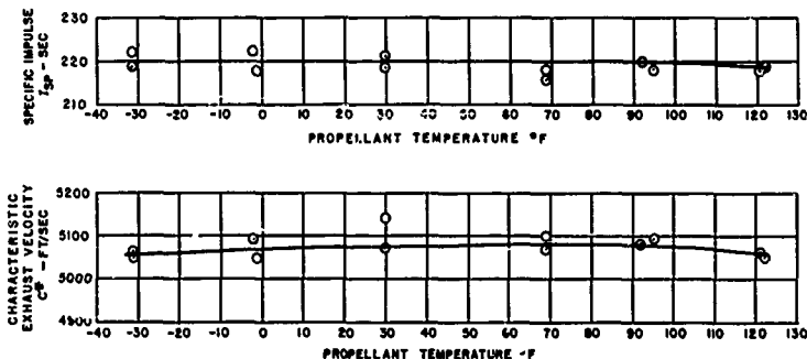
Figure 9. Performance of 75L* Tubular Thrust Chamber Assembly
