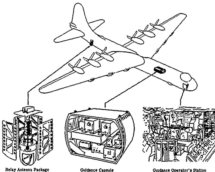
Figure 22. Model 110 Guidance System in DB-36
