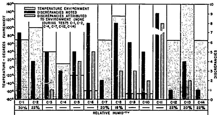
Figure 27. Temperature Test Results
