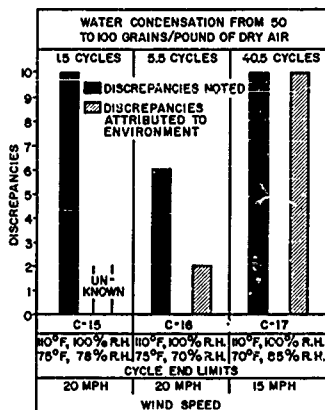
Figure 28. Humidity Test Results
