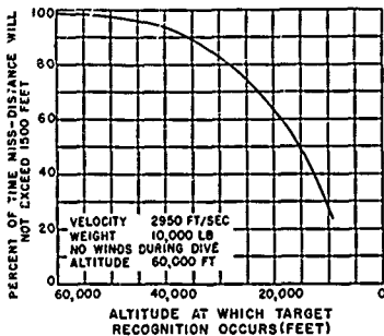
Figure 14A. Accuracy vs. Altitude of Target Recognition
