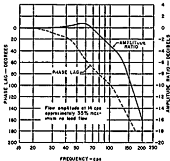
Figure 8. Frequency Response Curves, SV-9C Valve
