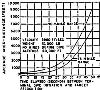
Figure 14B. Miss-Distance vs. Time of Target Recognition
