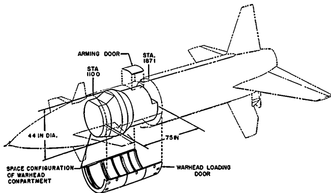
Figure 15. B-63 Warhead Compartment
