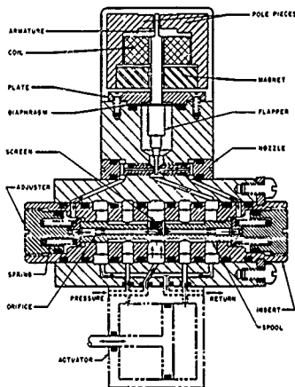
Figure 6. Schematic Cross-Section of "C" Valve
