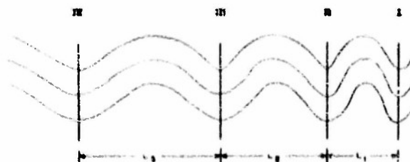
Figure 2b. Hypothetical long-wave pattern as seen on the 500-mb chart with wave length increasing upstream.
