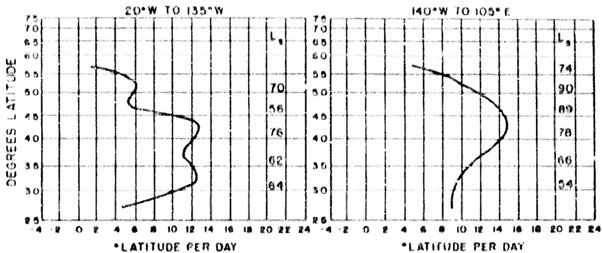
Figure 5a. Zonal wind profile and stationary wave lengths, 0600 GCT, 15 December 1950.
