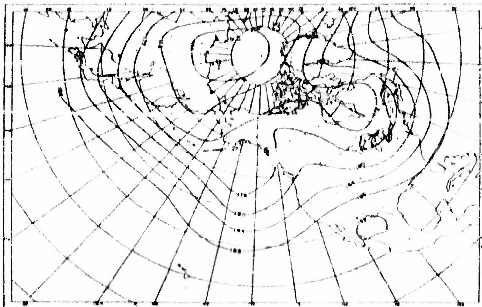
Figure 5d. Space-mean 500-mb chart, 0300 GCT, 16 December 1950.
