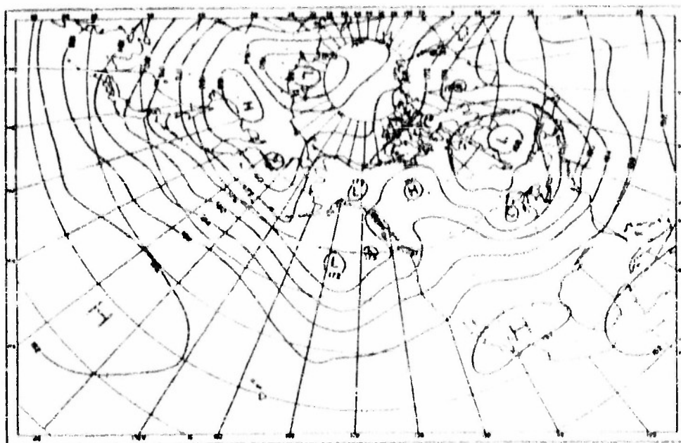
Figure 5b. 500-mb chart, 0600 GCT, 15 December 1950.
