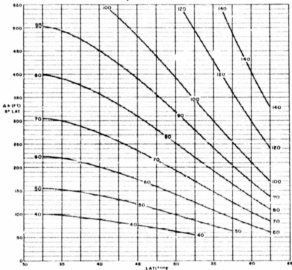
Figure A3. Stationary wave length (standing waves) as a function of the average height difference across 5° of latitude ( \Delta h ) and of the latitude.
