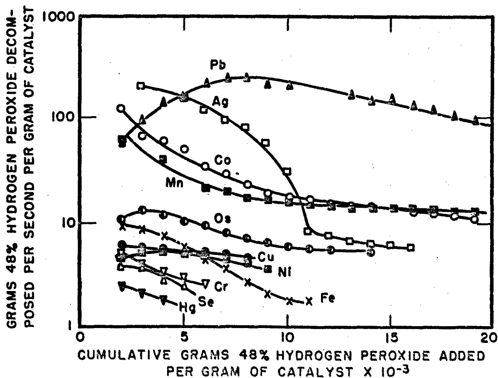
FIG. 5 - RELATIVE CATALYTIC ACTIVITY OF SOME METAL HYDROXIDES (FORMED FROM 0.0118g. METAL + 10cc. 4NNaOH).
