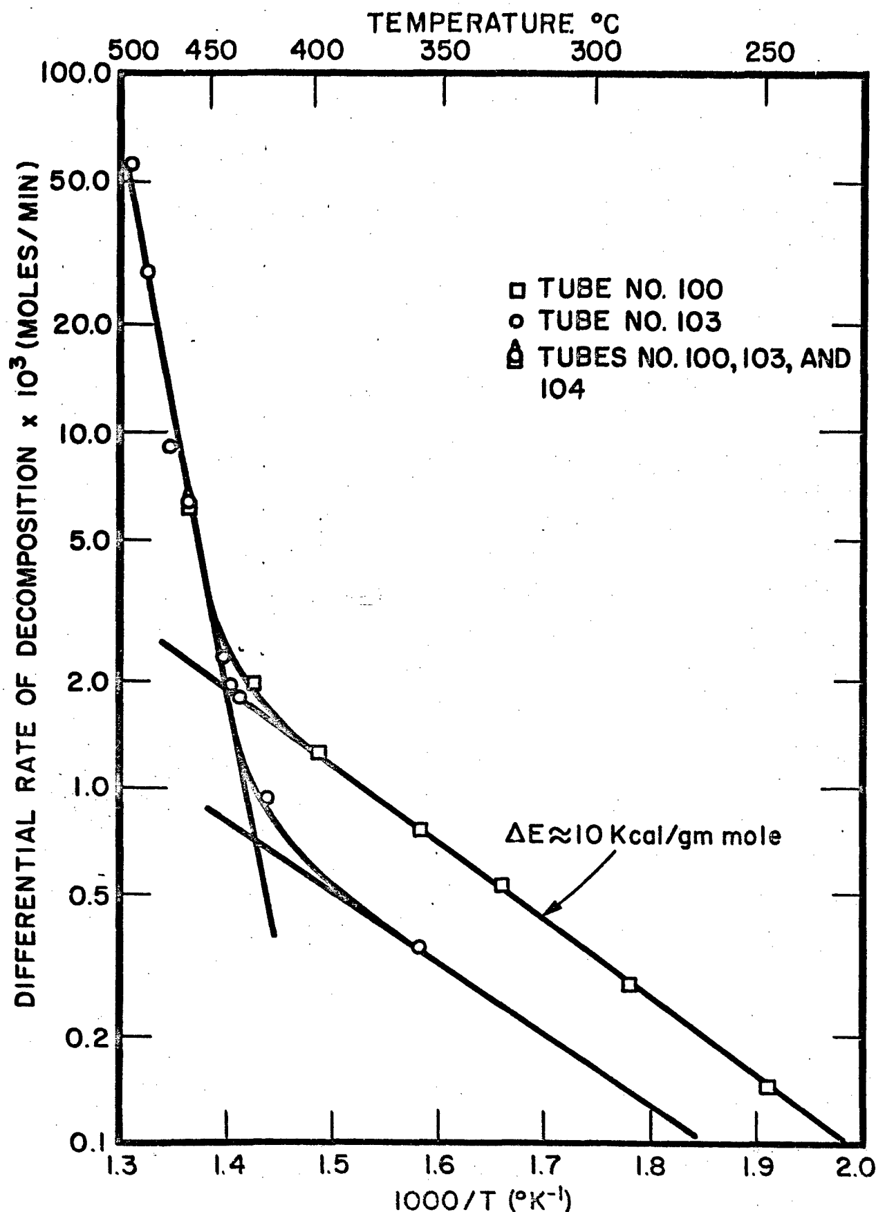
FIG. 1 - EFFECT OF TEMPERATURE ON THE DECOMPOSITION OF HYDROGEN PEROXIDE VAPOR. ( p_{\text{H}_2\text{O}_2} = 0.02 \text{ ATM.} )
