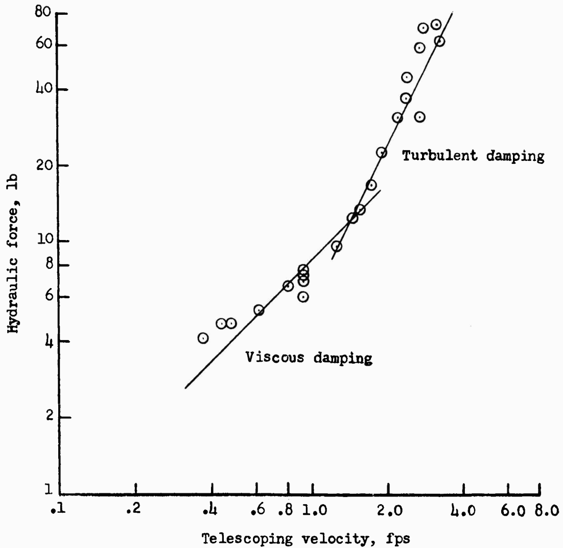
(c) Hydraulic force against telescoping velocity. Drop weight, 11.57 lb; drop height, 4 in.
