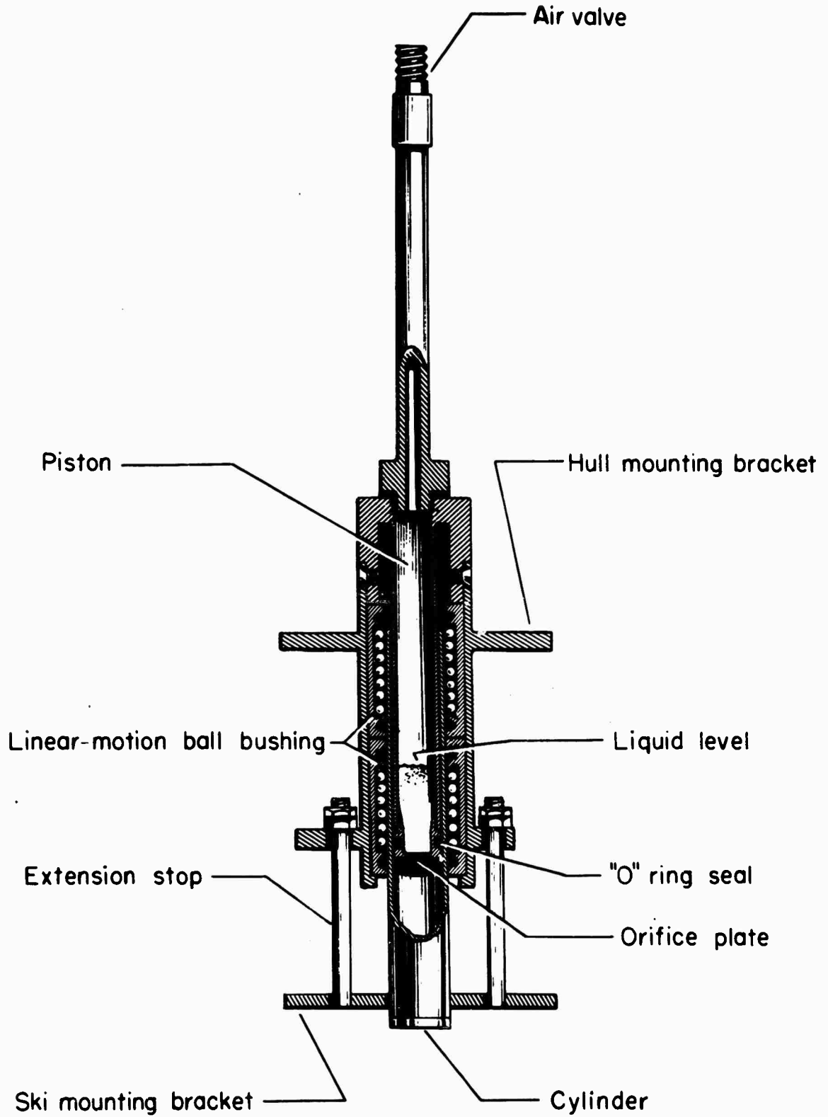
Figure 6.- Shock-absorber strut.
