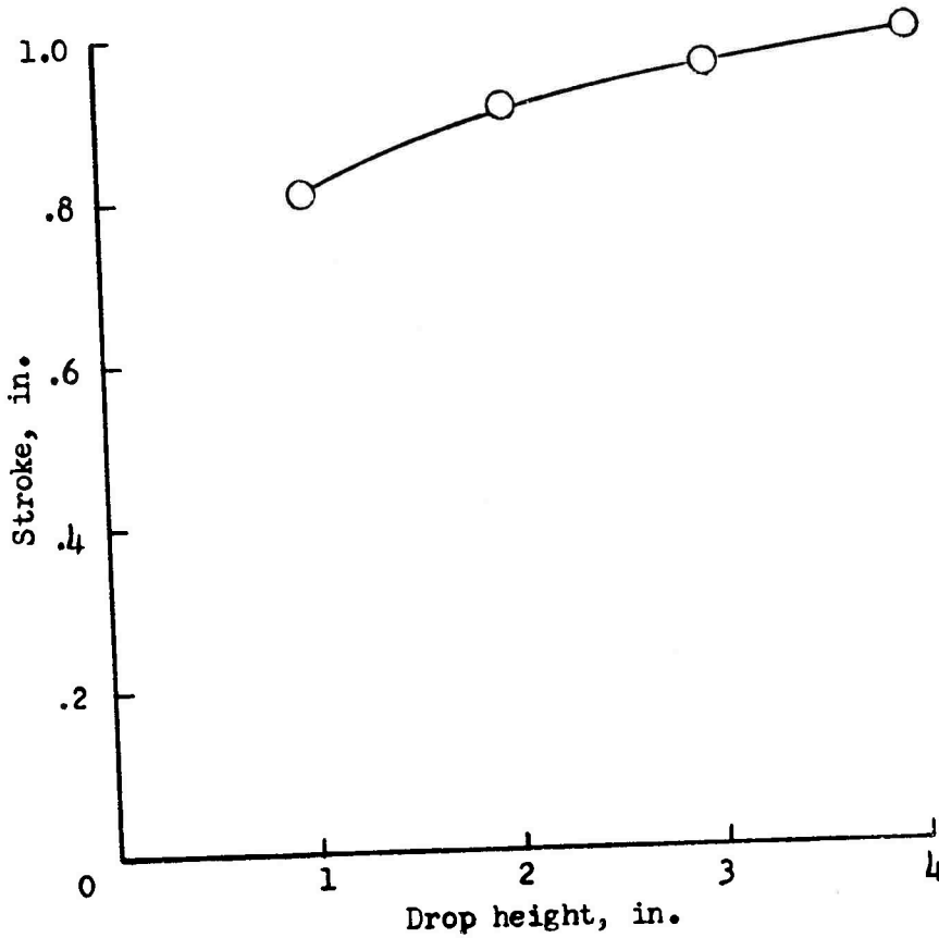
(b) Stroke-drop height diagram for a drop weight of 11.57 pounds. Figure 7.- Shock-absorber characteristics obtained from bench tests.
