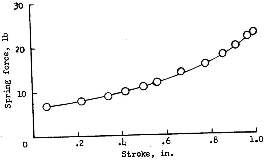
(a) Force-stroke diagram.
