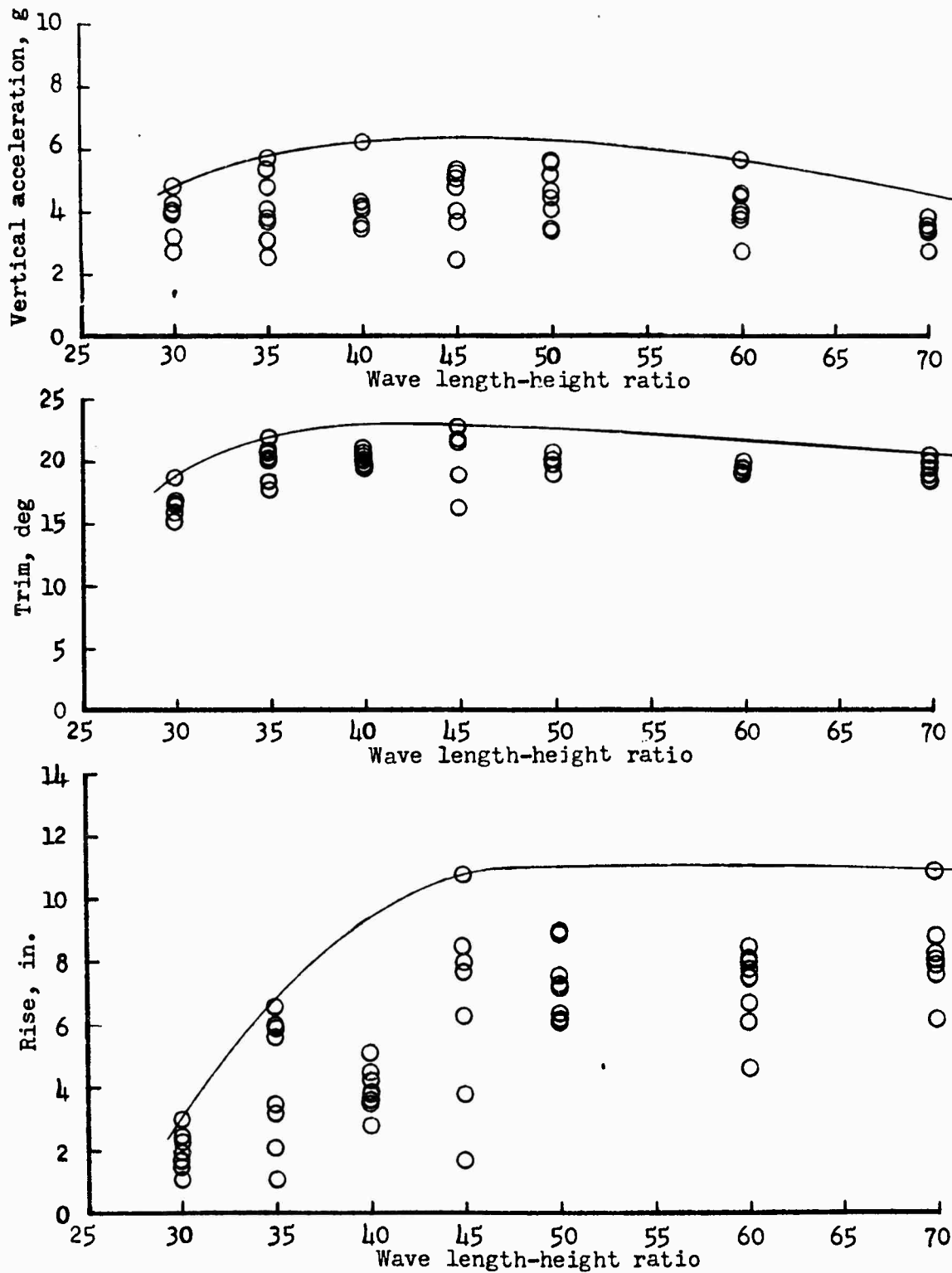
(b) Translating ski.
