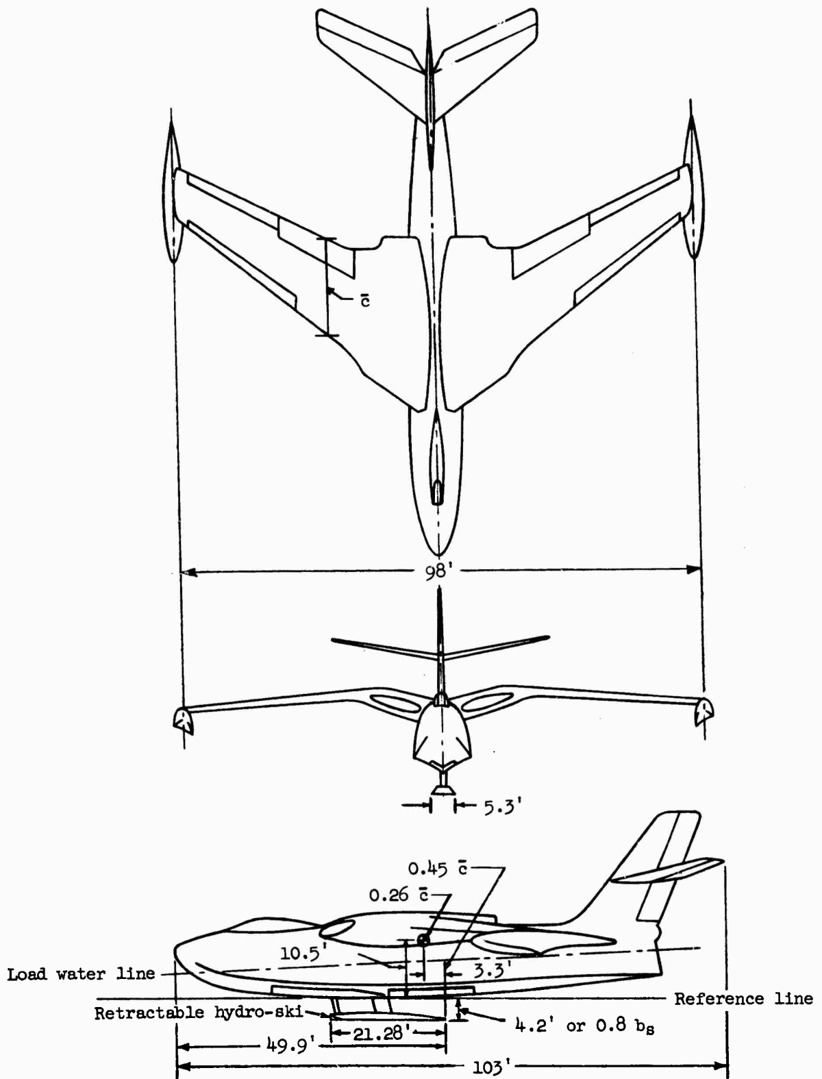
Figure 1.- General arrangement of full-scale seaplane design.
