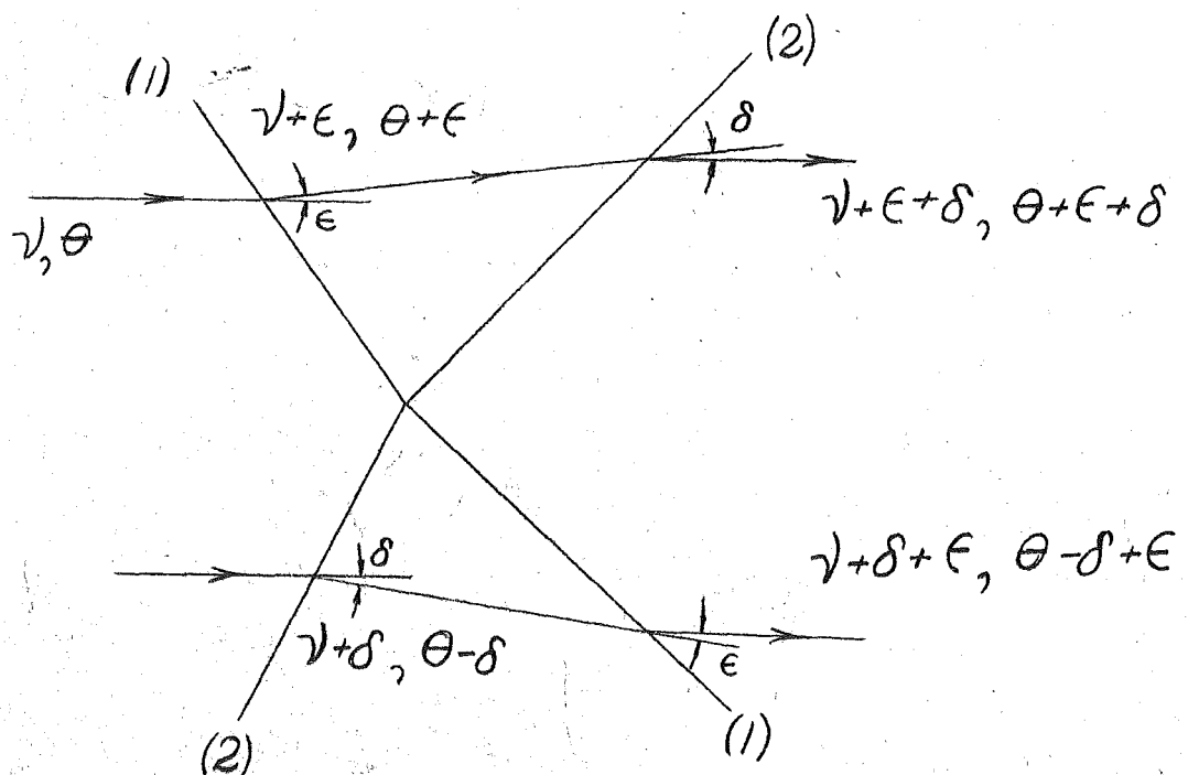
Fig. 5 Intersection of two expansion waves Unclassified
