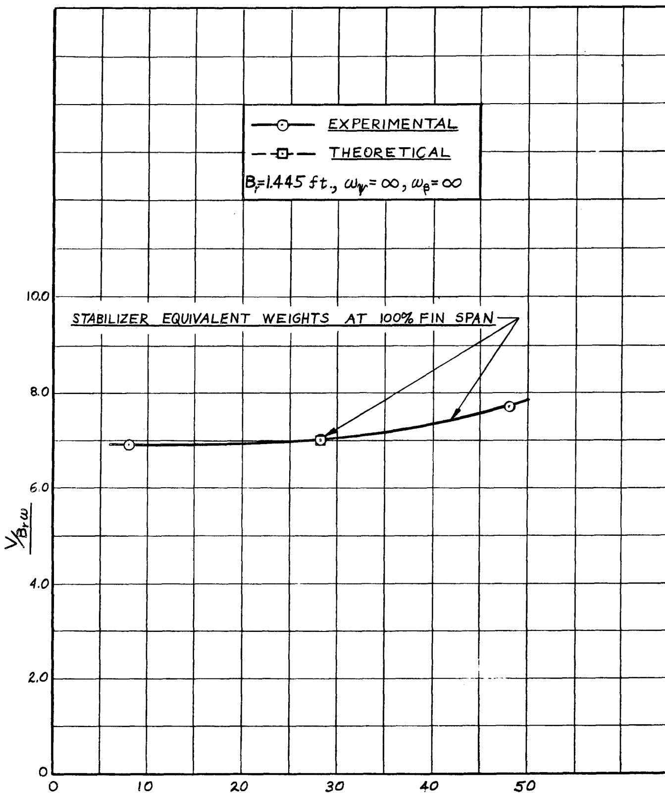
Fig. 7 Effect of Stabilizer Equivalent Weight C.G. Location on Critical V/B_r \omega , Fuselage Locked
