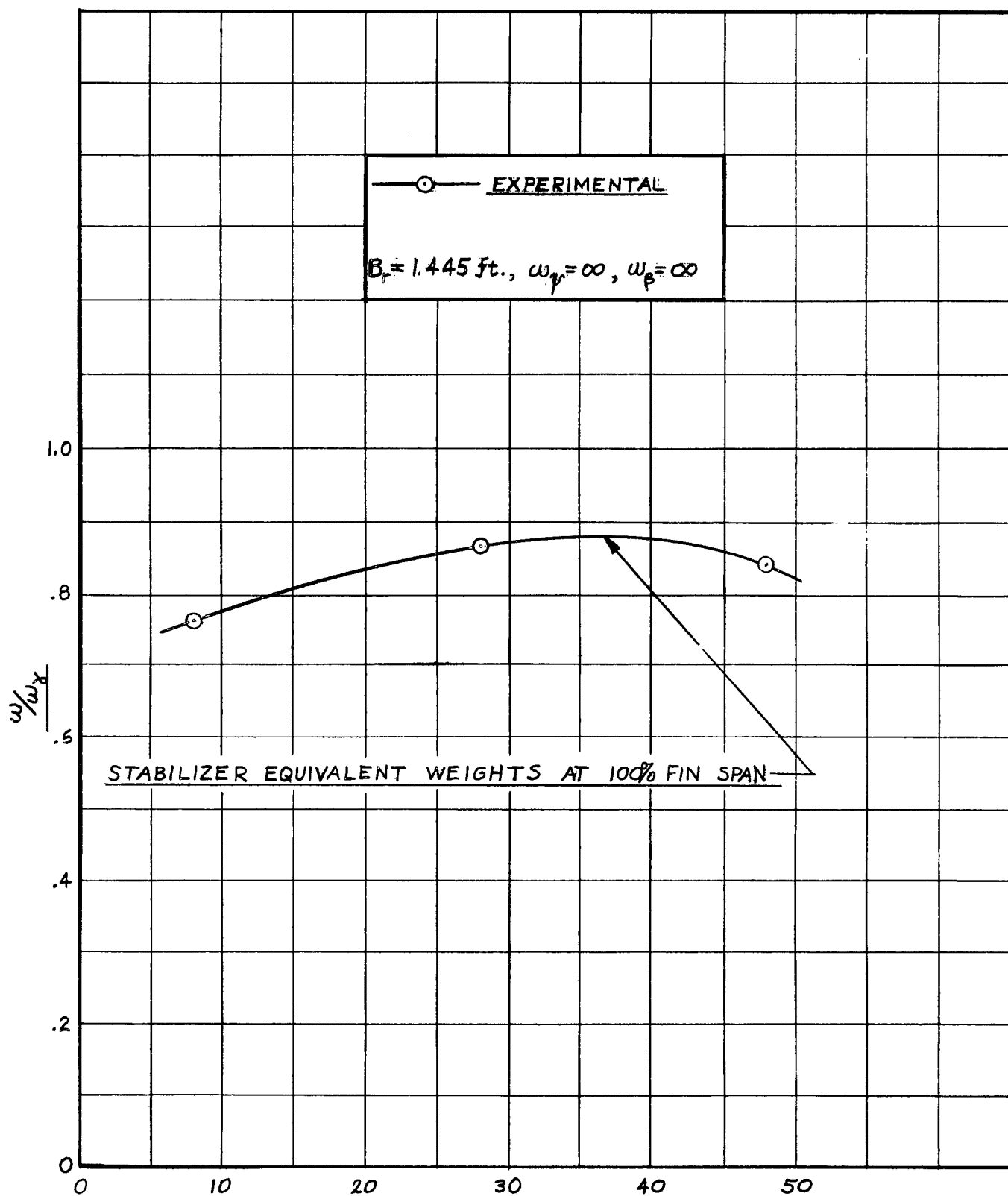
Fig. 12 Effect of Stabilizer Equivalent Weight C.G. Location on Critical \omega/\omega_{cr} , Fuselage Free
