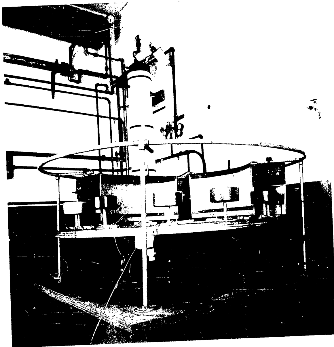
FIG. 5 ALTERNATE CONDENSATION CORROSION TESTER
