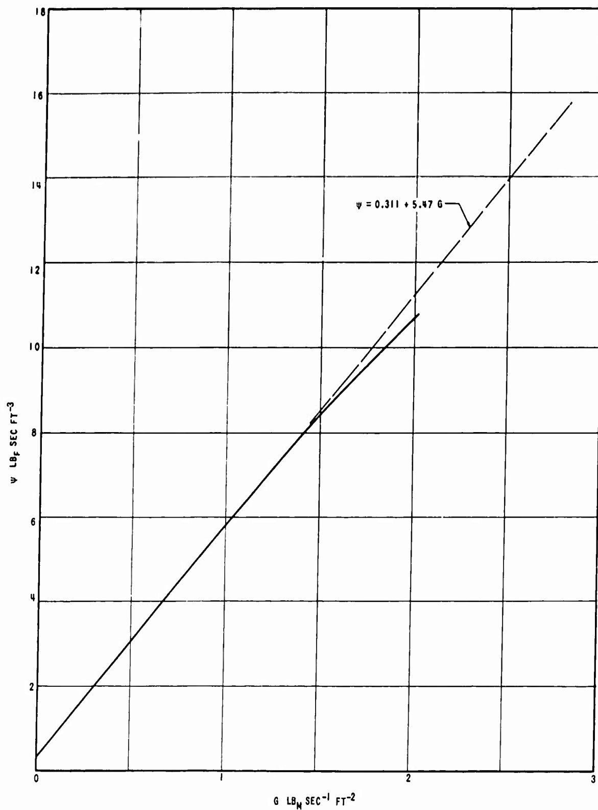
Figure 10. \psi versus Mass Velocity for Fabric BR-40
