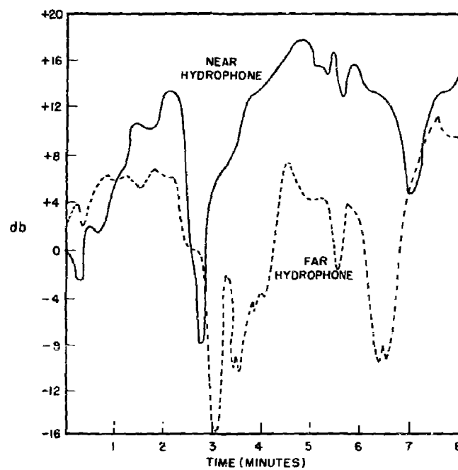
Fig. 18 - Transmission variability during an 8-minute period at a frequency of 126.3 cps to hydrophones located approximately 100 to 200 feet from the source (NOL data, from Ref. 14)
