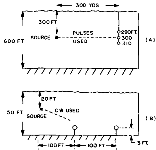
Fig. 16 - Sketches showing the transmission experiments performed by the Applied Physics Laboratory of the University of Washington (A) and by the Naval Ordnance Laboratory (B)
