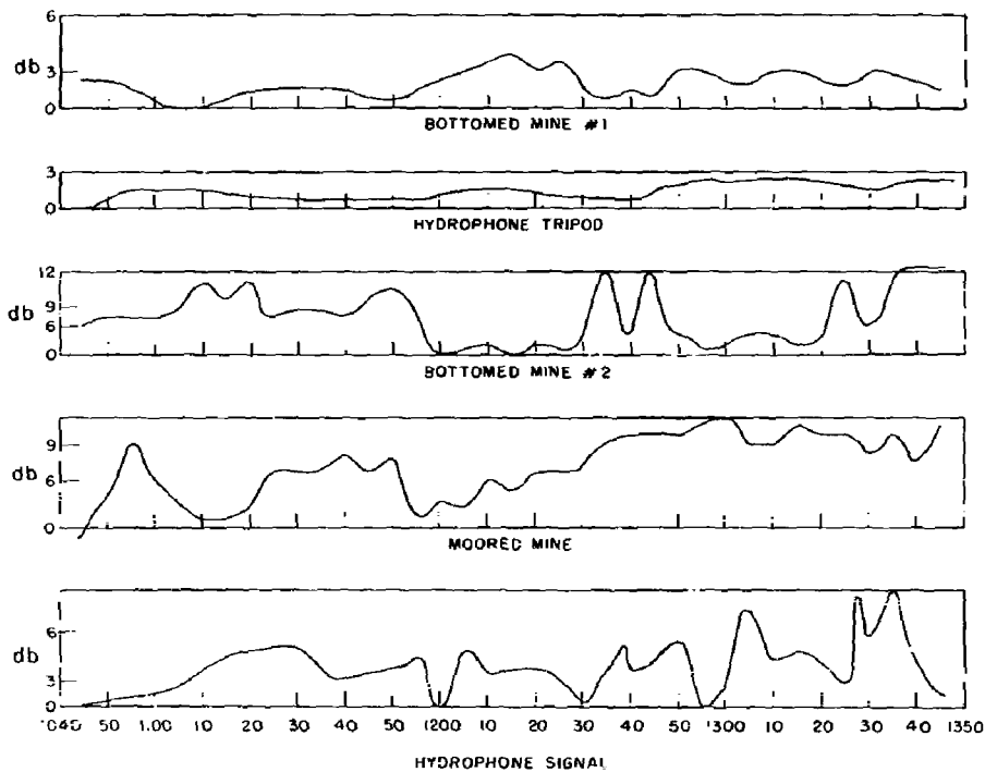
Fig. 13 - Eye-smoothed levels during a 3-hour period of the same events as in Fig. 12
