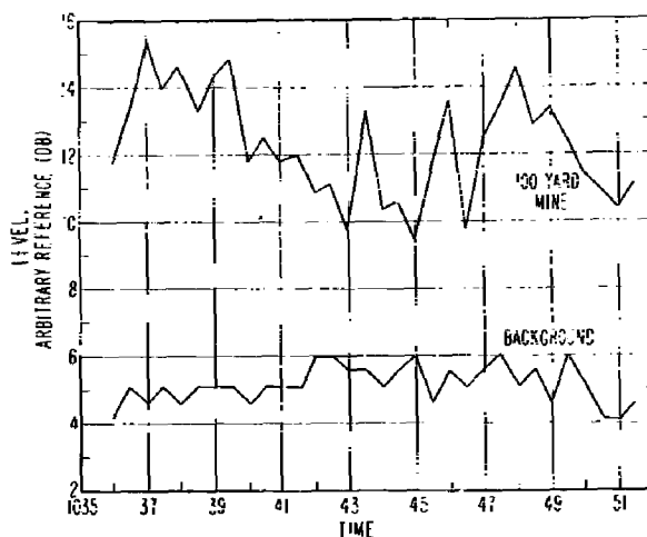
Fig. 10 - Echo variability during a 15-minute period of target at 100 yards
