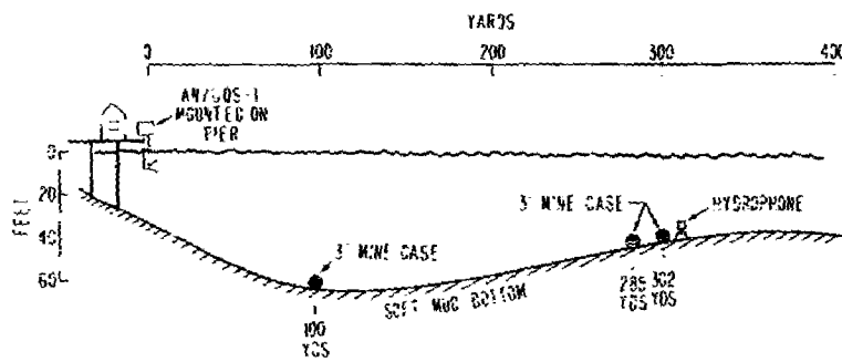
Fig. 4 - Schematic cross section of experimental setup at Solomons, Md.
