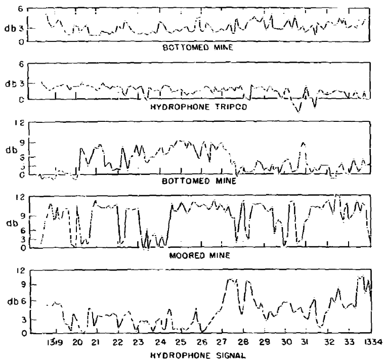
Fig. 12 - Echo levels from the two 300-yard mines, a moored mine, the hydrophone tripod, and the one-way signal level to the hydrophone. Data read from oscilloscope photographs taken at 10-second intervals.
