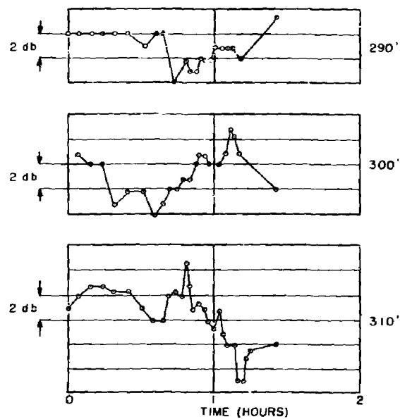
Fig. 17 - Transmission variability during a 1\frac{1}{2} -hour period to three hydrophones 300 yards distant from a deep sound source (APL data, copied from Ref. 13)
