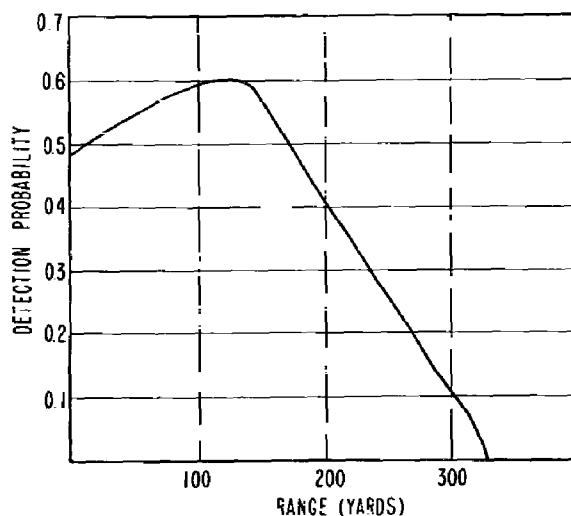
Fig. 1 - Probability of detection of bot-tomed mines versus lateral range during a single passage of an AN/UQS-1-equipped ship travelling at speeds from 1 to 10 knots (USNMCS, Panama City, plot copied from Ref. 2)
