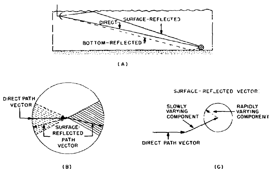
Fig. 14 - (a) Direct, surface-reflected, and bottom-reflected paths. (b,c) Vector phase relationships of the surface reflection.
