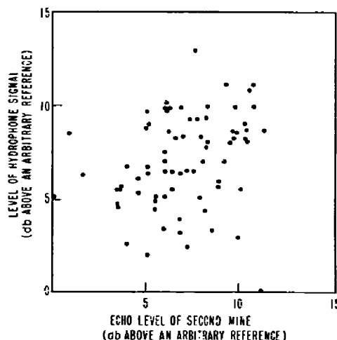
Fig. 9 - Relation between the one-way transmission to a bottomed hydrophone and the echo level from a nearby bottomed target
