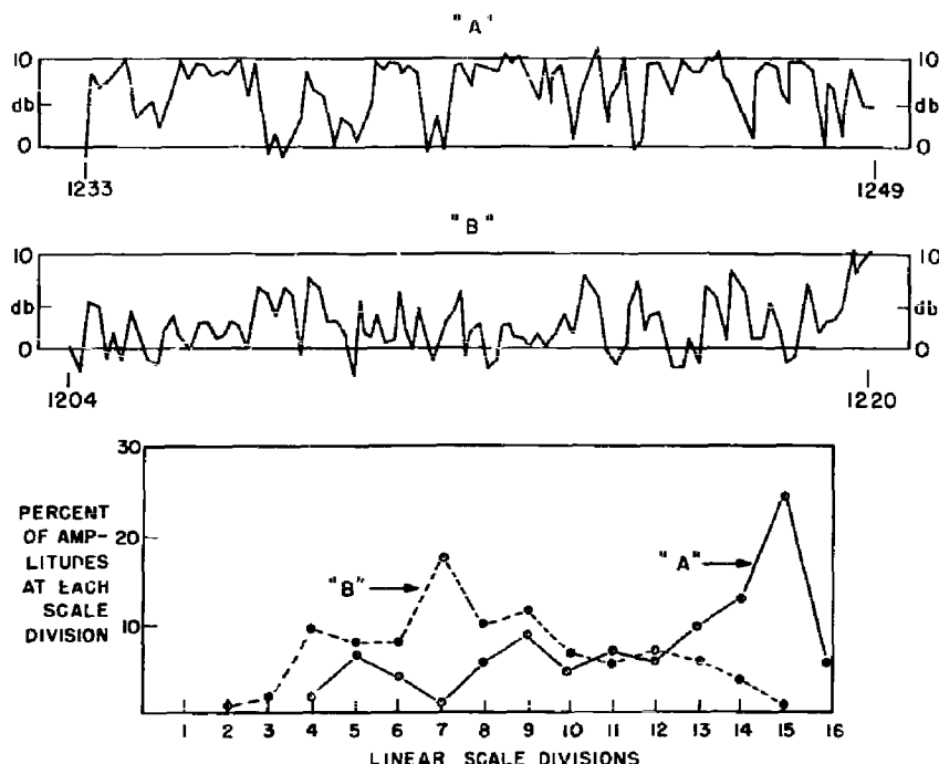
Fig. 15 - The distribution of amplitude of the echo from one of the bottomed mines during a period of good transmission "A" and during a fade "B"
