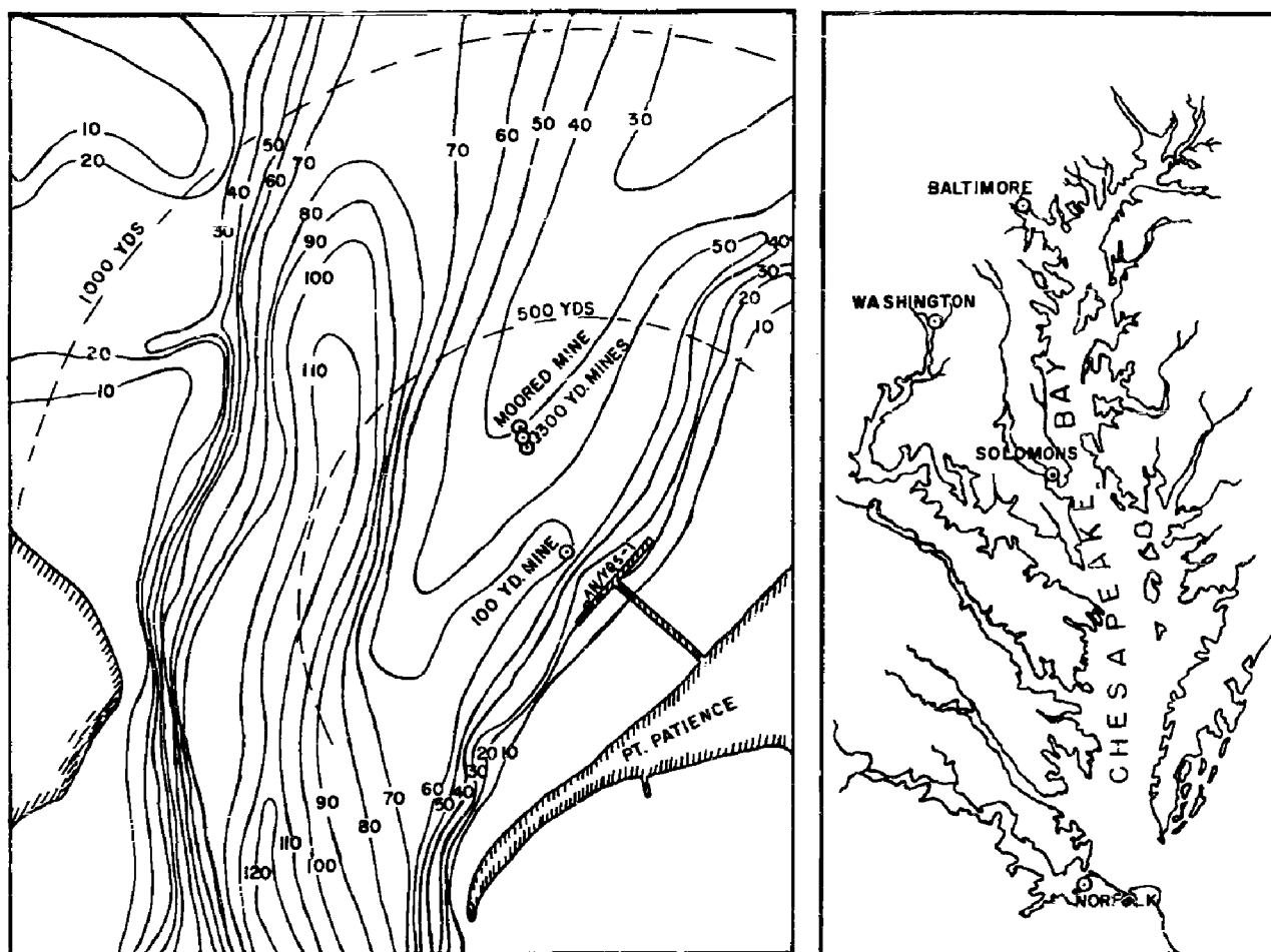
Fig. 2 - Bathymetric chart of test area at Solomons, Md., and location chart of Chesapeake Bay
