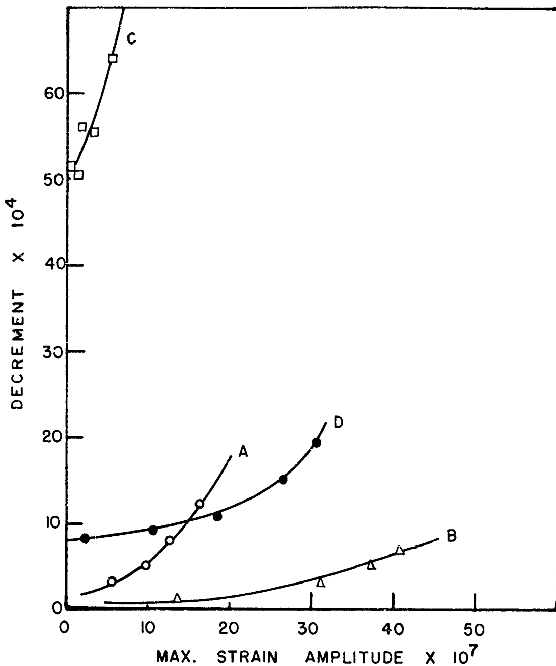
FIG. 19 EFFECT OF ANNEALING AT 25^{\circ} C ON INTERNAL FRICTION
