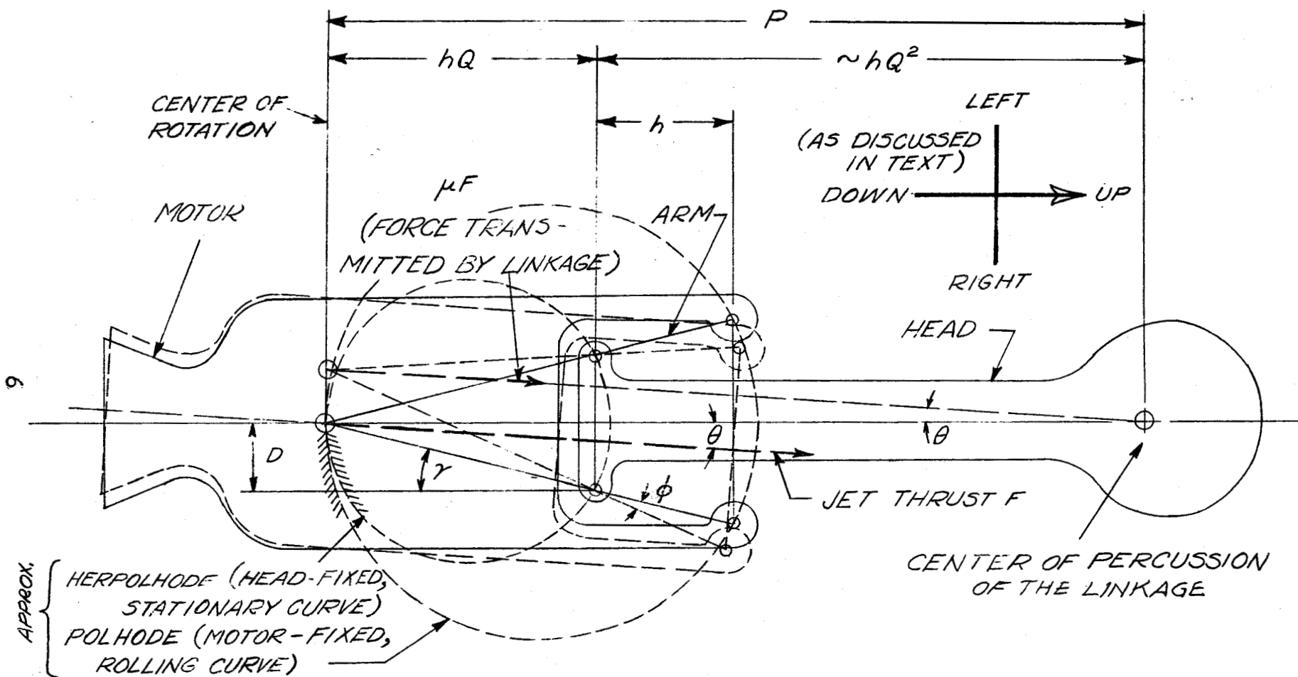
FIG. 1 - TRAPEZOIDAL LINKAGE
