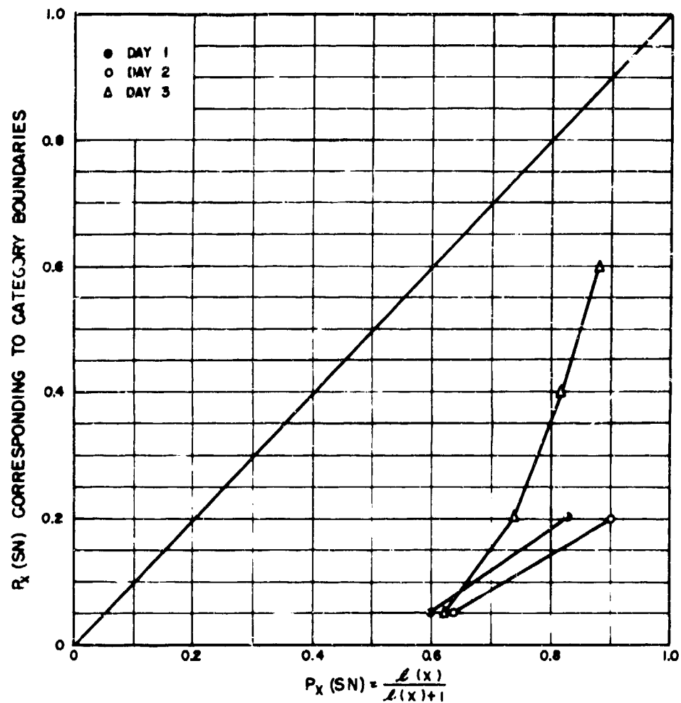
FIG 14. OBJECTIVE PROBABILITY VS. SUBJECTIVE PROBABILITY FOR OBSERVER 4.
