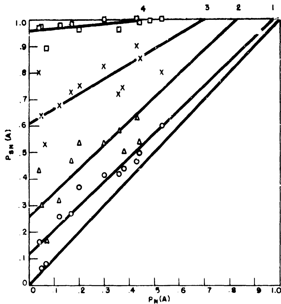
FIG. 2. P_{SN}(A) VS. P_N(A) FOR OBSERVER 1 IN THE FIRST EXPECTED-VALUE EXPERIMENT.
