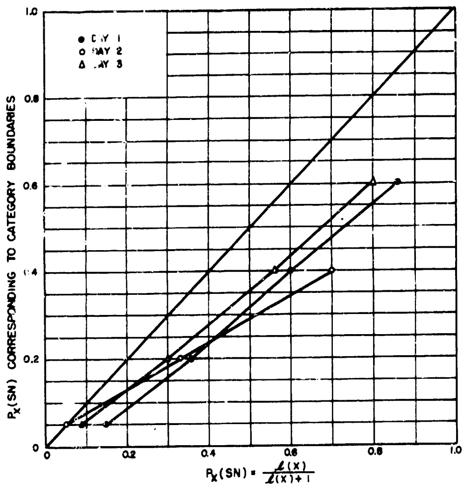
FIG. 12. OBJECTIVE PROBABILITY VS. SUBJECTIVE PROBABILITY FOR OBSERVER 2.
