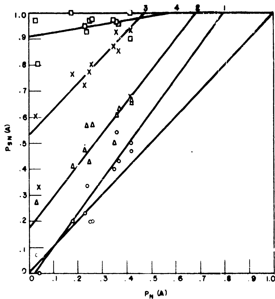
FIG. 3. P_{SN}(A) VS P_N(A) FOR OBSERVER 2 IN THE FIRST EXPECTED-VALUE EXPERIMENT.
