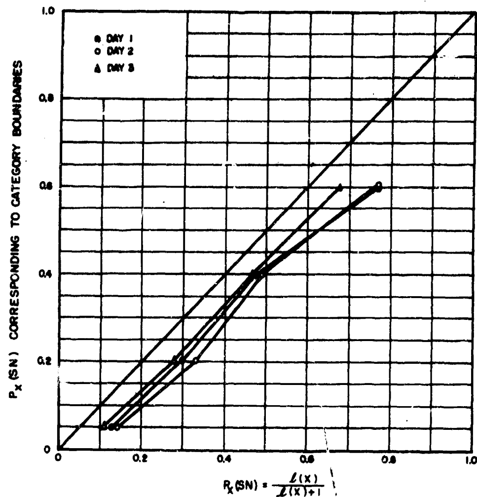
FIG. II. OBJECTIVE PROBABILITY VS. SUBJECTIVE PROBABILITY FOR OBSERVER 1.
