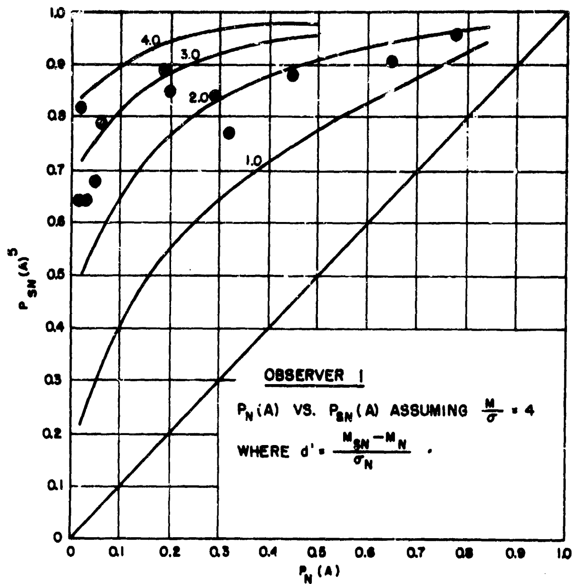
FIG. 7. P_{SN}(A) VS. P_N(A) FOR OBSERVER 1 IN THE SECOND EXPECTED-VALUE EXPERIMENT.
