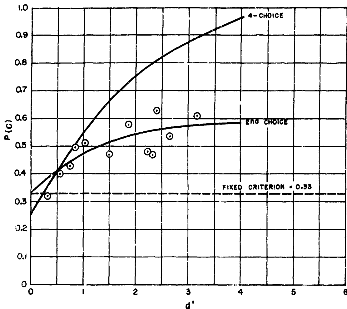
FIG. 16. THE SECOND-CHOICE DATA AND PREDICTIONS FOR THE SECOND-CHOICE SITUATION UNDER THE ASSUMPTION THAT \frac{\Delta M}{\Delta \sigma} = 4 .
