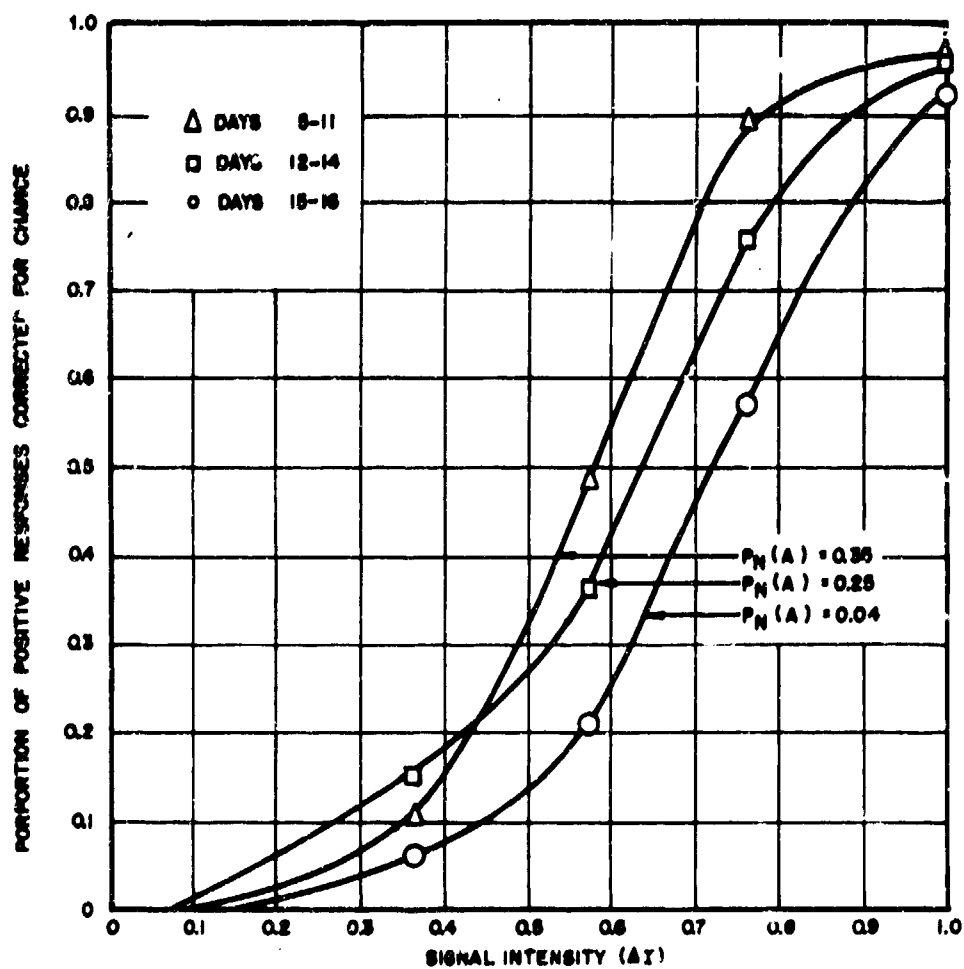
FIG. 6. RAW DATA CORRECTED FOR CHANCE, AVERAGE FOR ALL OBSERVERS IN THE FIRST EXPECTED-VALUE EXPERIMENT.
