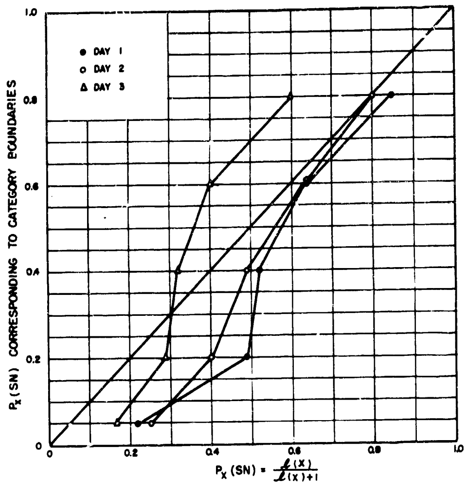
FIG. 13. OBJECTIVE PROBABILITY VS. SUBJECTIVE PROBABILITY FOR OBSERVER 3.
