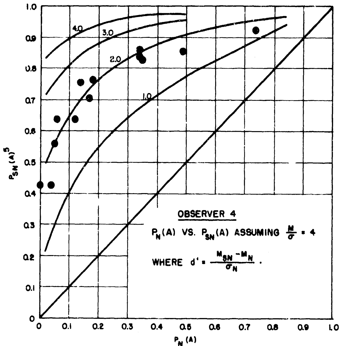
FIG. 10. P_{SN}(A) VS. P_N(A) FOR OBSERVER 4 IN THE SECOND EXPECTED-VALUE EXPERIMENT.
