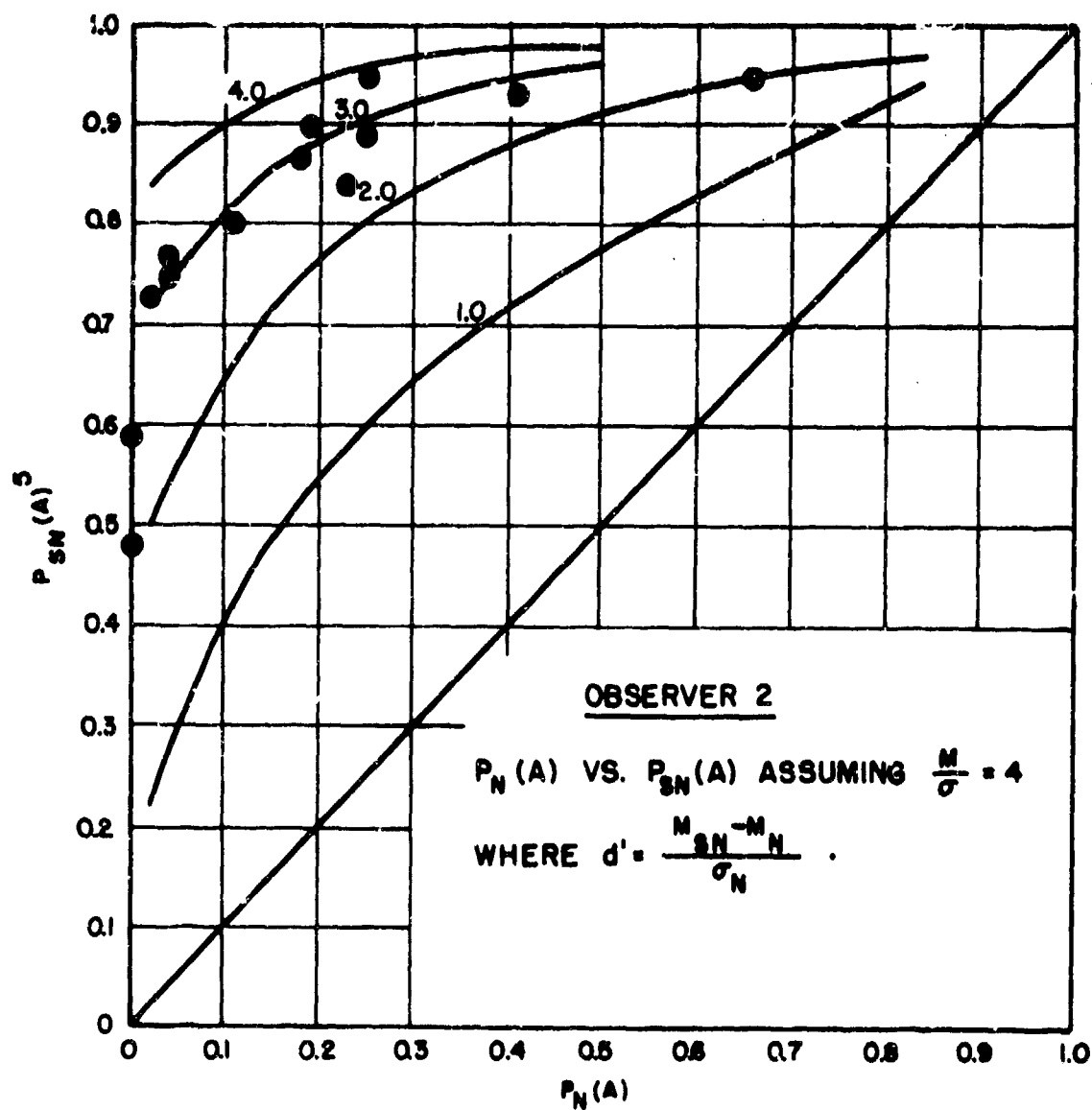
FIG. 8. P_{SN}(A) VS. P_N(A) FOR OBSERVER 2 IN THE SECOND EXPECTED-VALUE EXPERIMENT.
