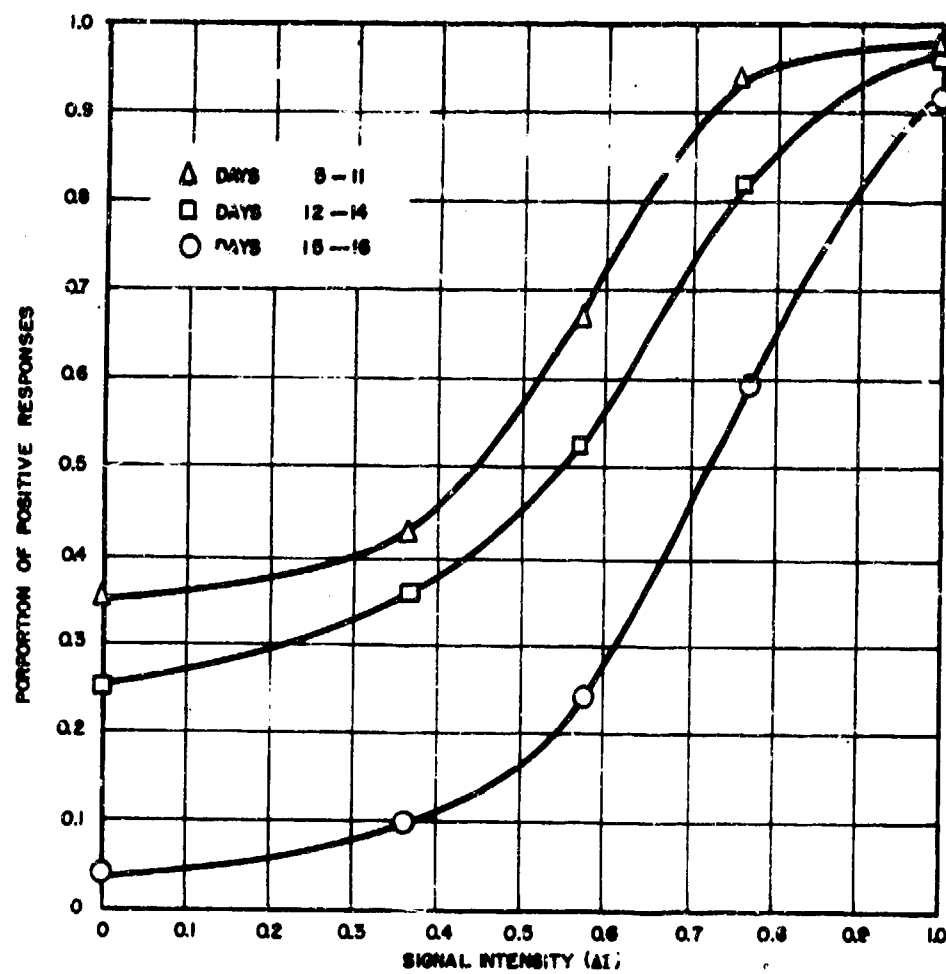
FIG. 5. RAW DATA, AVERAGE FOR ALL OBSERVERS IN THE FIRST EXPECTED-VALUE EXPERIMENT.
