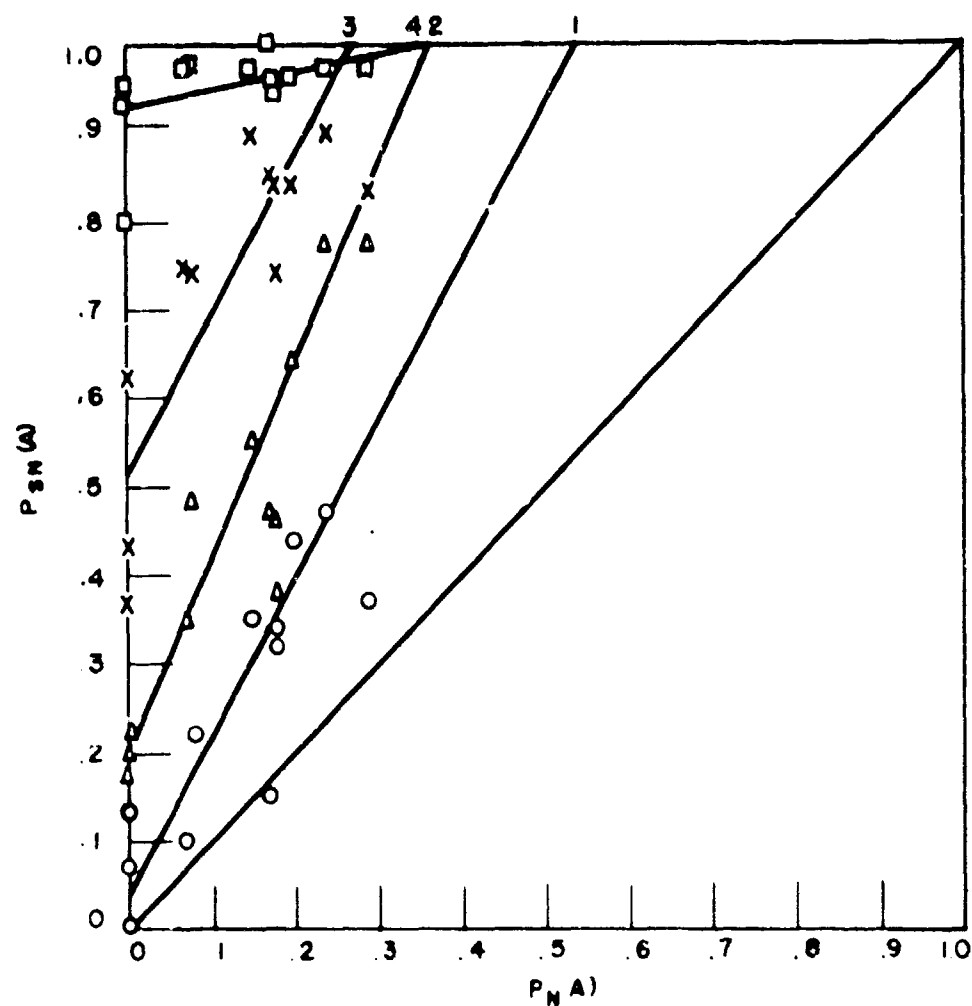
FIG. 4. P_{SN}(A) VS. P_N(A) FOR OBSERVER 3 IN THE FIRST EXPECTED-VALUE EXPERIMENT.
