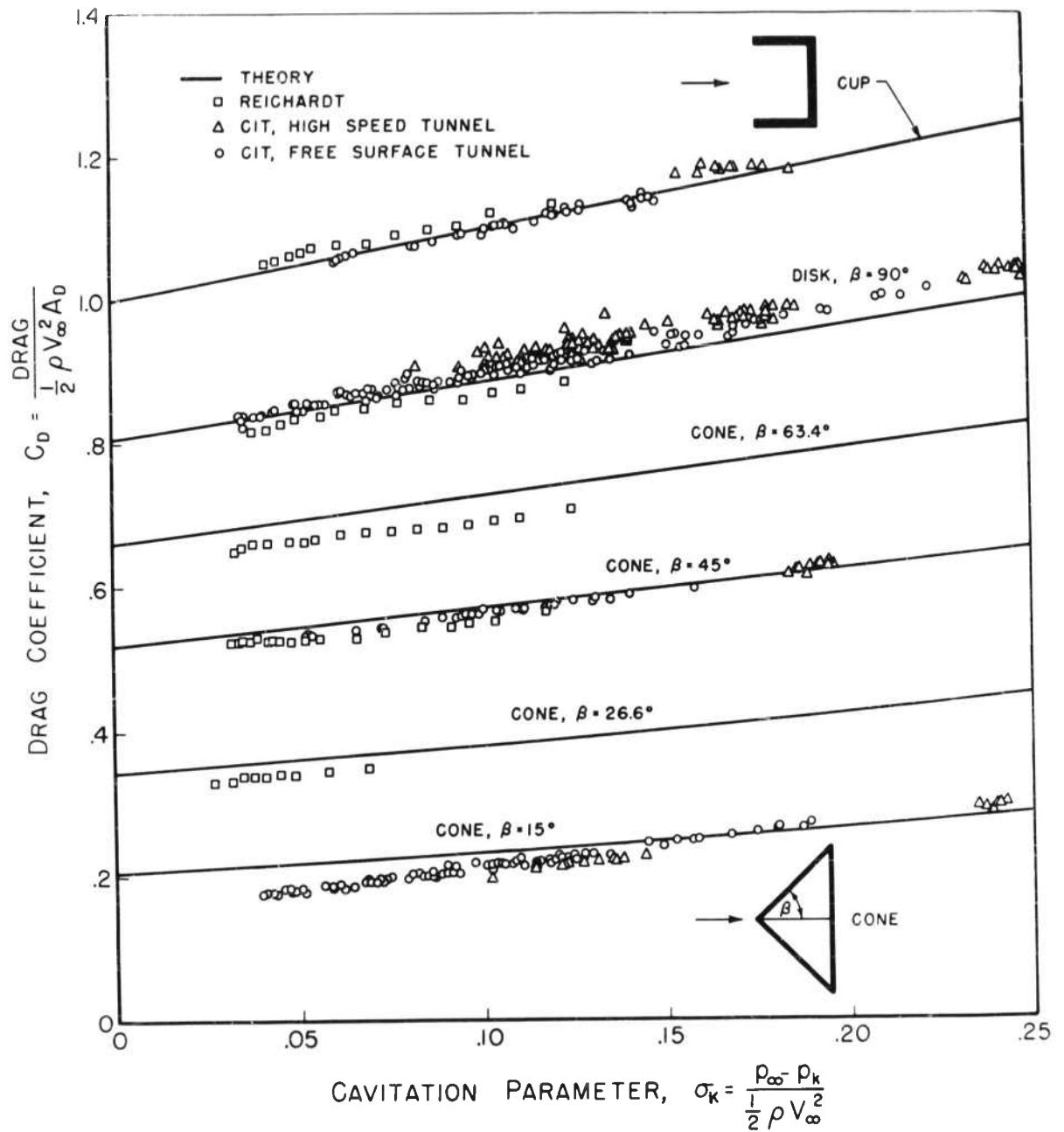
Fig. 2 - Drag coefficient vs. cavity parameter \sigma_k for cups, disks and cones
