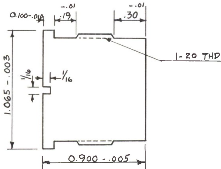
Figure 2. Aluminum Base plugs
