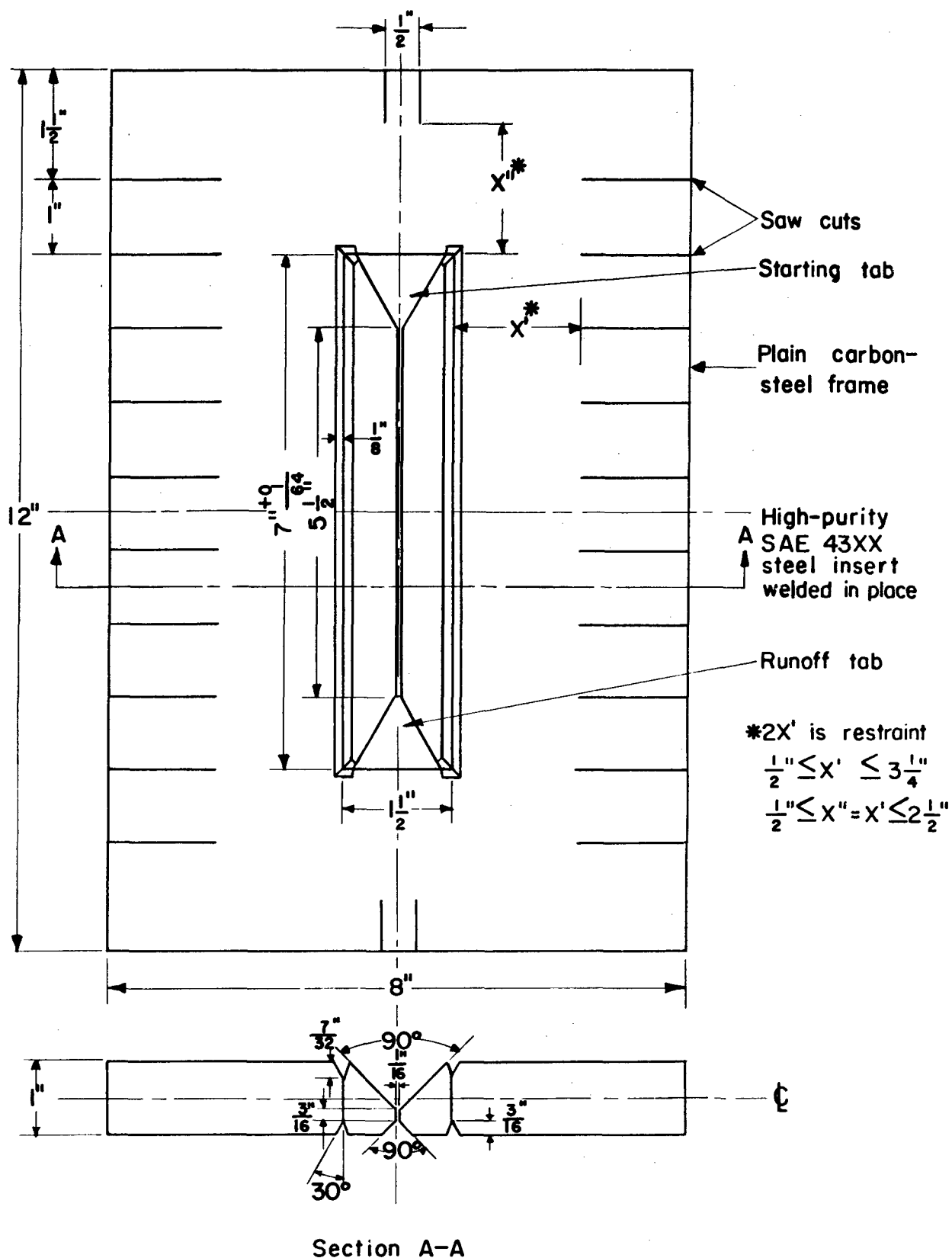
FIGURE 9. RESTRAINED WELD-CRACKING SPECIMEN
