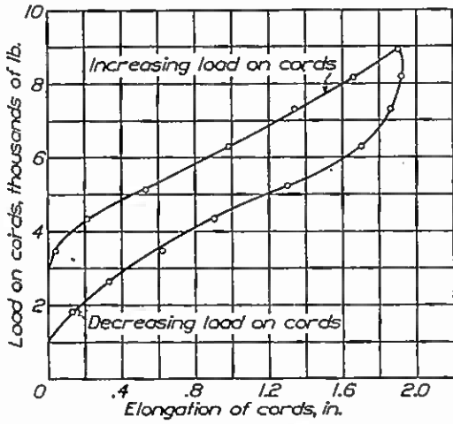
FIGURE 8.—Hysteresis curve of rubber cords on Mercury-type gear. Work done on rubber cords, 12,100 in.-lb.; work returned by rubber cords, 8,460 in.-lb.; work absorbed by rubber cords, 3,640 in.-lb. or 30.1 per cent
