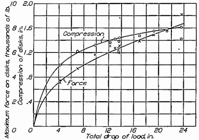
FIGURE 14.—Compression of rubber disks and forces on them during drop tests
