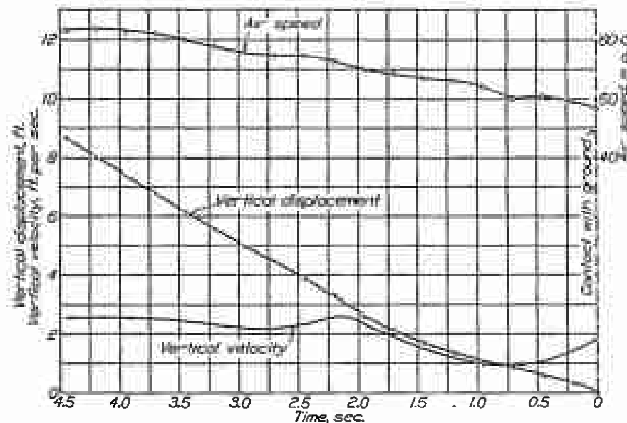
FIGURE 21.—Normal landing
