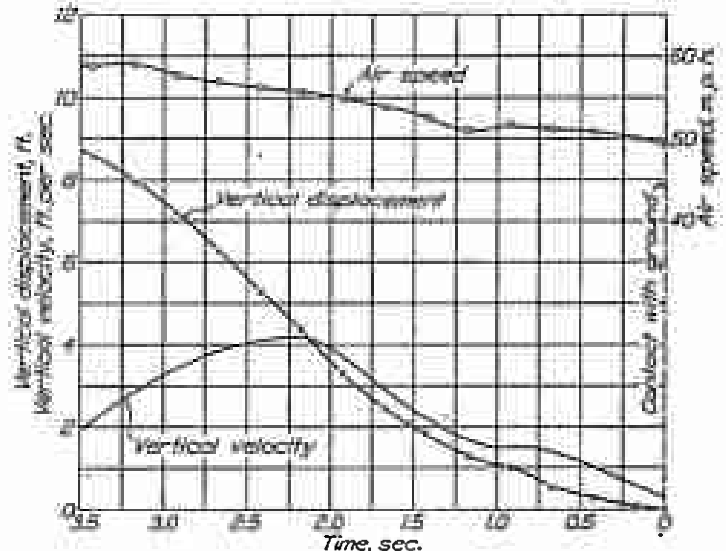
FIGURE 20.—Normal landing
