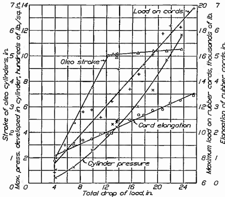
FIGURE 13.—Strokes of oleo cylinder, maximum pressure in cylinder, elongation of rubber cards, and load on rubber cards during drop tests
