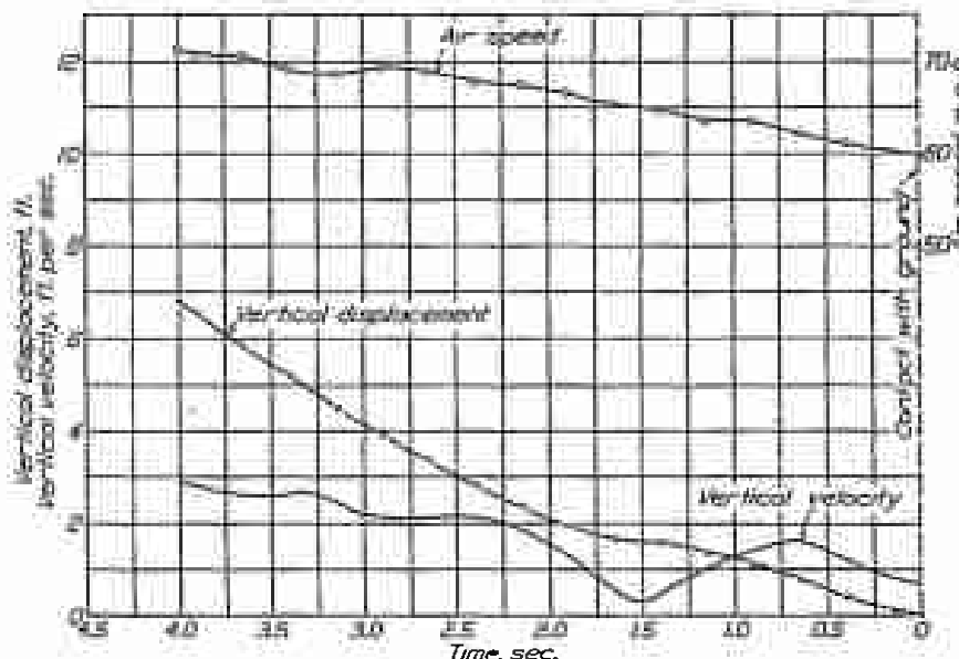
FIGURE 22.—Two-point landing
