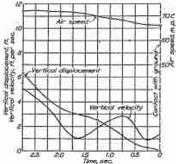
FIGURE 23.—Two-point landing
