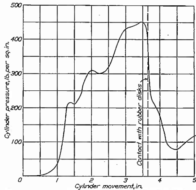
FIGURE 18.—Variation of cylinder pressure with cylinder displacement for an NY-8 oleo gear. Free drop of 1 inch. Oil level 5 3/8 inches from top of piston with full load on gear.
