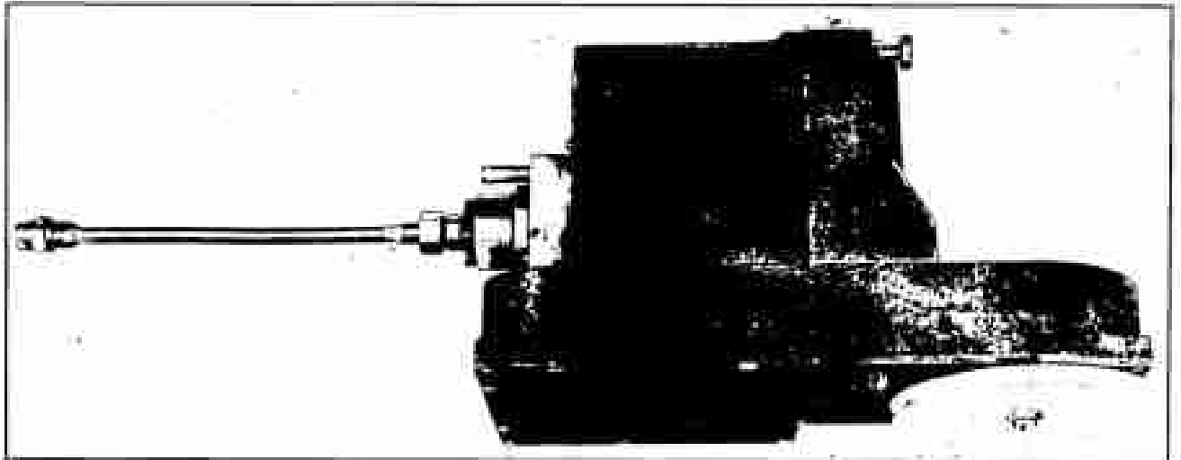
FIGURE 6.—Pressure-displacement recorder
