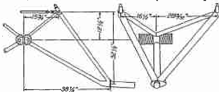
FIGURE 3.—Mercury (rubber-cord type) landing-gear chassis
