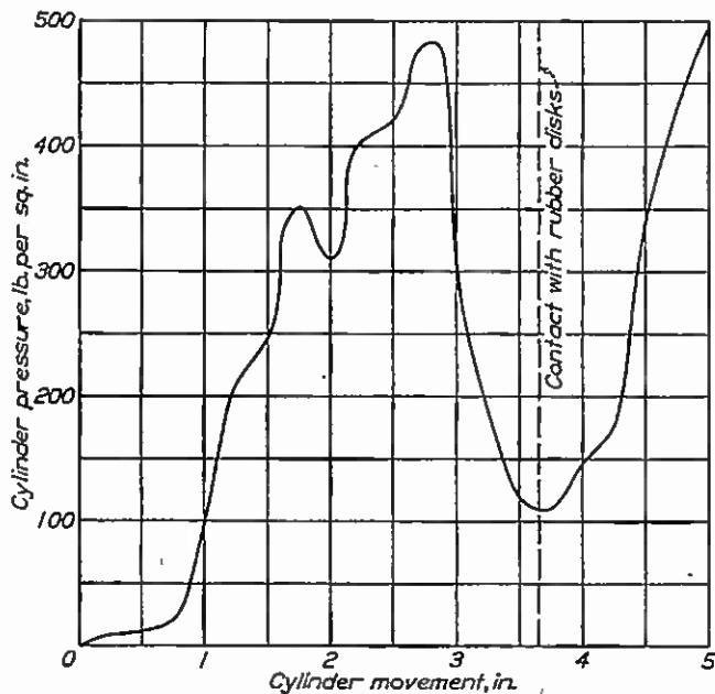
FIGURE 17.—Variation of cylinder pressure with cylinder displacement for an NY-3 oleo gear. Free drop of 1 inch. Oil level 4 3/8 inches from top of piston with full load on gear.
