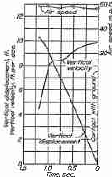
FIGURE 24.—Pancake landing
