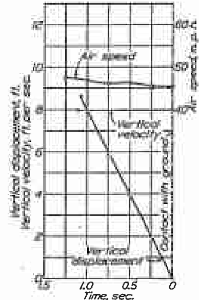
FIGURE 25.—Pancake landing
