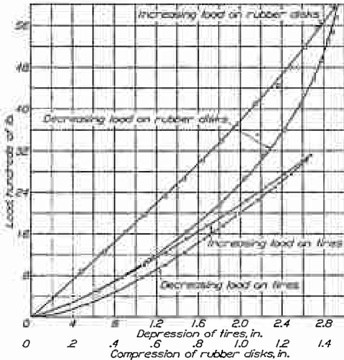
FIGURE 9.—Hysteresis curves of tires and rubber disks on NY-9 oleo gear. Work done on disks, 4,040 in.-lb.; work returned by disks, 2,840 in.-lb.; work absorbed by disks, 1,200 in.-lb. or 30.1 per cent. Work done on tires, 1,830 in.-lb.; work returned by tire, 1,625 in.-lb.; work absorbed by tire, 205 in.-lb. or 11.2 per cent
