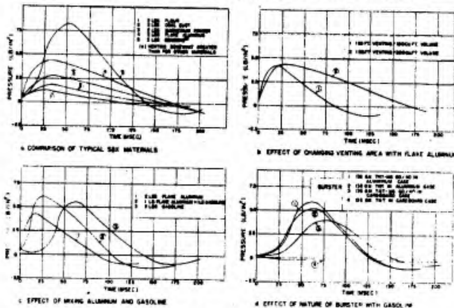
FIG. 9. PRESSURE VERSUS TIME CURVES FOR SBX UNDER VARIOUS CONDITIONS MORROW
