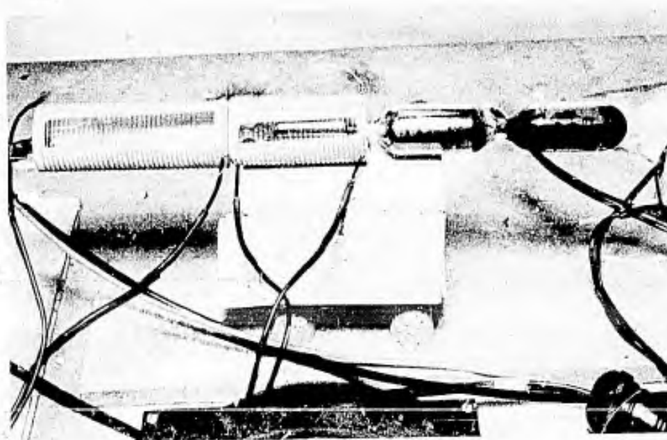
FIG. 5 APPARATUS FOR PREPARATION OF HIGH PURITY SELENIUM
