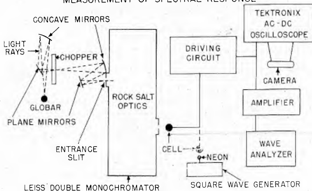
FIG. II MEASUREMENT OF SPECTRAL RESPONSE
