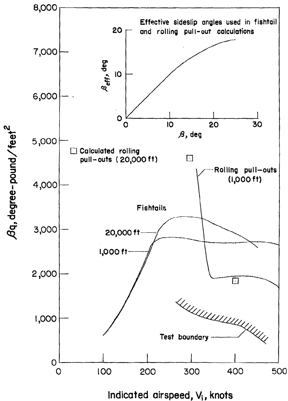
Figure 20.- Comparison of test results for the F-86A airplane with maximum calculated values of vertical-tail load parameter \beta q during fishtail and rolling pull-out maneuvers.
