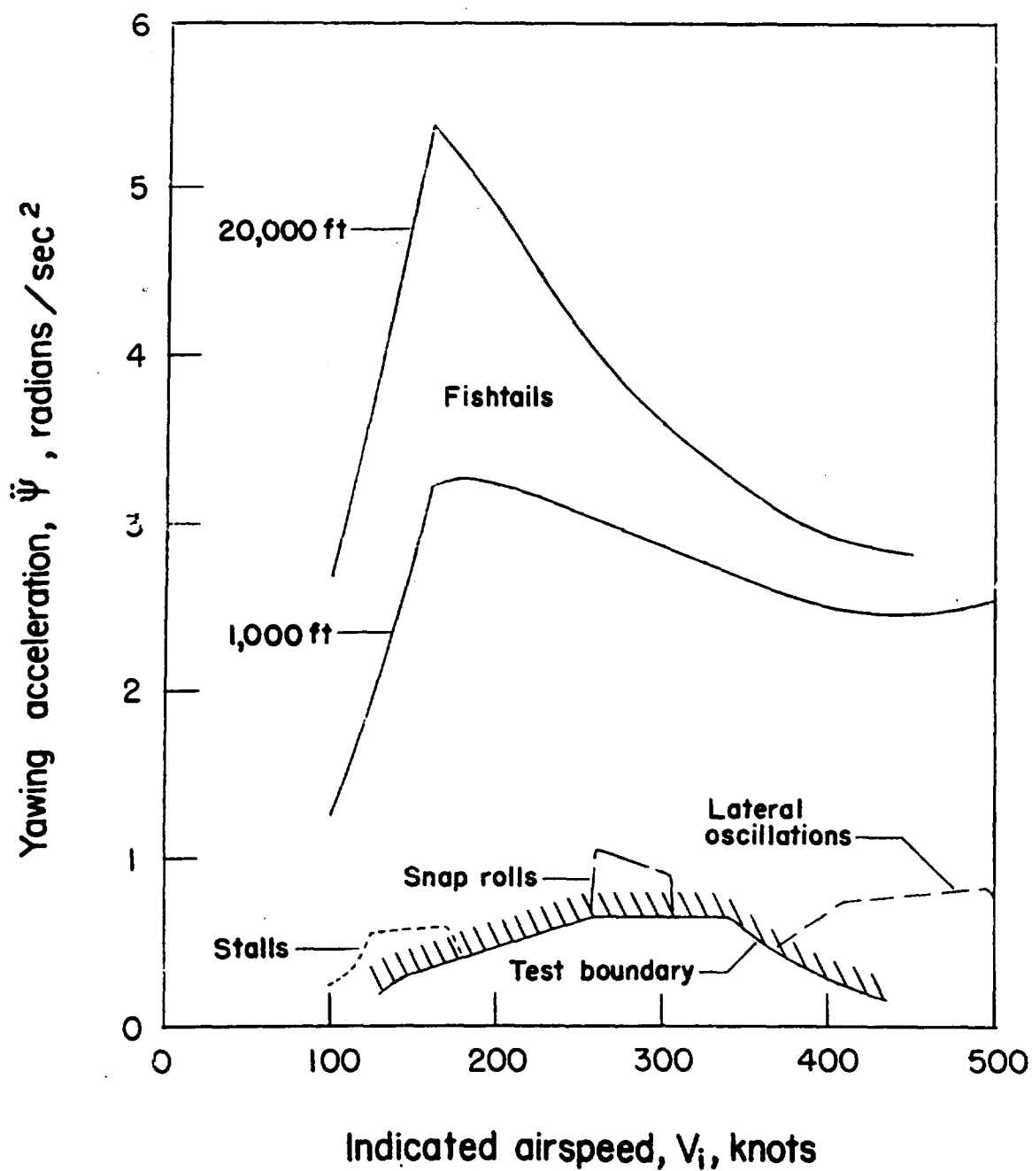
Figure 27.- Comparison of test results for the F-84 airplane with maximum calculated values of yawing acceleration during fishtail maneuvers.
