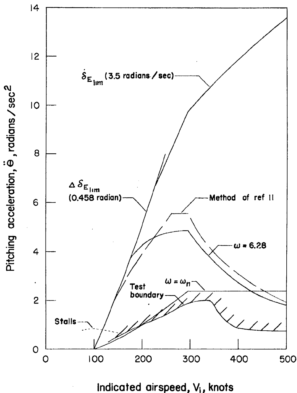
Figure 10.- Comparison of test results with maximum calculated pitching accelerations obtained by maneuvering the F-86A airplane sinusoidally between a load factor of 1 and the upper limit of the design V-n diagram at sea level.
