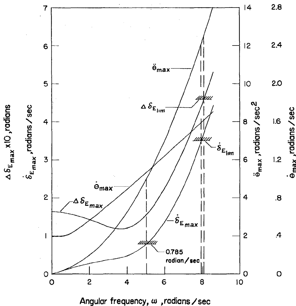
Figure 7.- Maximum control and response values calculated for the F-86A airplane maneuvering sinusoidally between the upper and lower limits of the design V-n diagram for an airspeed of 300 knots at sea level.
