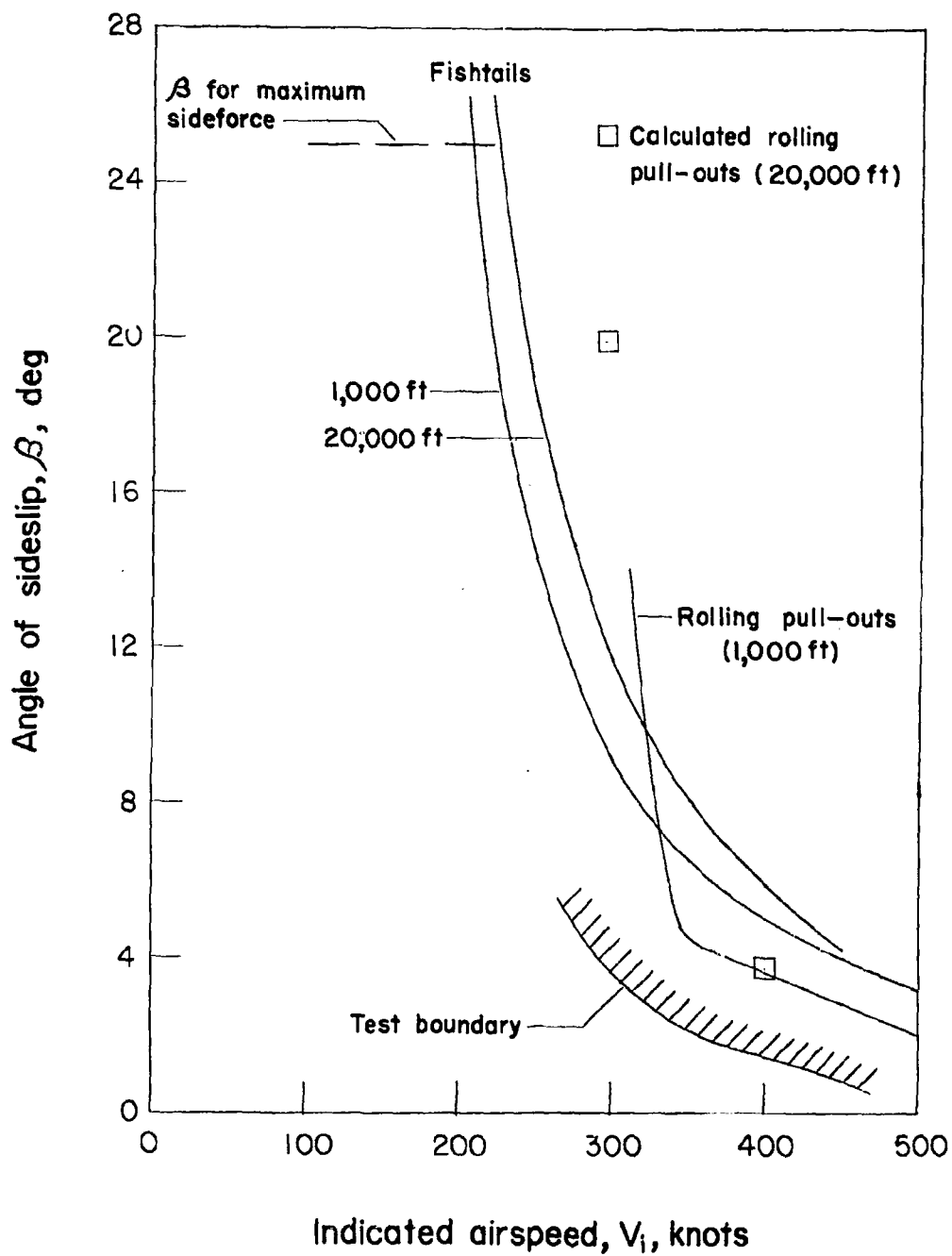
Figure 18.- Comparison of test results for the F-86A airplane with maximum calculated values of sideslip during fishtail and rolling pull-out maneuvers.
