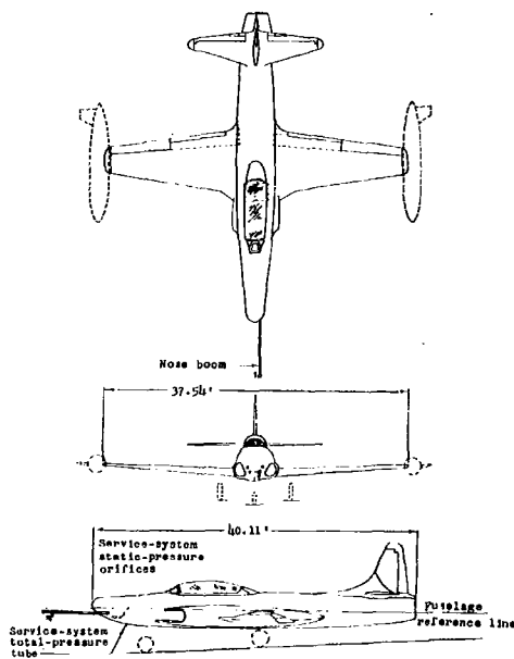
F-94B
