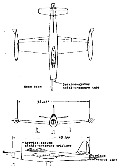
F-84G
