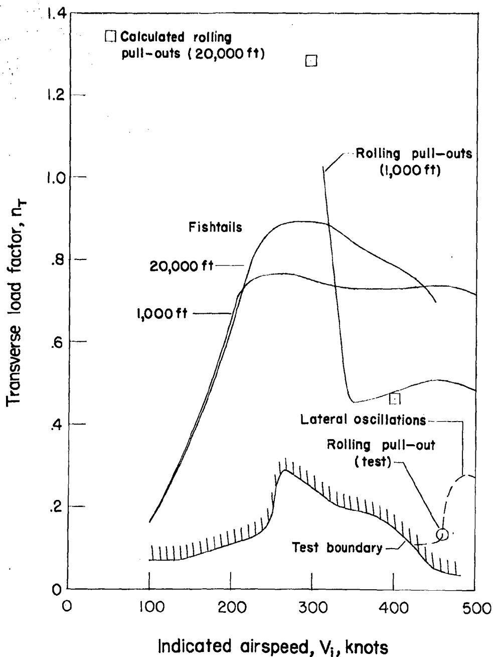
Figure 22.- Comparison of test results for the F-86A airplane with maximum calculated values of transverse load factor during fish-tail and rolling pull-out maneuvers.
