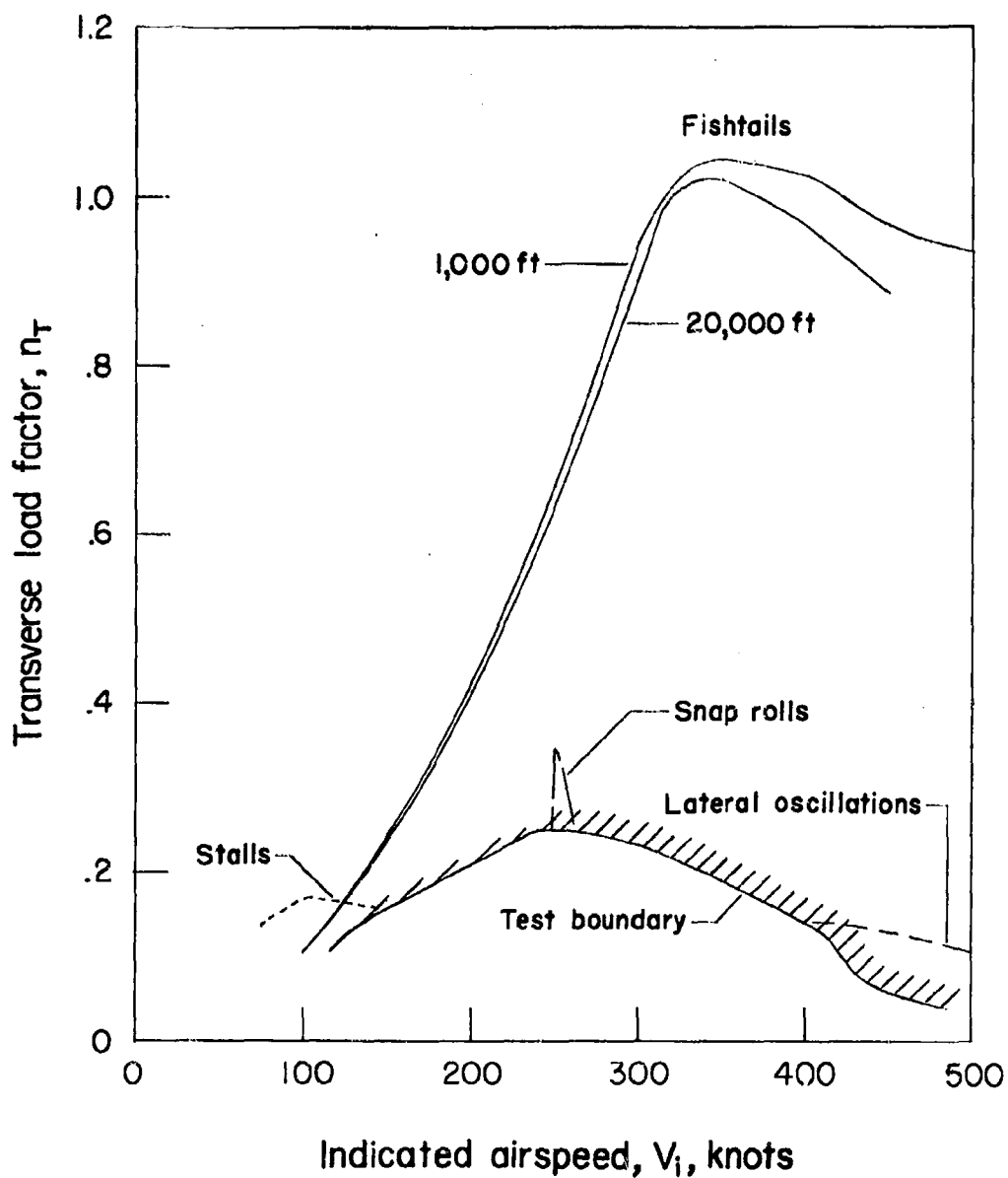
Figure 23.- Comparison of test results for the F-84 airplane with maximum calculated values of transverse load factor during fish-tail maneuvers.
