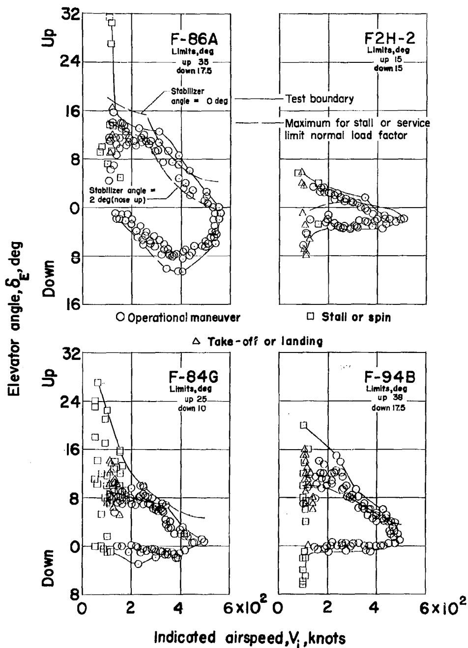
Figure 3.- Comparison of test results with maximum elevator angles needed to reach stall or the service limit normal load factor in gradual maneuvers.
