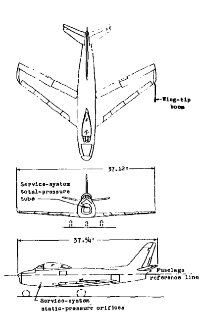
F-86A
