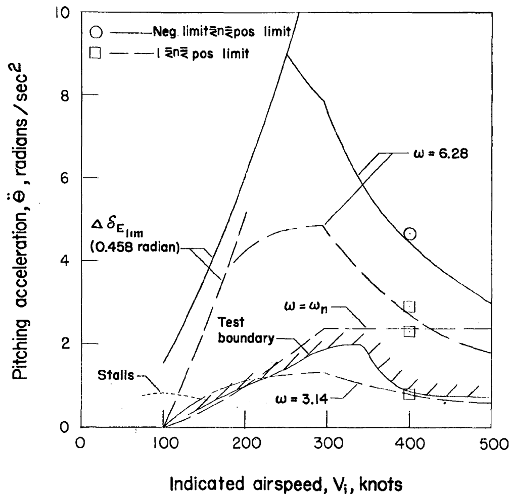
Figure 9.- Comparison of test results with maximum calculated pitching accelerations obtained by maneuvering the F-86A airplane sinusoidally within the V-n diagram at sea level. (Symbols are for altitude of 20,000 feet.)
