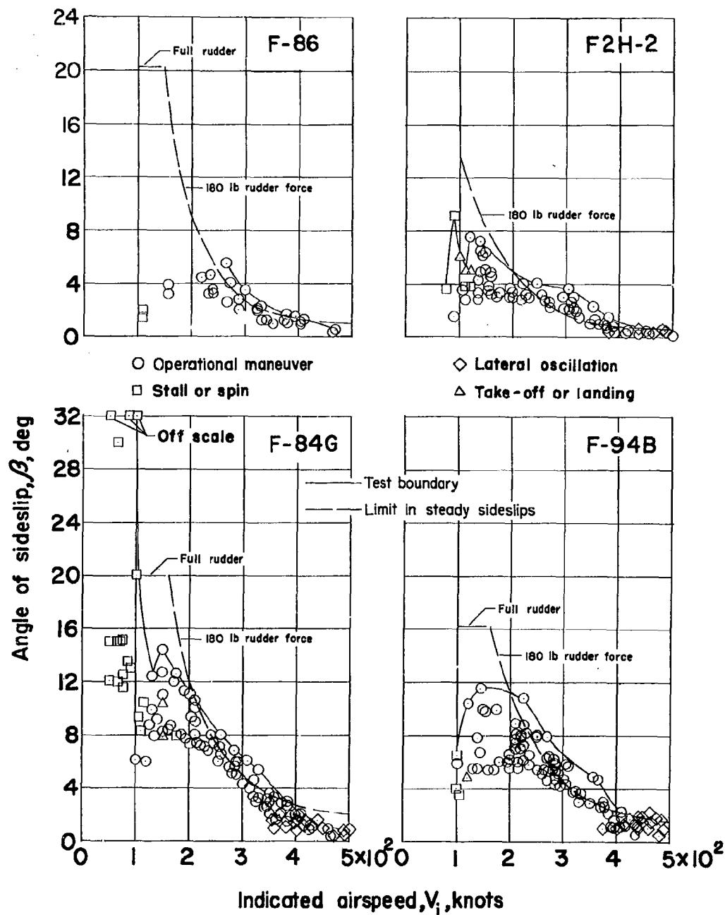
Figure 17.- Comparison of test results with maximum angles of sideslip obtainable in steady sideslips using maximum rudder control force of 180 pounds.
