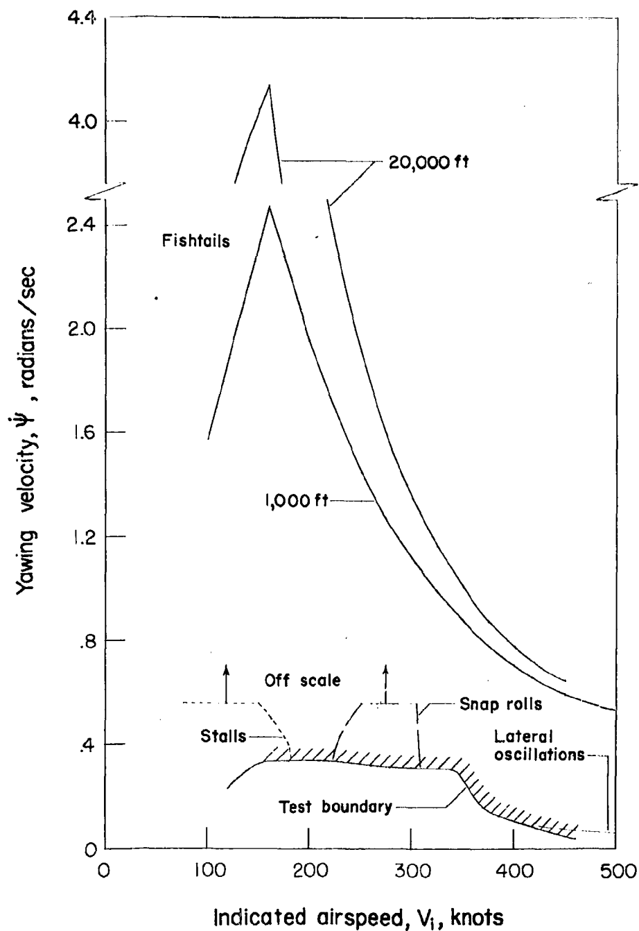
Figure 25.- Comparison of test results for the F-84 airplane with maximum calculated values of yawing velocity during fishtail maneuvers.
