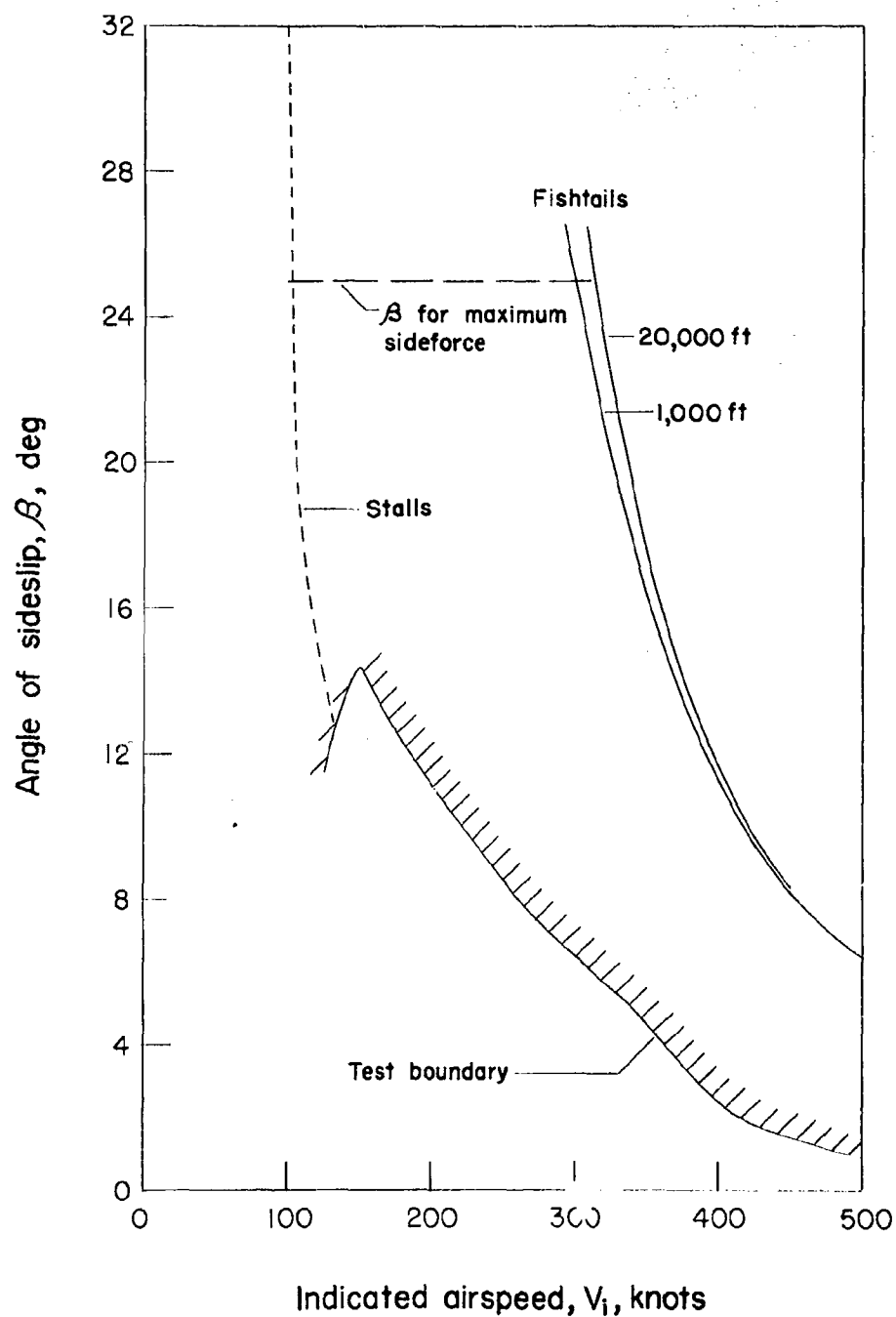
Figure 19.- Comparison of test results for the F-84 airplane with maximum calculated values of sideslip during fishtail maneuvers.
