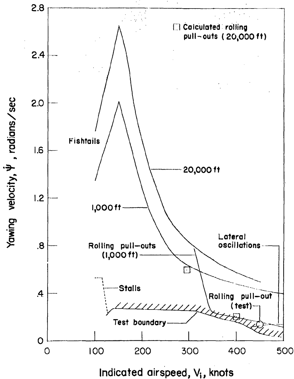
Figure 24.- Comparison of test results for the F-86A airplane with maximum calculated values of yawing velocity during fishtail and rolling pull-out maneuvers.
