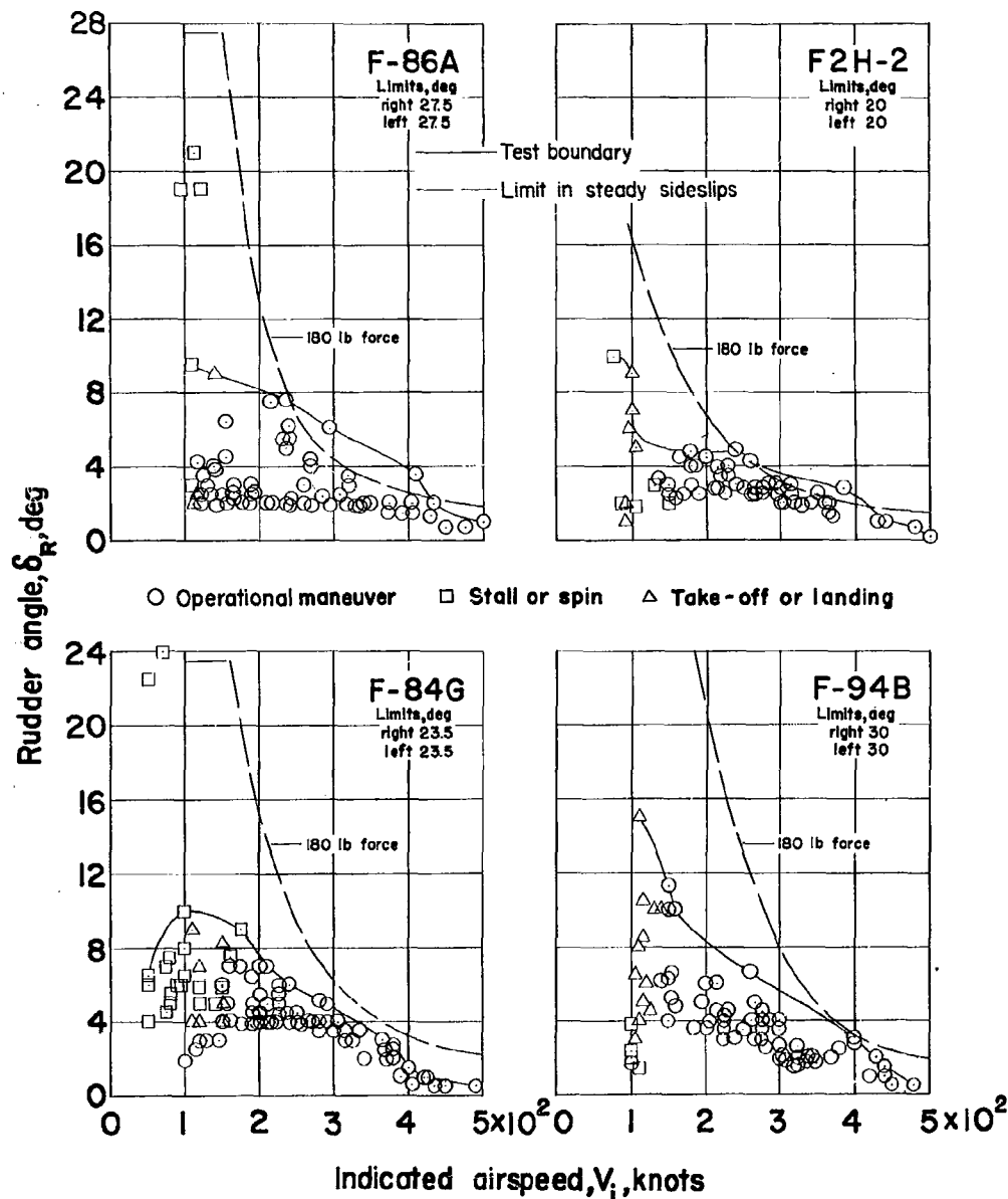
Figure 16.- Comparison of test results with maximum rudder angles obtainable in steady sideslips using maximum control force of 180 pounds.
