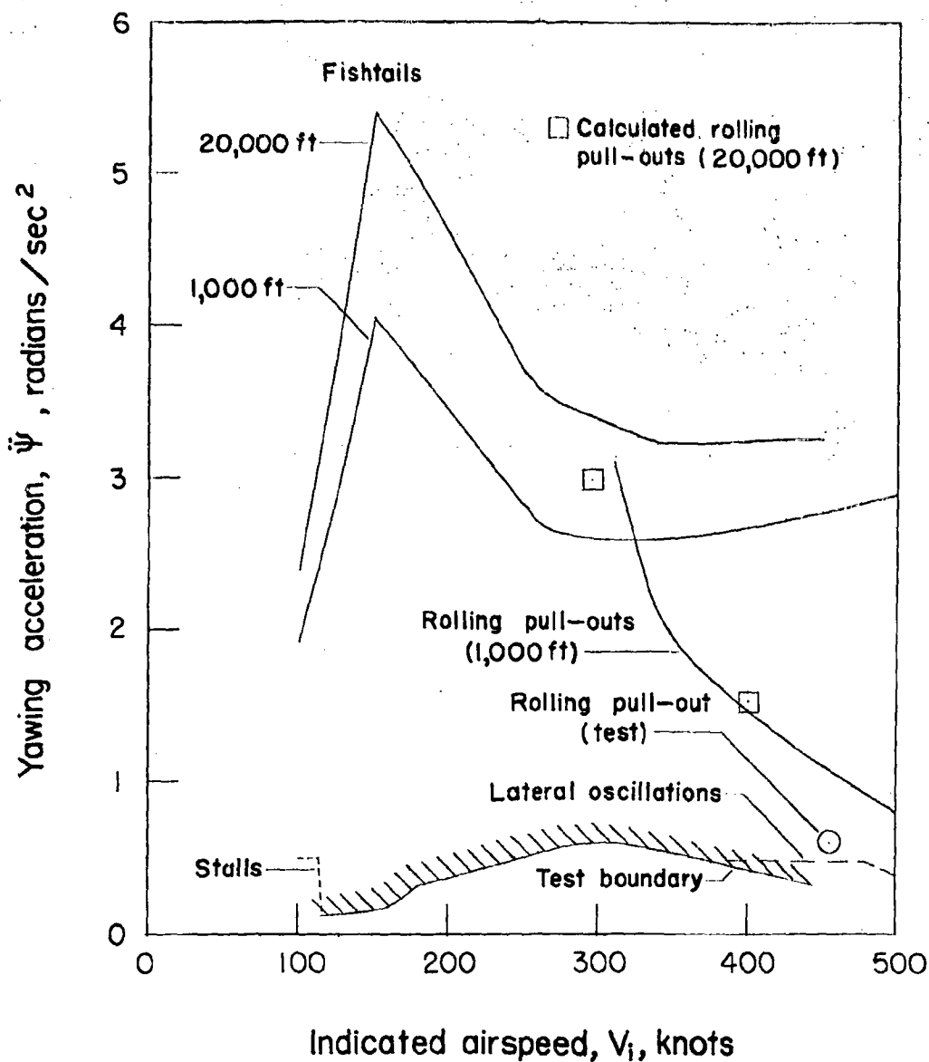
Figure 26.- Comparison of test results for the F-86A airplane with maximum calculated values of yawing acceleration during fishtail and rolling pull-out maneuvers.
