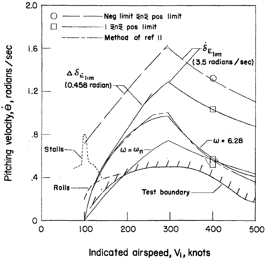
Figure 11.- Comparison of test results with maximum calculated pitching velocities obtained by maneuvering the F-86A airplane sinusoidally within the V-n diagram at sea level. (Symbols at 400 knots are for altitude of 20,000 feet.)
