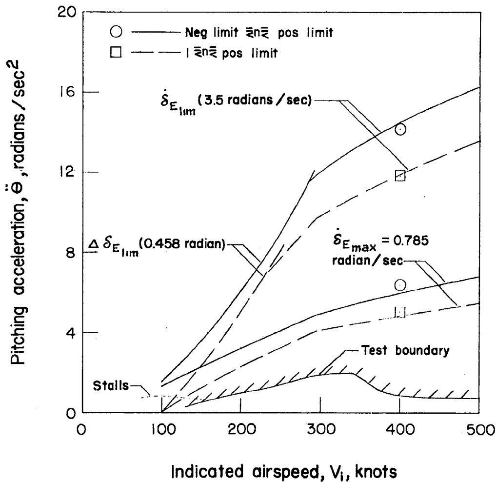
Figure 8.- Comparison of test results with maximum calculated pitching accelerations obtained by maneuvering the F-86A airplane sinusoidally within the V-n diagram at sea level. (Symbols are for altitude of 20,000 feet.)
