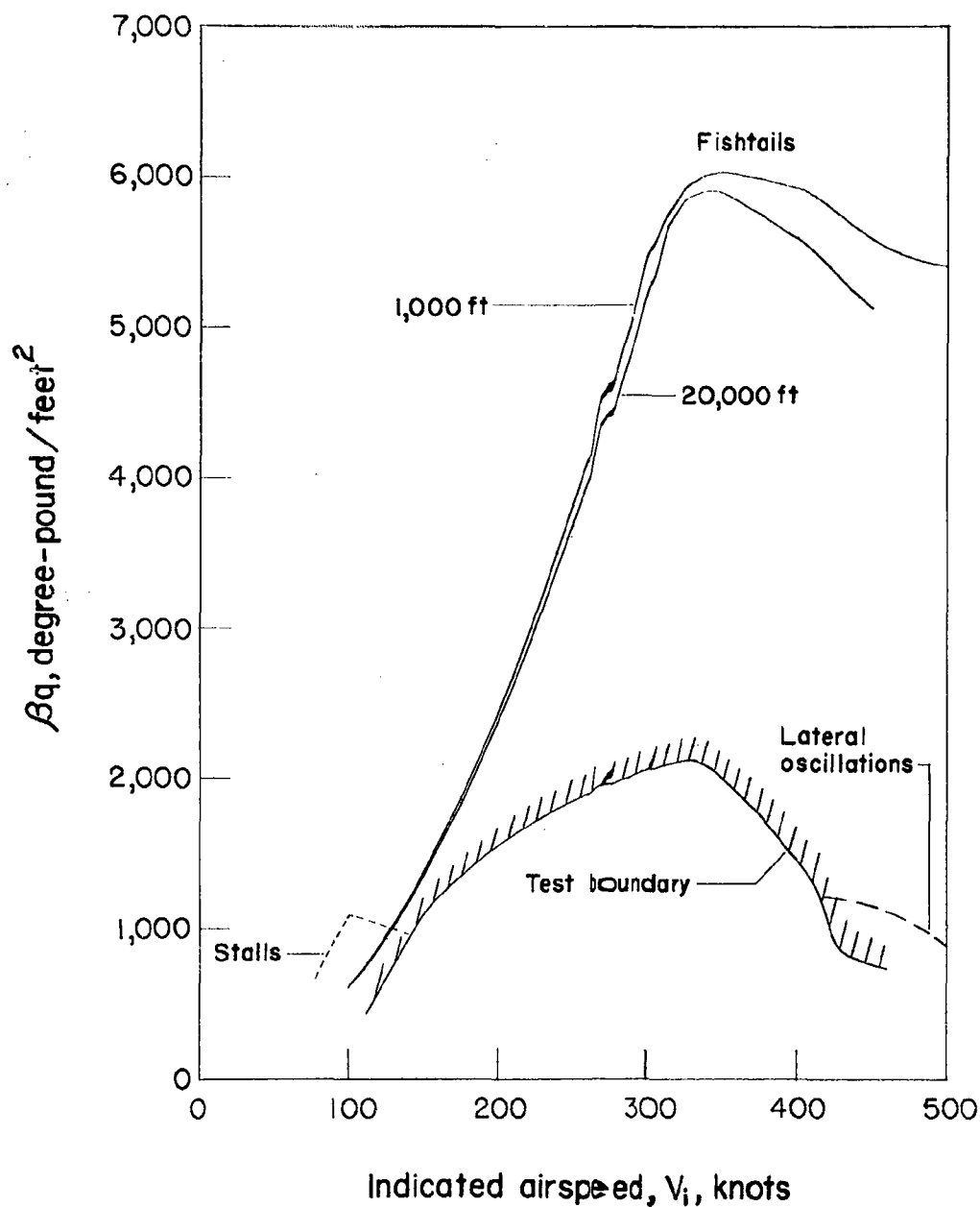
Figure 21.- Comparison of test results for the F-84 airplane with maximum calculated values of vertical-tail load parameter \beta_q during fishtail maneuvers.
