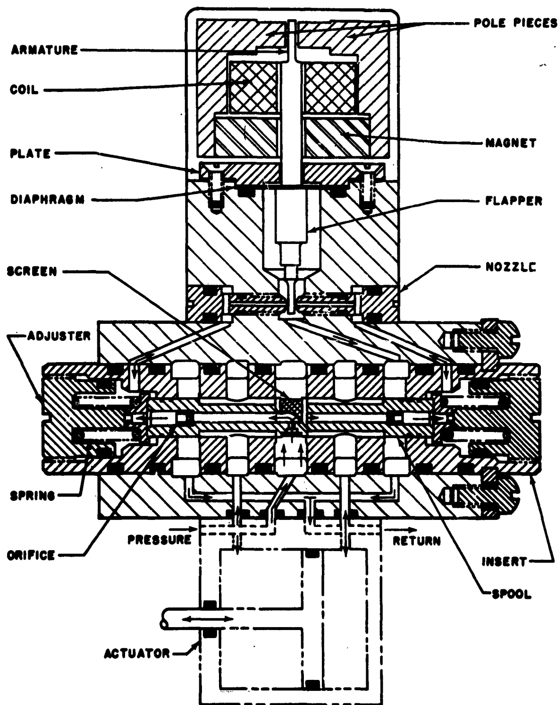
Fig. 7 - Schematic of Bell Valve
