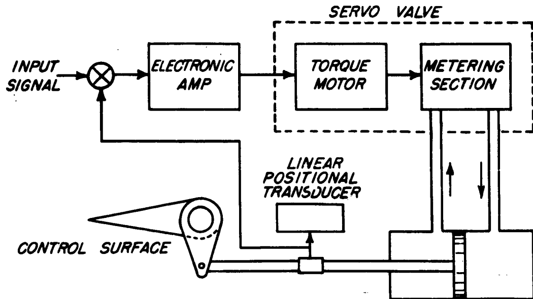
Fig. 2(a) - Servo Valve Positioning Control Surface
