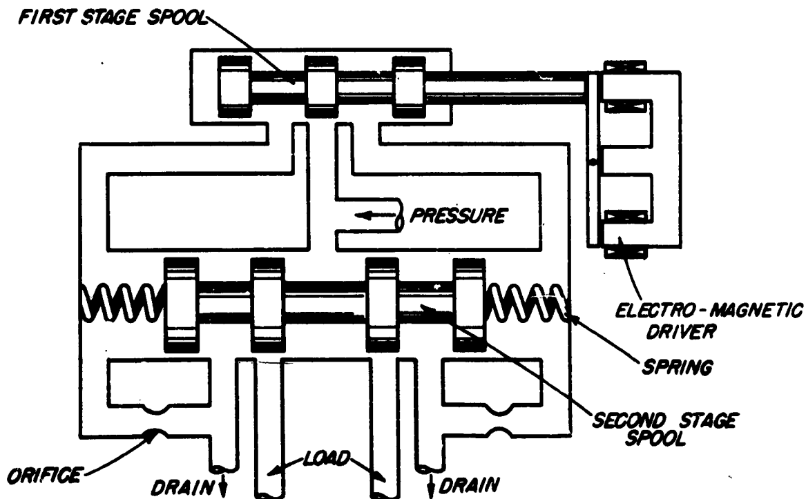
Fig. 17 - Schematic of North American Valve
