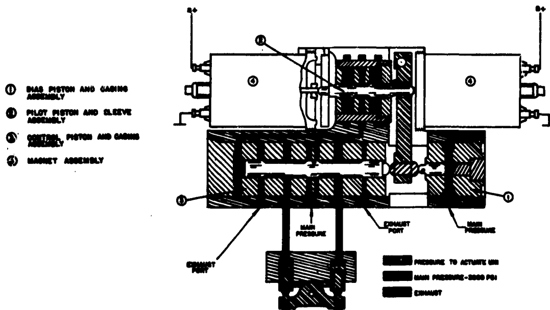
Fig. 18 - Schematic of Raytheon MRTG 65-1 Valve
