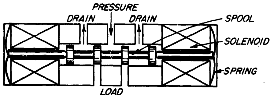
Fig. 4 Schematic of Bendix B-I Valve
