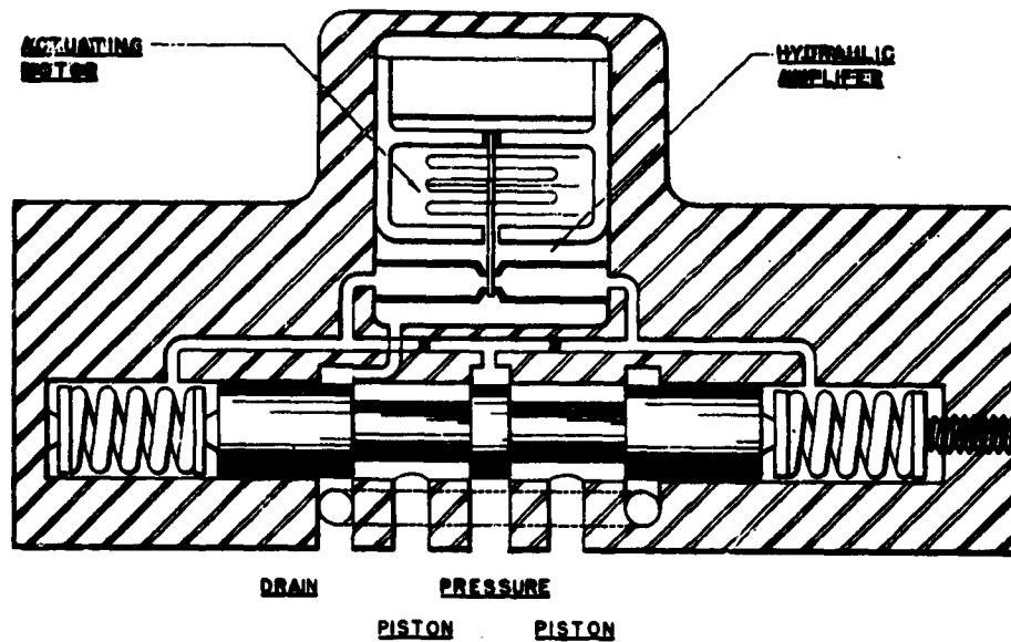
Fig. 10 - Schematic of Moog Valve (Models 500, 900, 1400)
