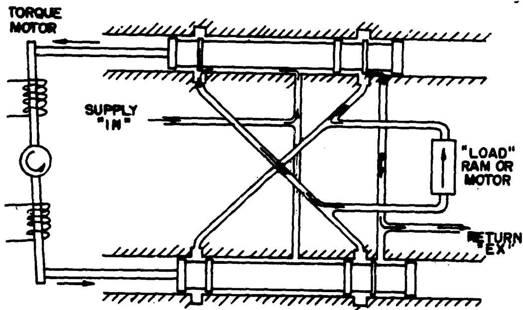
Fig. 6 - Schematic of Midwest Model 4 Valve
