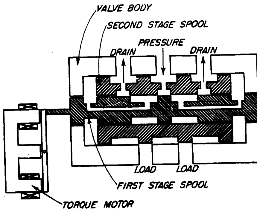
Fig. 14 - Schematic of Cadillac Gage CG-II Valve
