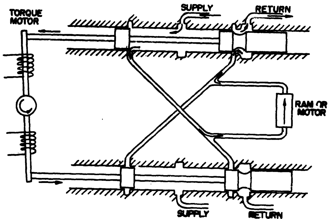
Fig. 5 - Schematic of Midwest Model 3 Valve
