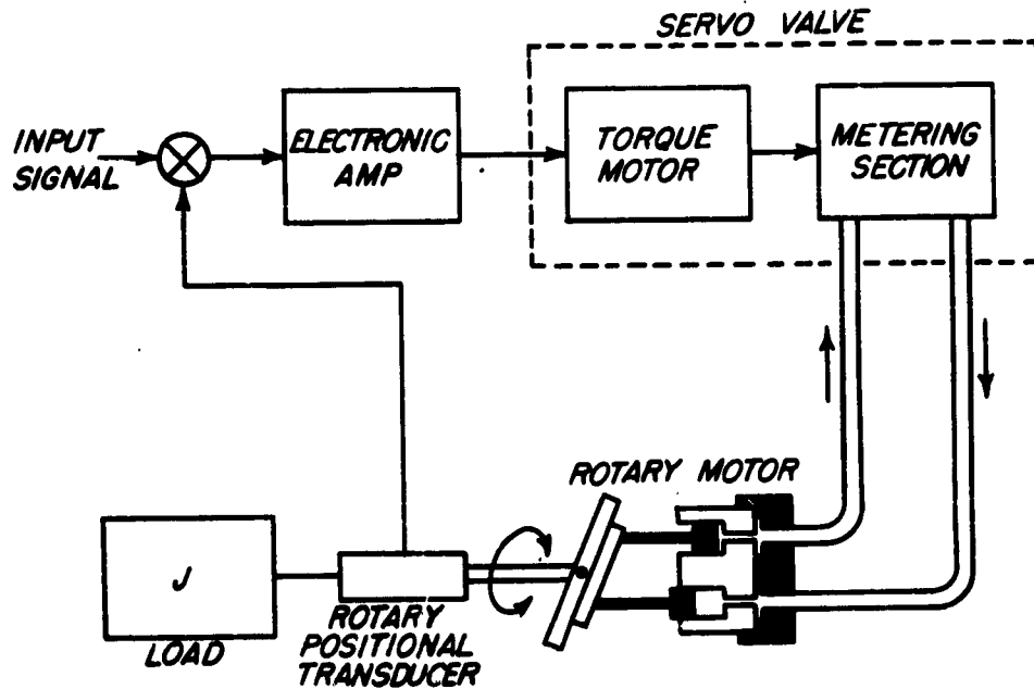
Fig. 2(b) - Servo Valve Driving Rotary Actuator
