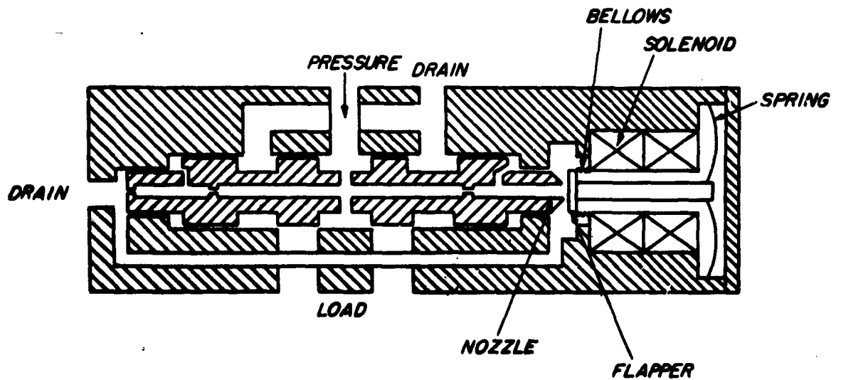
Fig. 12 - Schematic of Pegasus 120-B Valve
