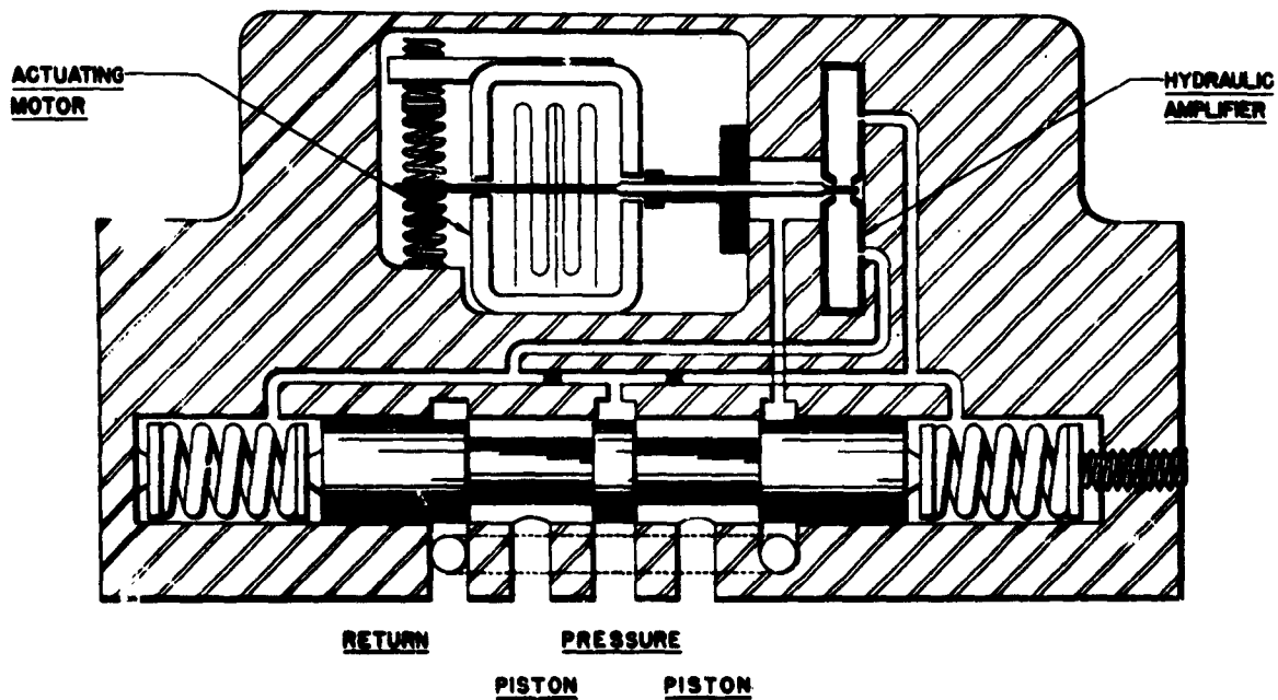
Fig. 11 - Schematic of Moog Model 2000 Valve
