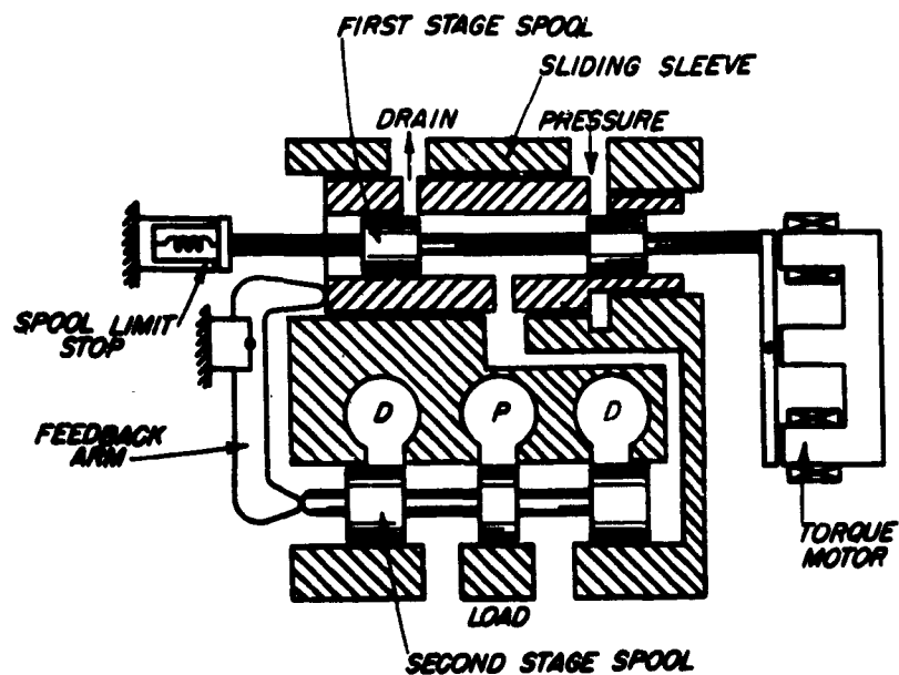
Fig. 19 - Schematic of Sanders Model 10 Valve
