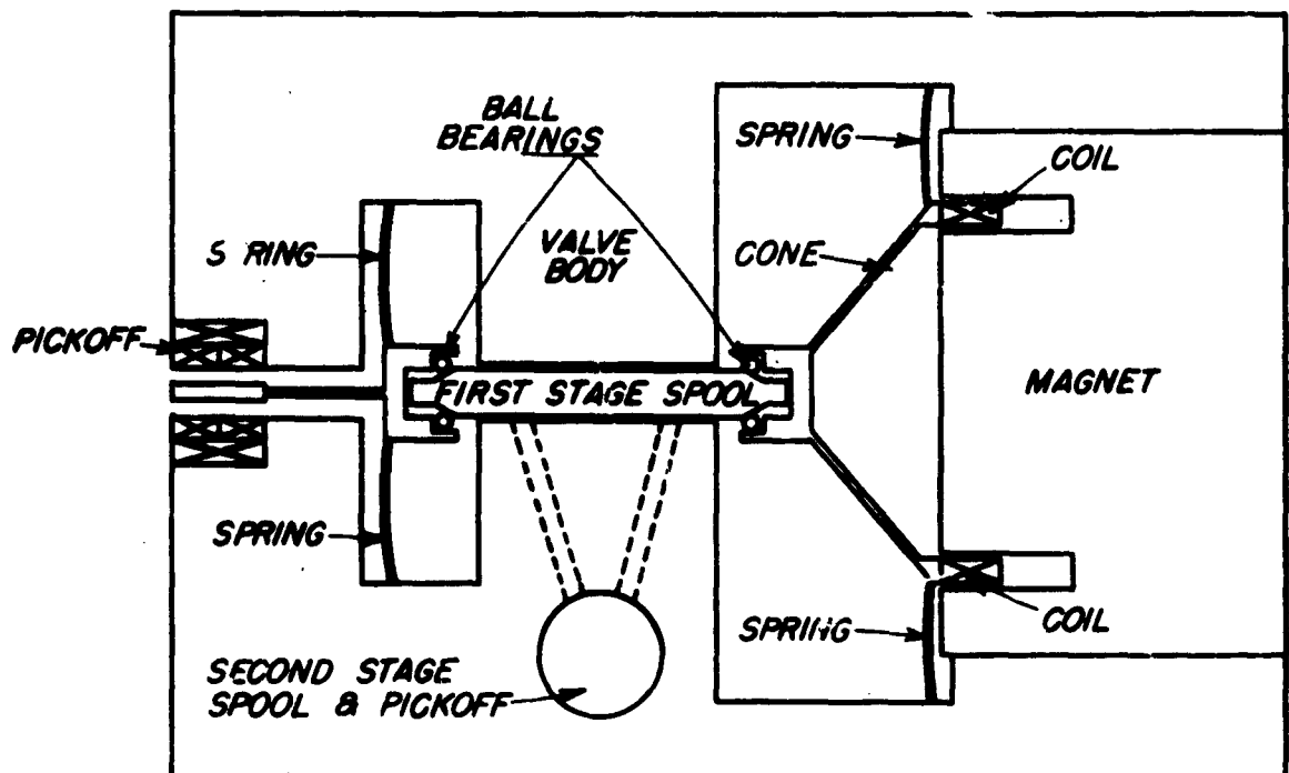
Fig. 13 - Schematic of Bertea (Point Mugu) Valve
