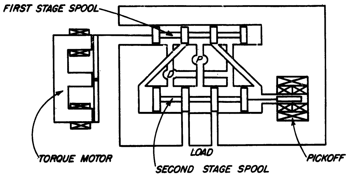
Fig. 16 - Schematic of Hydraulic Controls DS-2 Valve
