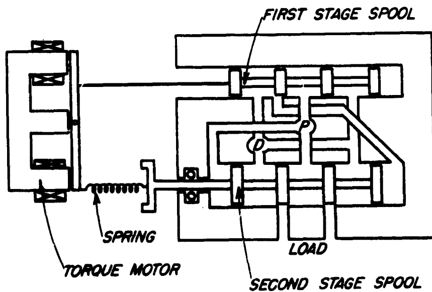
Fig. 15 - Schematic of Drayen-Hanson Valve
