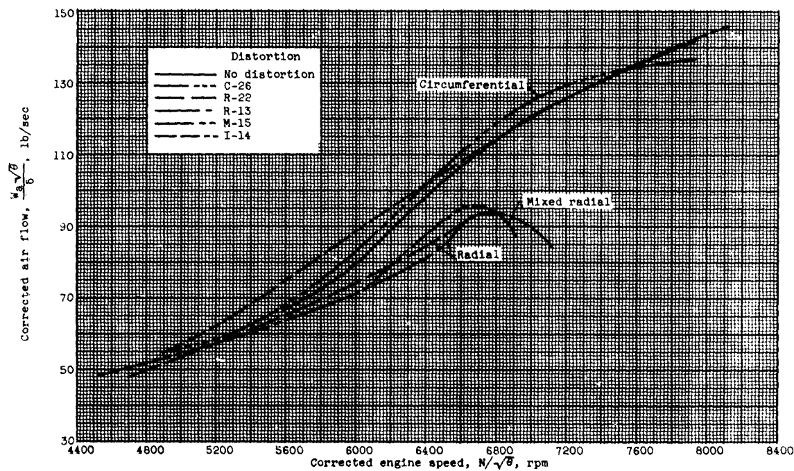
(b) Air flow. Data taken in direction of increasing speed.
