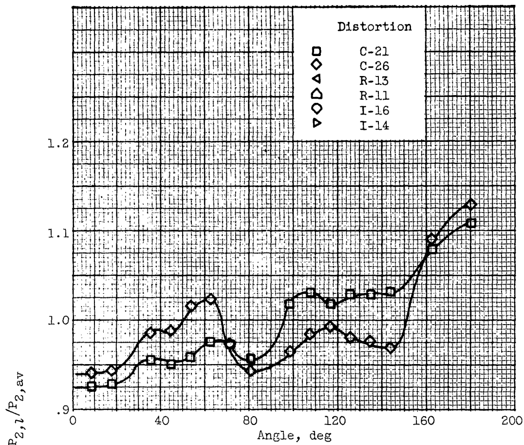
(a) Circumferential distortions.
