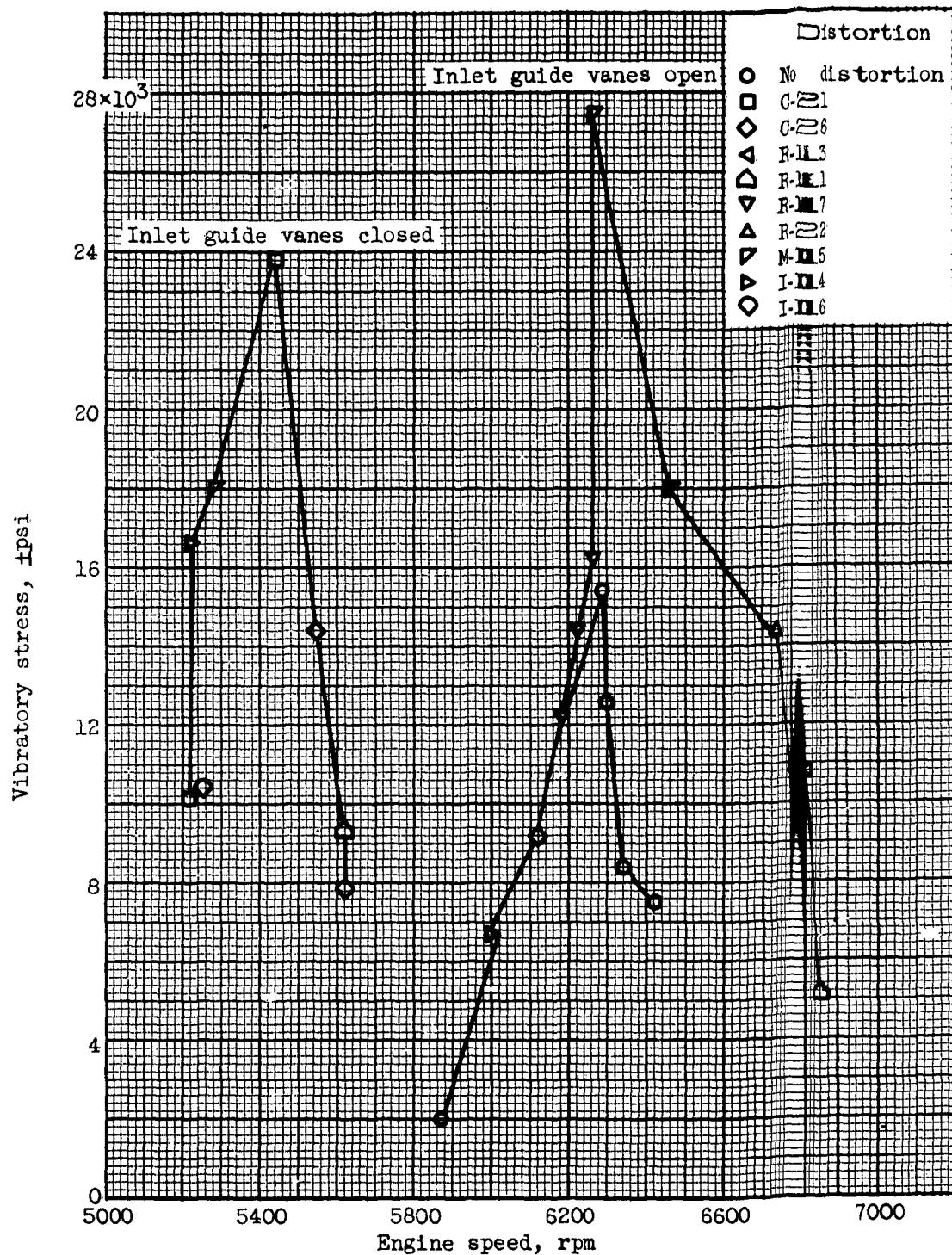
Figure 19. - Concluded. Peak vibratory stress of first-stage rotor blade.
