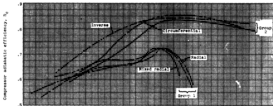
(a) Efficiency. Data taken in direction of increasing speed.
