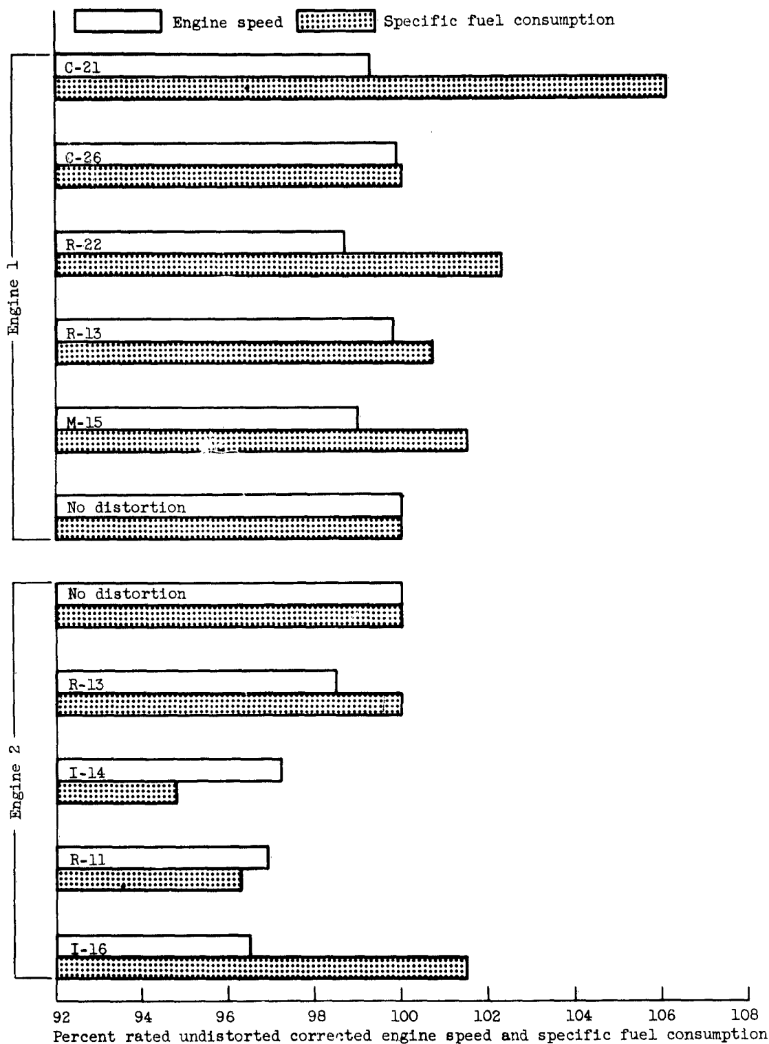
Figure 16. - Effect of distortion on specific fuel consumption at a loiter condition of 30 percent of rated thrust (no distortion).
