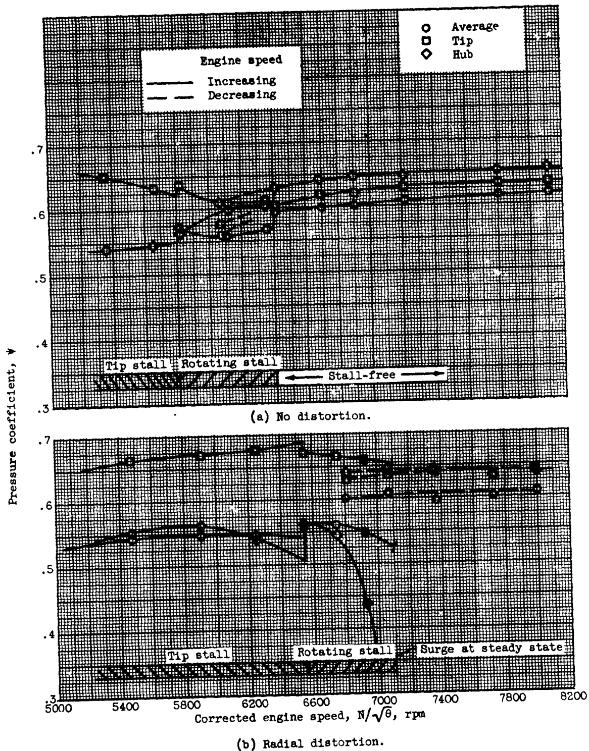
Figure 12. - Effect of radial distortion on characteristics of stages 8 to 10. Inlet guide vanes open; altitude, 35,000 feet; flight Mach number, 0.8.
