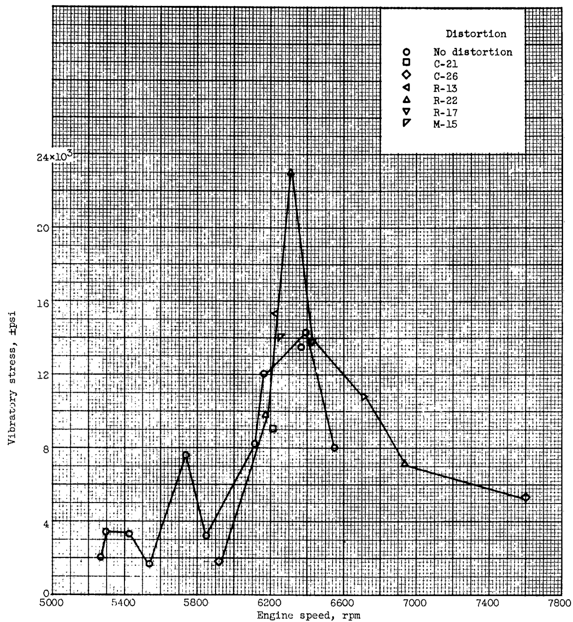
Figure 19. - Peak vibratory stress of first-stage rotor blade.
