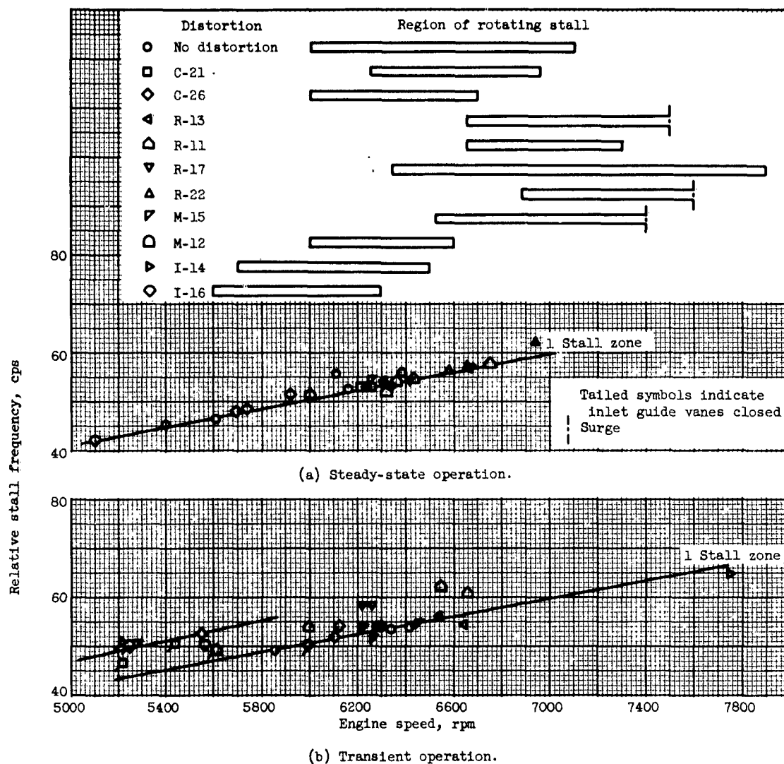
Figure 18. - Variation of relative stall frequency with rotor speed. Inlet guide vanes open.
