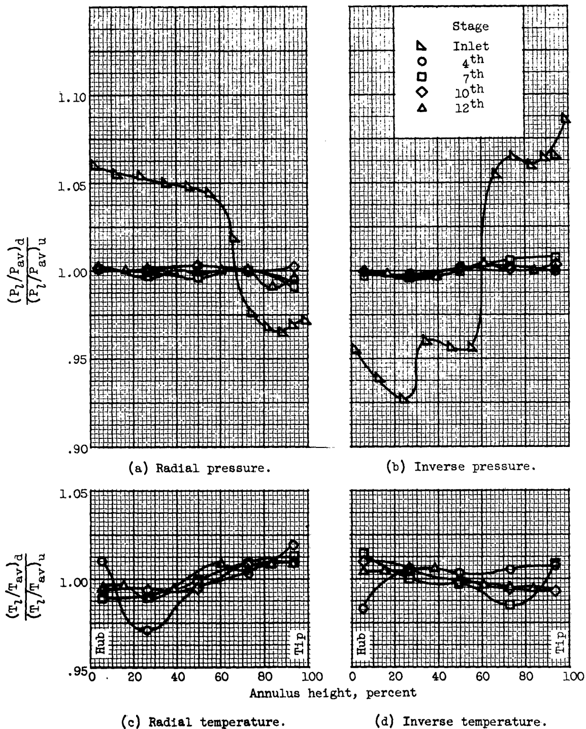
Figure 9. - Typical effects of radial and inverse distortions on compressor-interstage pressure and temperature.
