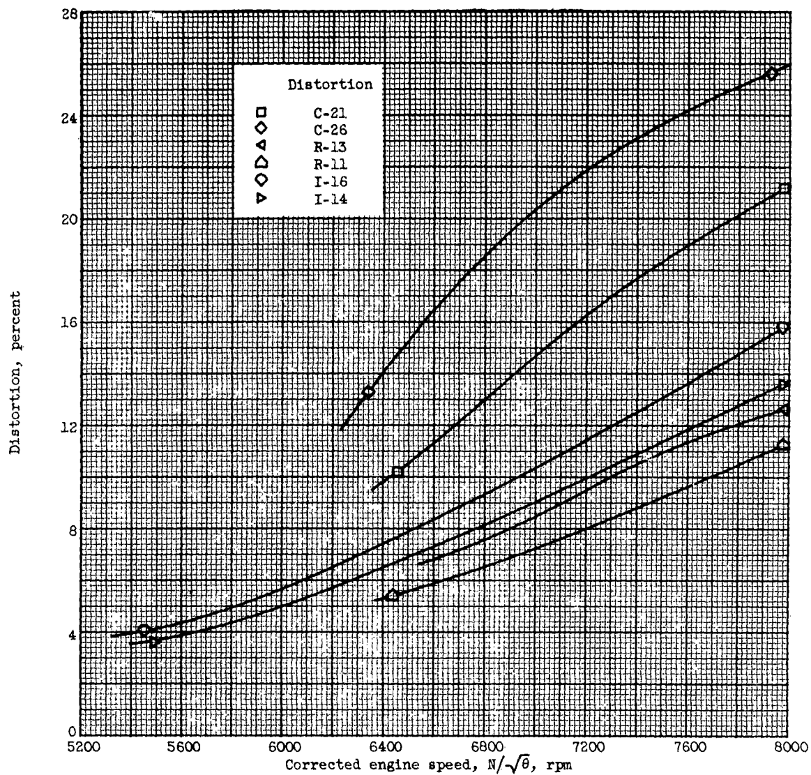
Figure 6. - Variation of distortion with engine speed. Inlet guide vanes open; altitude, 35,000 feet.
