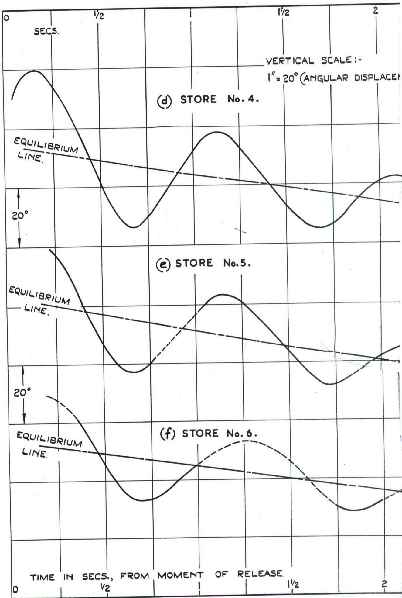
FIG. 6.(d-f). BOMB OSCILLATIONS 500 LB. M.C. BOMB TAIL - TYPE XT UNCLASSIFIED
