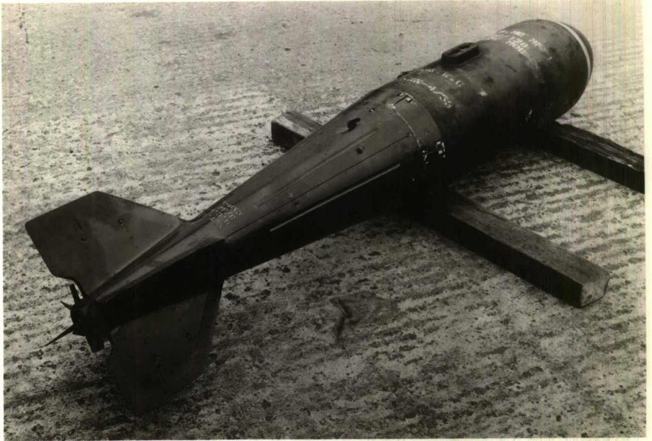
FIG.1a. 500 lb M.C. BOMB WITH TAIL TYPE XTI
