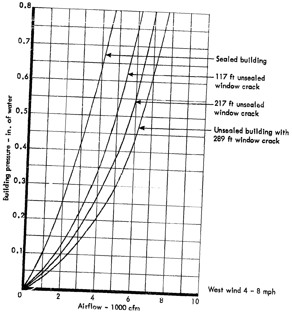
Figure 25. Building-pressurization characteristics.
