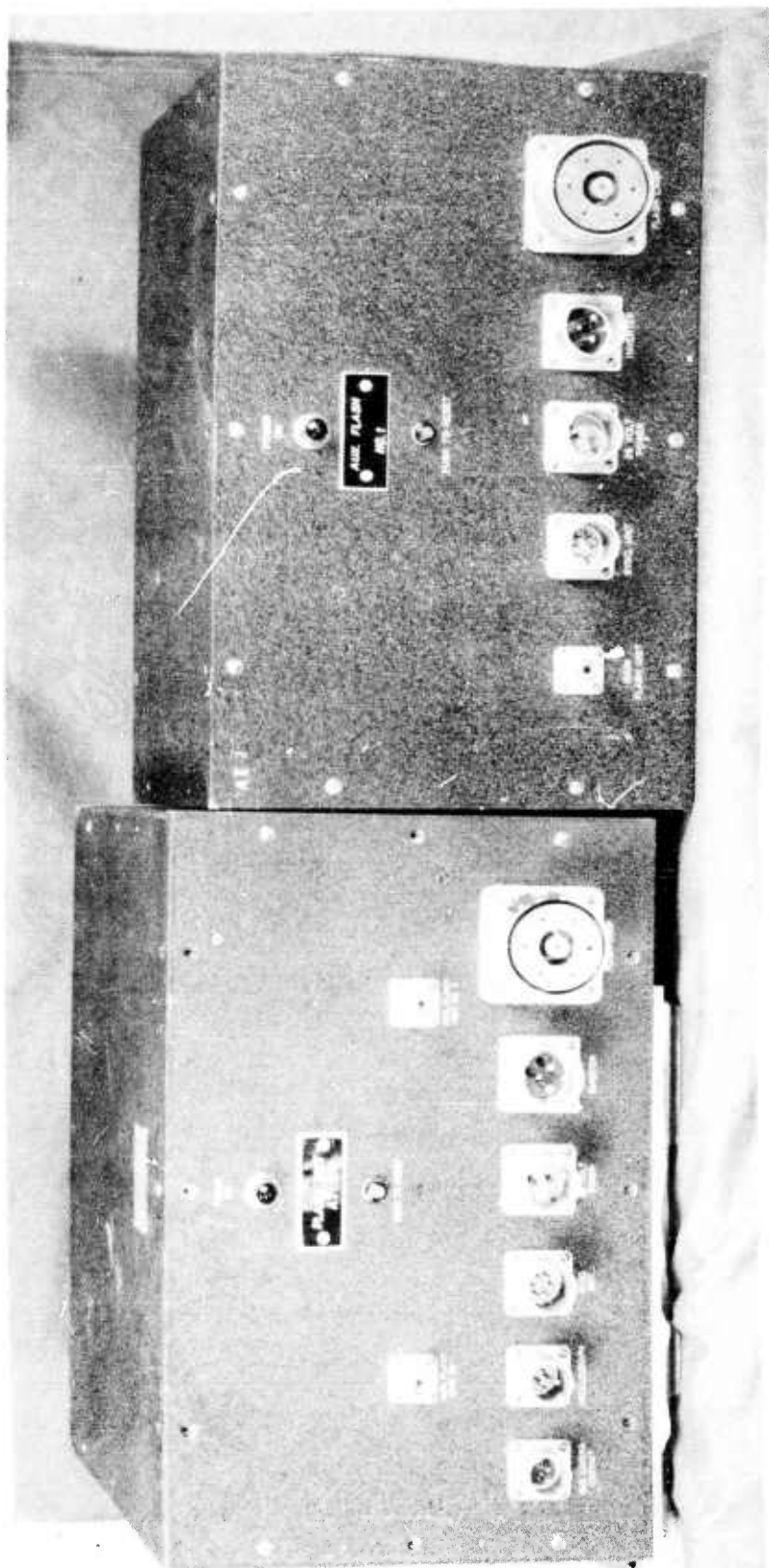
Fig. Ba-l.09. Main Flash Unit (MFU) and Auxiliary Flash Unit (AFU).
