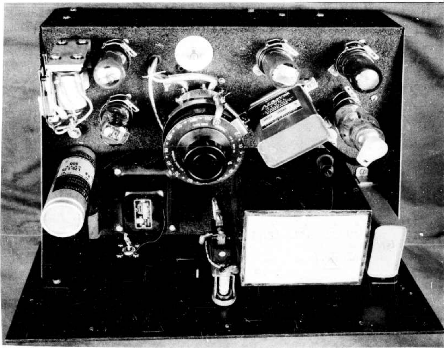
Fig. E a -2.02. Main flash unit AT-1 (MFU), top view.
