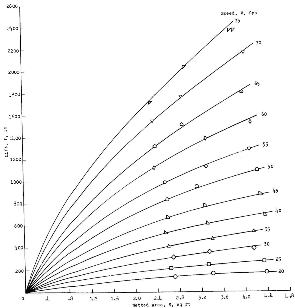
(a) Lift.
