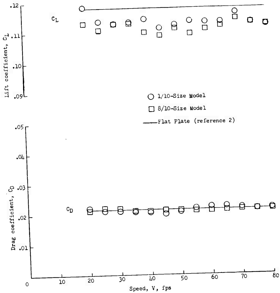
(c) Bare ski at 9^\circ trim.
