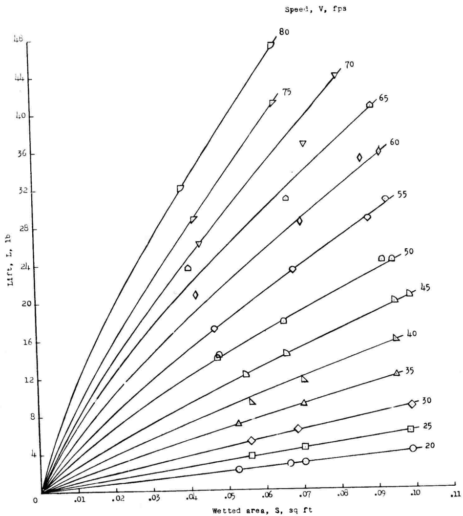
(a) Lift.
