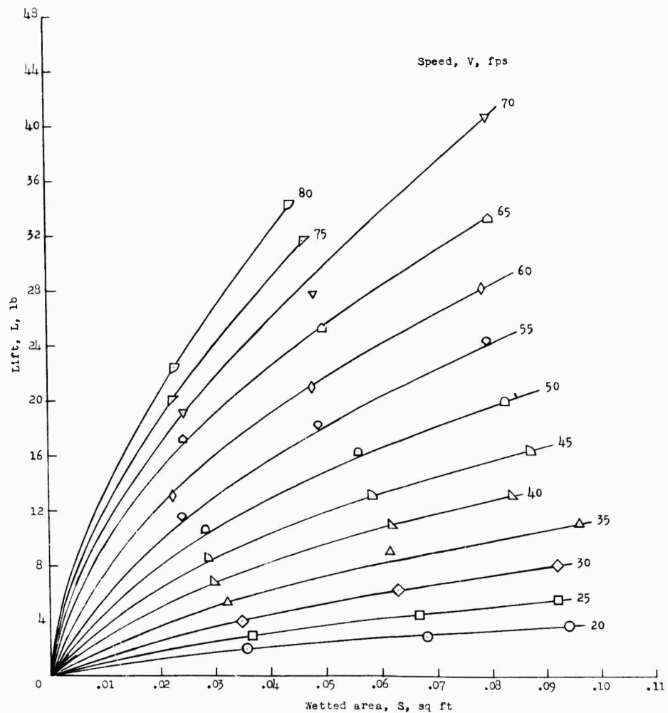
(a) Lift.
