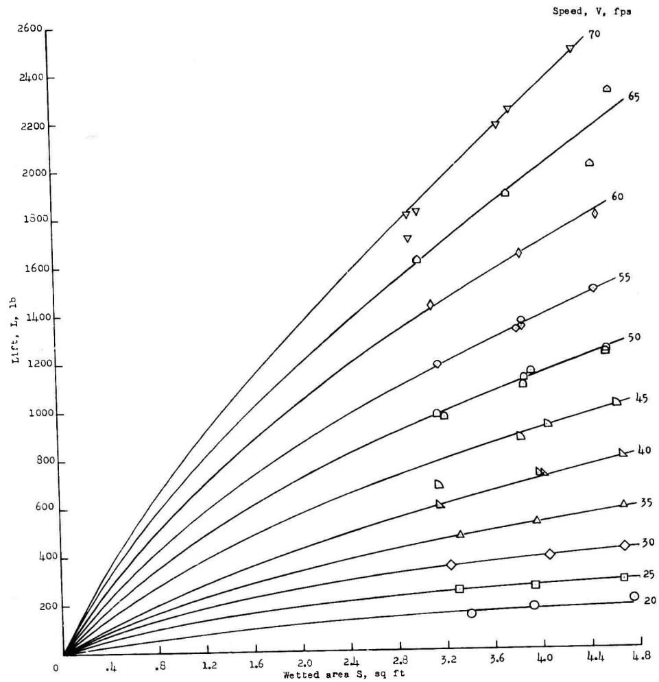
(a) Lift.
