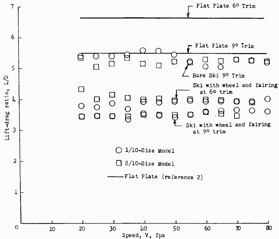
Figure 10.- Variation of lift-drag ratio with speed.
