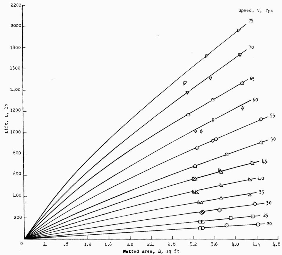
(a) Lift.
