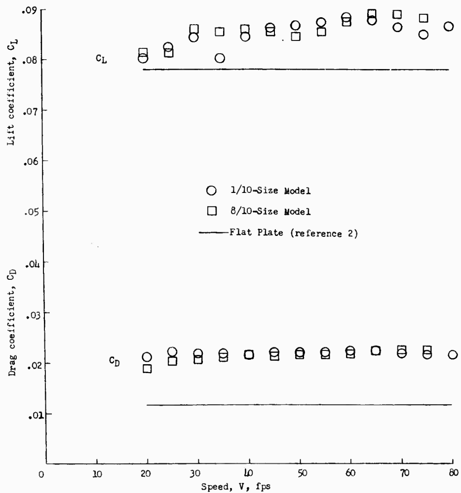
(a) Ski with wheel and fairing at 6^\circ trim.
