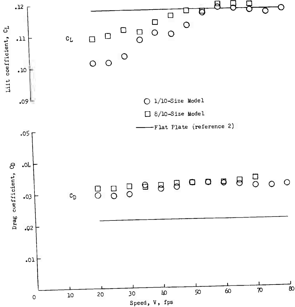
(b) Ski with wheel and fairing at 9^\circ trim.
