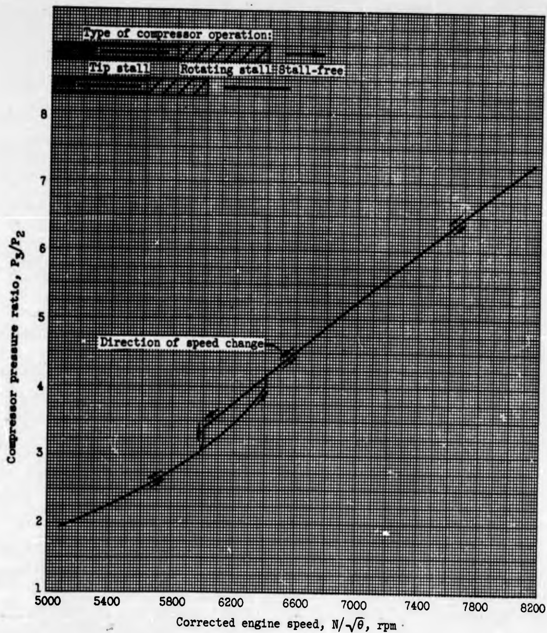
Figure 6. - Steady-state operating line. Altitude, 35,000 feet; undistorted; open inlet guide vanes.
