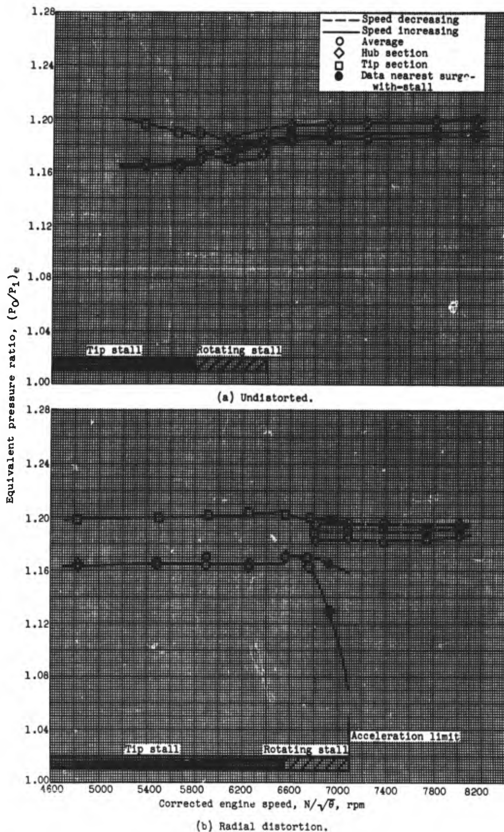
Figure 20. - Effect of radial distortion on equivalent pressure ratio at hub, tip, and average sections of stage group eight to ten. Open inlet guide vanes; altitude, 35,000 feet.
