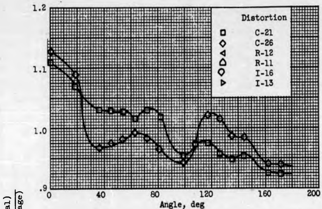
(a) Circumferential distributions.
