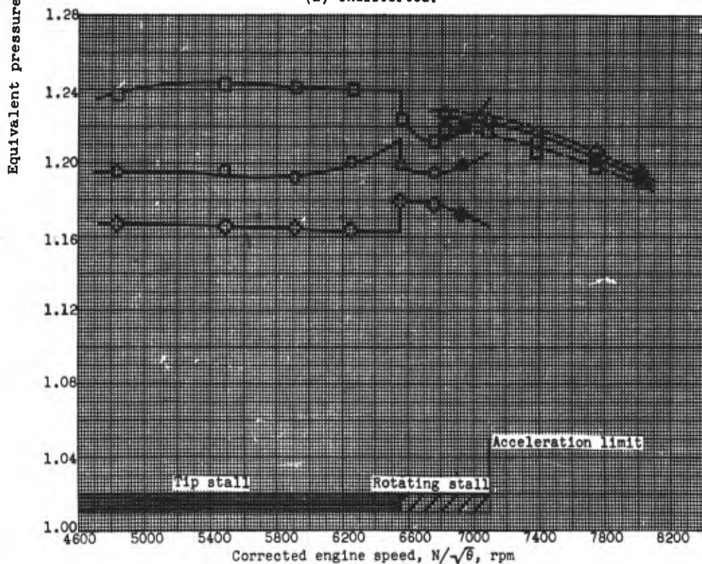
(b) Radial distortion.
