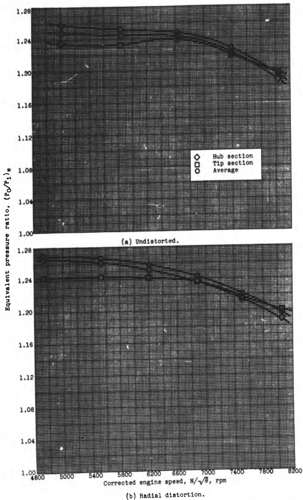
Figure 15. - Effect of radial distortion on equivalent pressure ratio at hub, tip, and average sections of stage five to seven. Closed inlet guide vanes; altitude, 35,000 feet.
