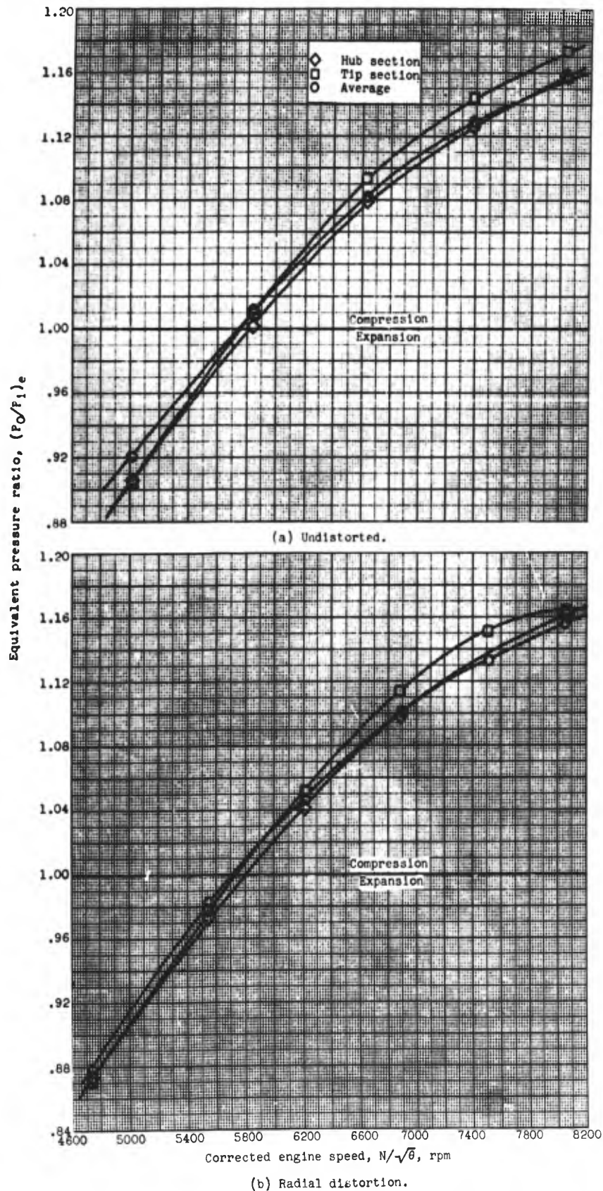
Figure 17. - Effect of radial distortion on equivalent pressure ratio at hub, tip, and average sections of stage group eleven and twelve. Closed inlet guide vanes; altitude, 35,000 feet.
