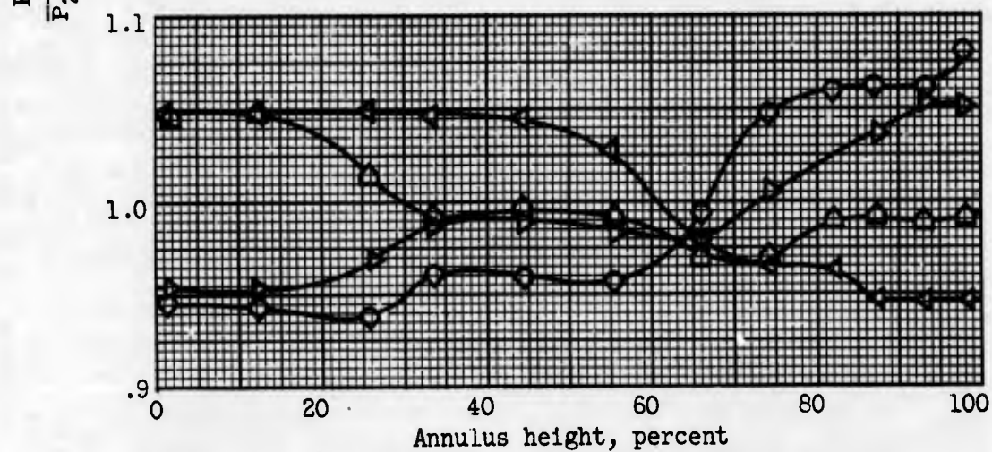
(b) Radial and inverse radial distributions.
