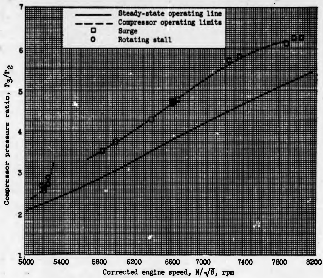
Figure 5. - Compressor operational limits. Undistorted; closed inlet guide vanes; altitude, 35,000 feet.
