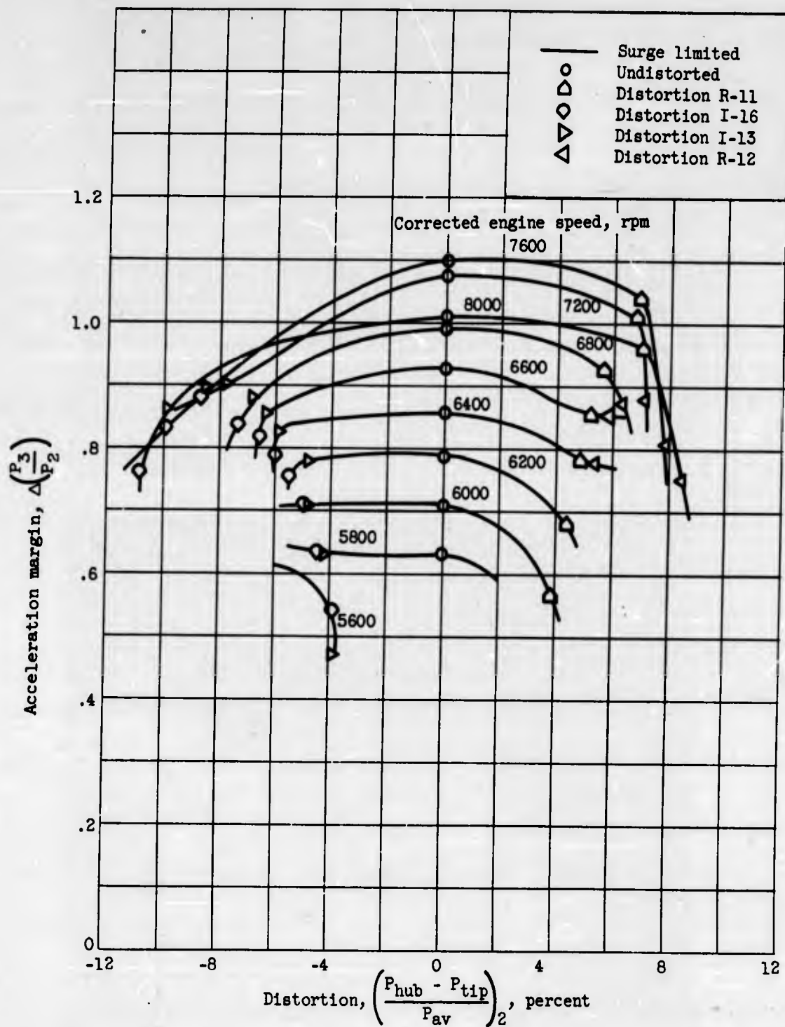
Figure 25. - Effect of radial and inverse radial distortion on acceleration margin. Inlet guide vanes closed; altitude, 35,000 feet.
