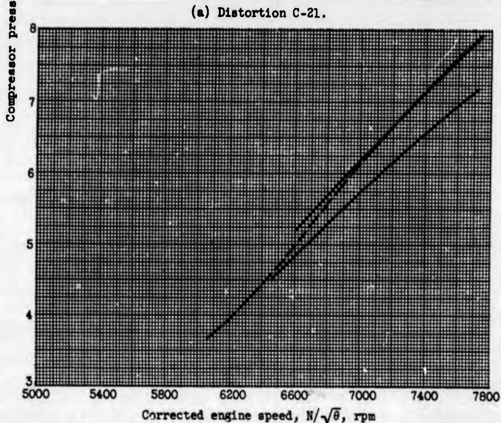
Figure 24. - Comparison of surge pressure ratios for undistorted and circumferentially distorted compressor with minimum inlet pressure. Open inlet guide vanes; altitude, 35,000 feet.
