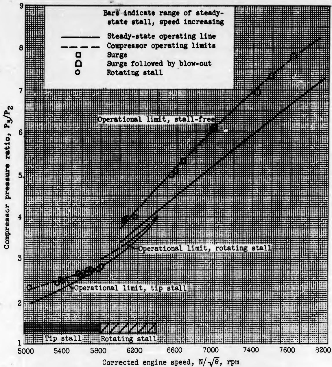
Figure 9. - Compressor operational limits. Undistorted; open inlet guide vanes; altitude, 35,000 feet.
