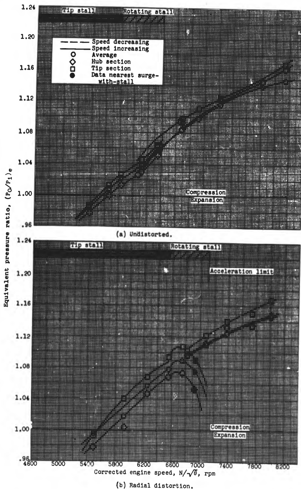
Figure 21. - Effect of radial distortion on equivalent pressure ratio at hub, tip, and average sections of stage group eleven and twelve. Open inlet guide vanes; altitude, 35,000 feet.
