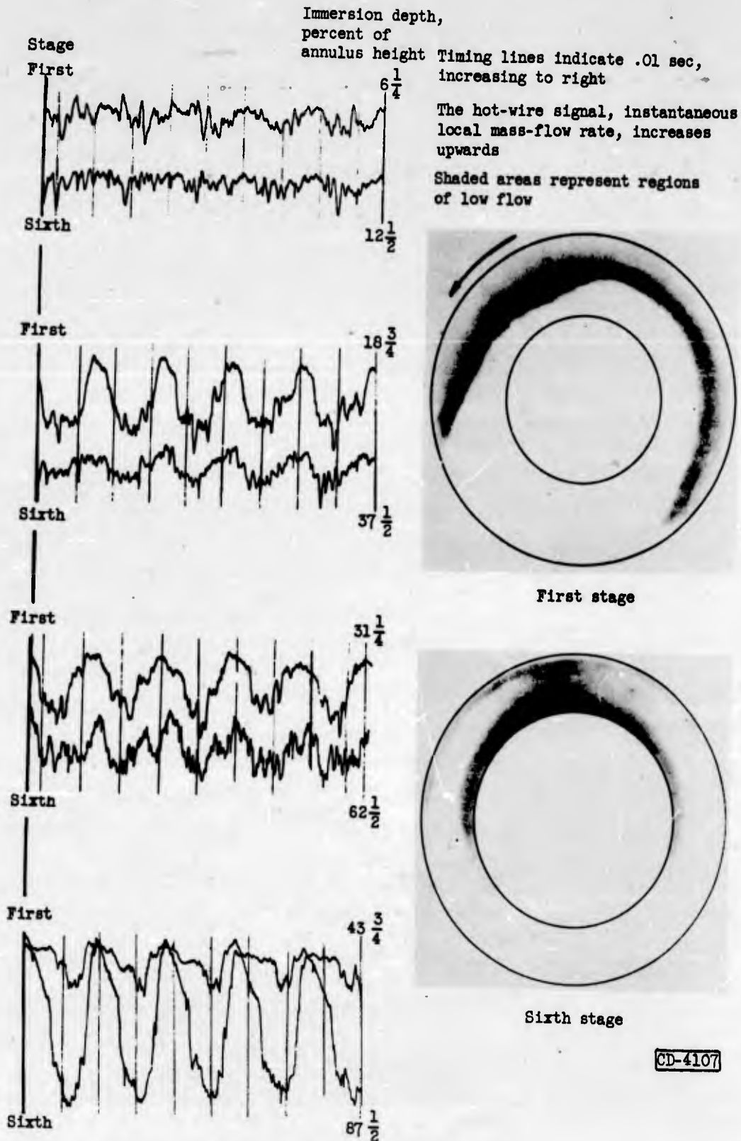
Figure 11. - Anemometer traces and representations of flow fluctuations at first and sixth stages. Operation with radial distortion just prior to steady-state surge; altitude, 35,000 feet; open inlet guide vanes.
