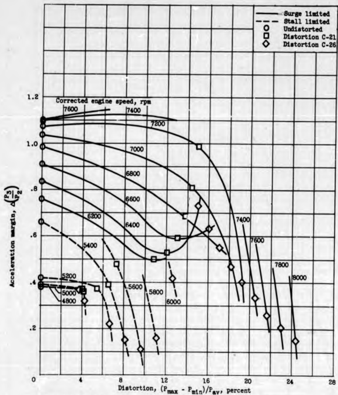
Figure 22. - Effect of circumferential distortion on acceleration margin. Inlet guide vanes closed; altitude, 35,000 feet.
