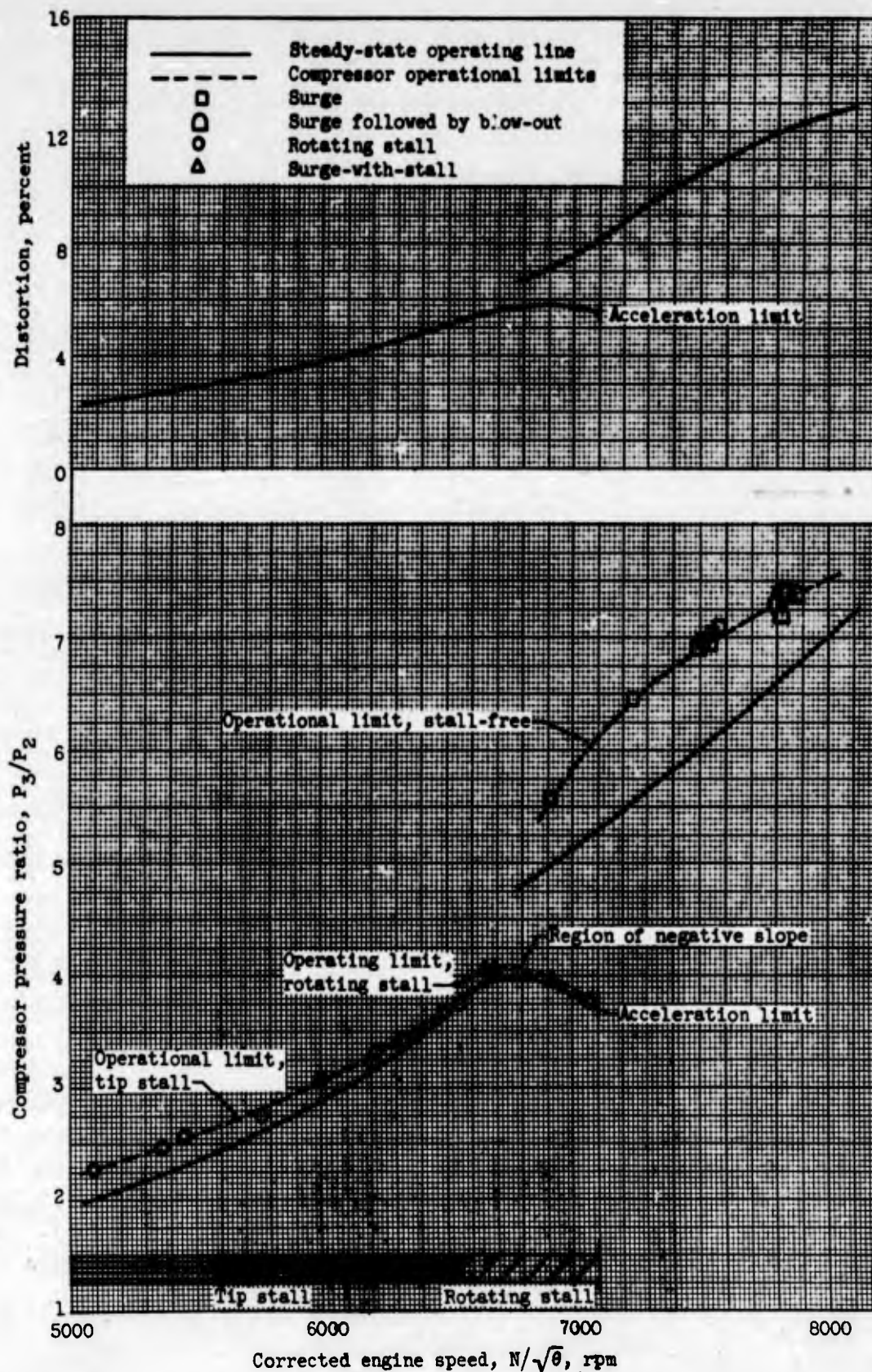
Figure 10. - Compressor operational limits. Radial distortion; open inlet guide vanes; altitude, 35,000 feet.
