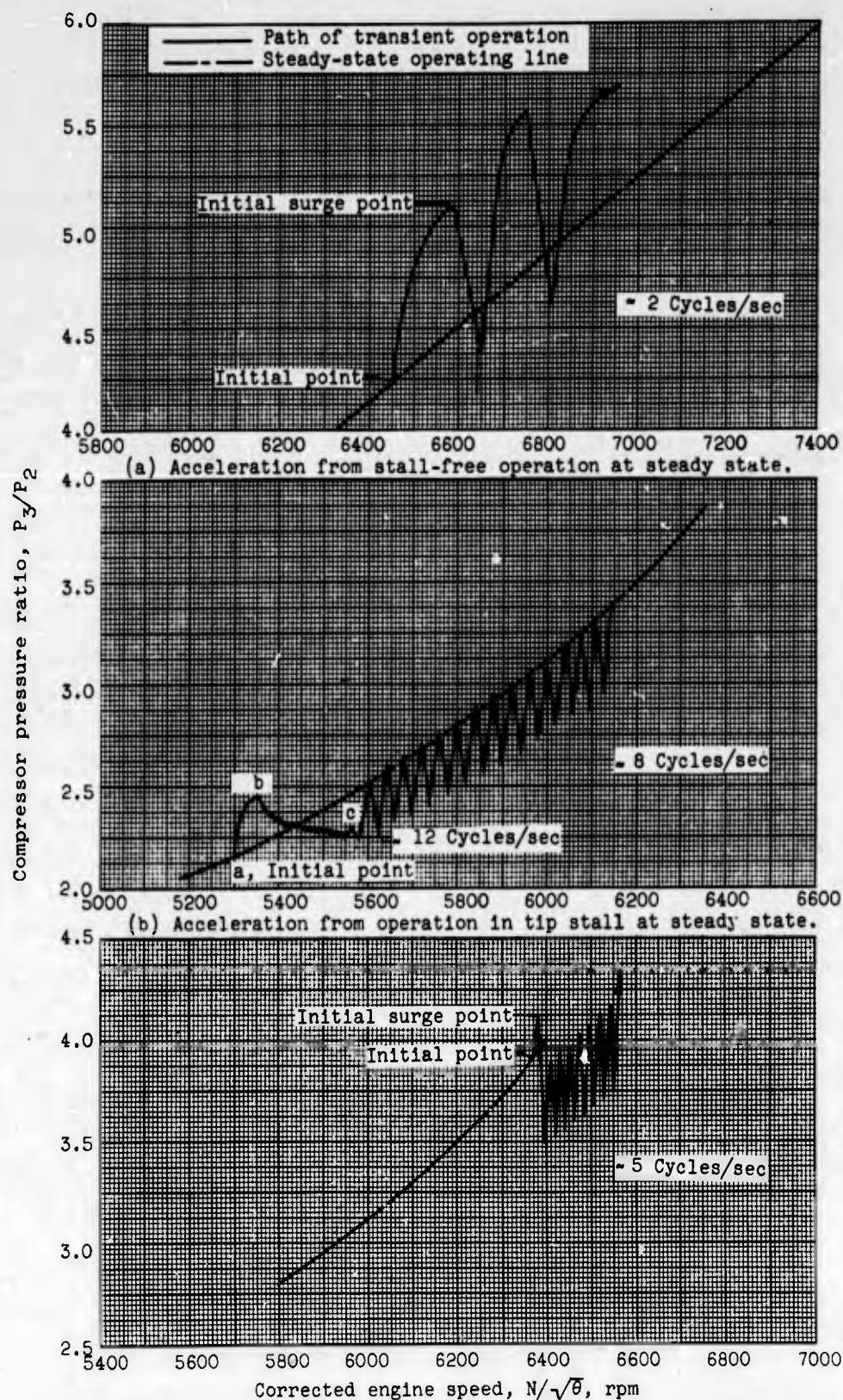
(c) Acceleration from operation in rotating stall at steady state.
