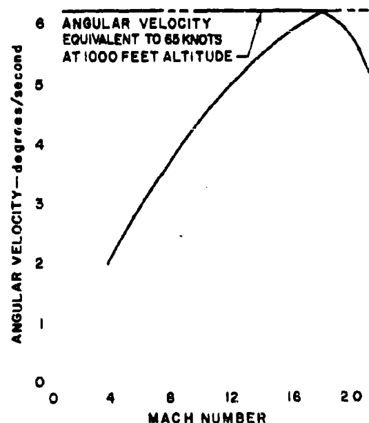
Figure 5. Equivalent Terrain Speed During Cruise of MX-2276
