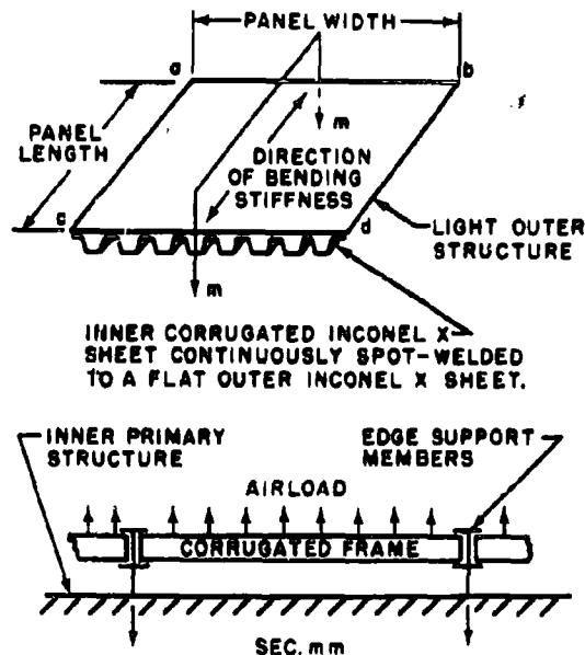
Figure 39. Structural Configuration Principles
