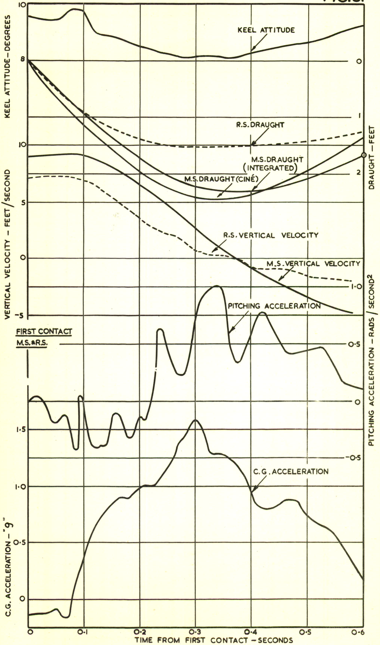
TOTAL IMPACT RESULTS FOR RUN NO 4/11-2-52 V_H = 125 F.P.S.
