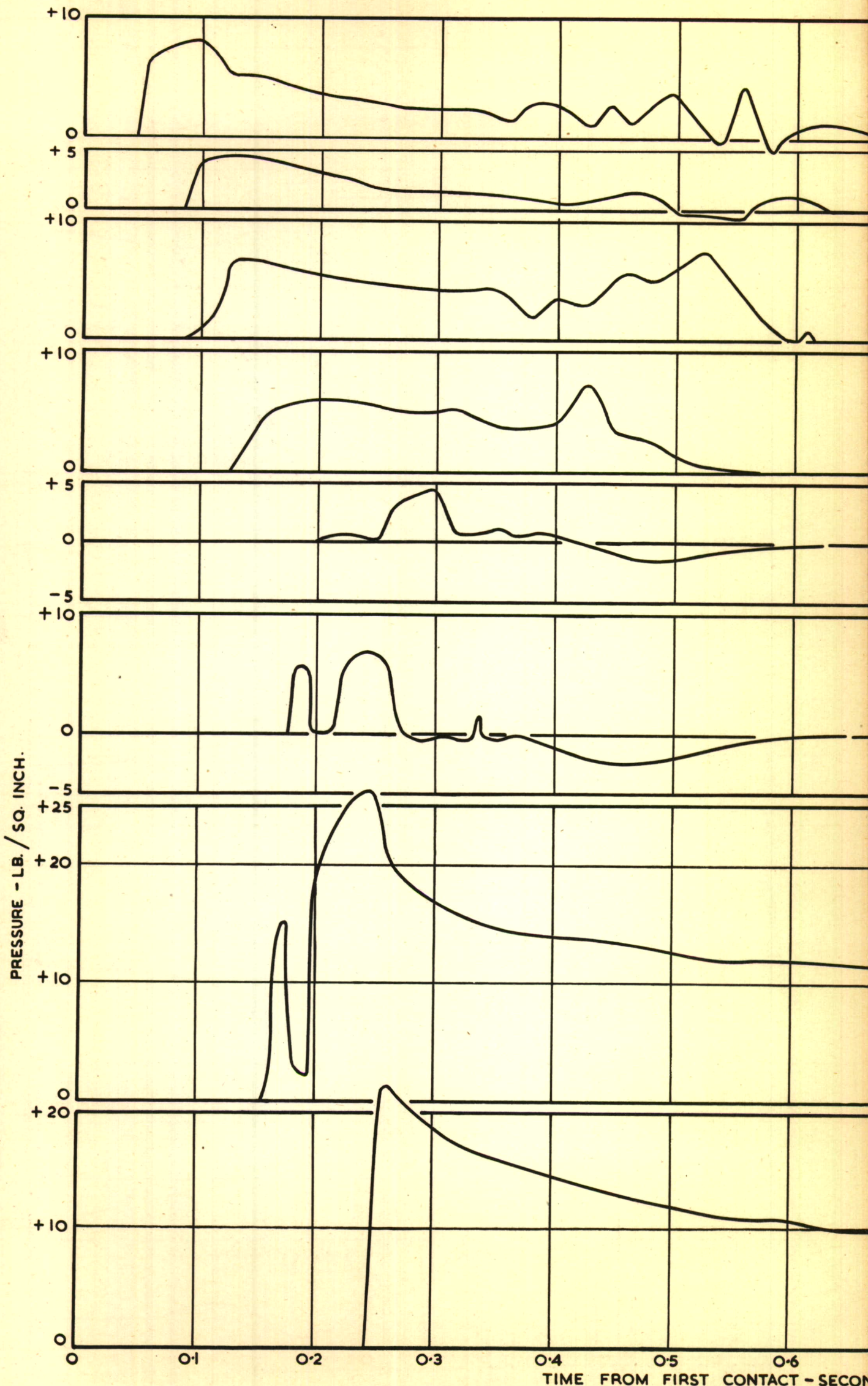
PRESSURE RESULTS FOR RUN NO 2
