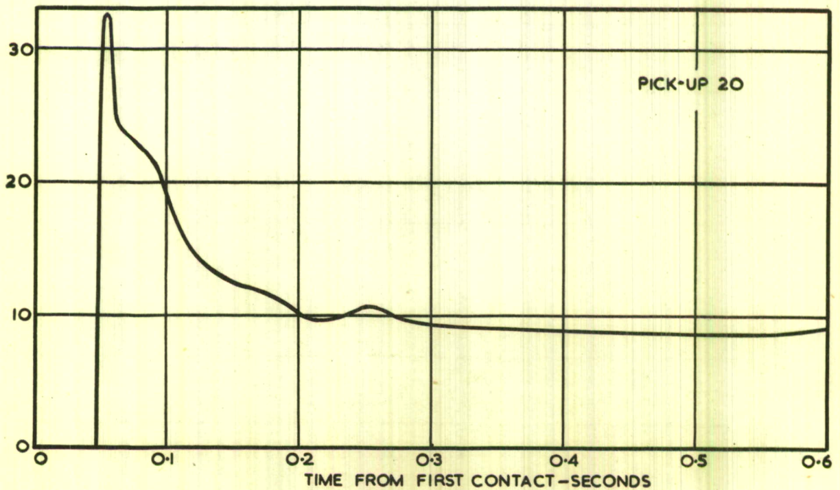
PRESSURE RESULTS FOR RUN NO 11/5-2-52.
