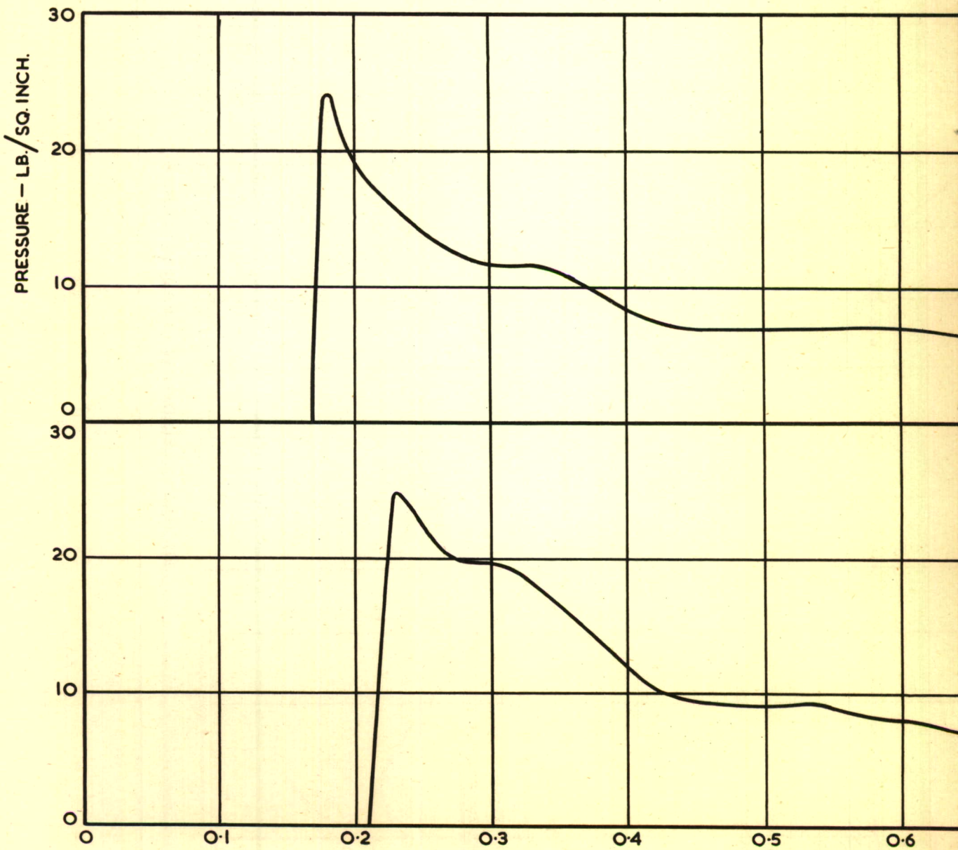
TIME FROM FIRST CONTACT - SEC. PRESSURE RESULTS FOR RUN N°
