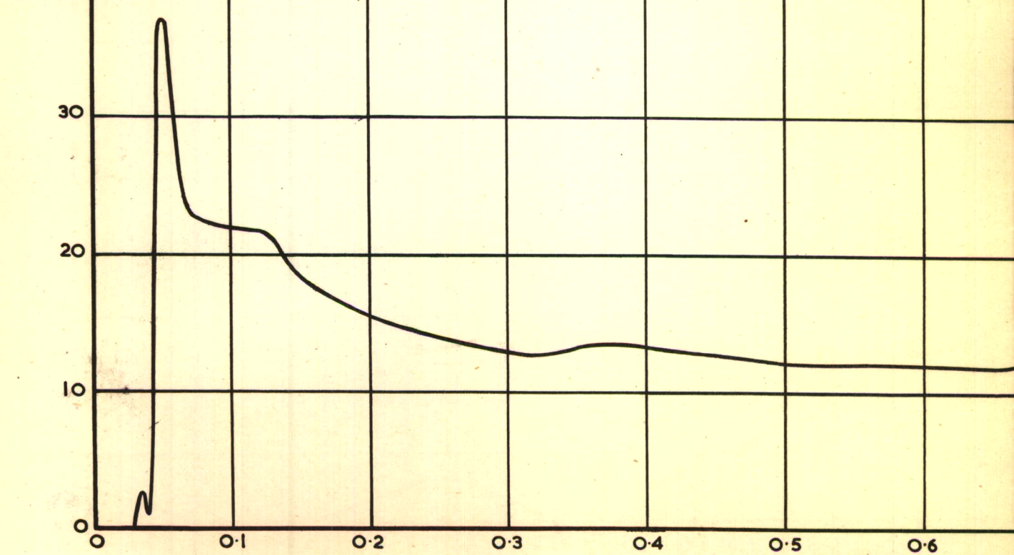
TIME FROM FIRST CONTACT - SECONDS PRESSURE RESULTS FOR RUN N o 13./5
