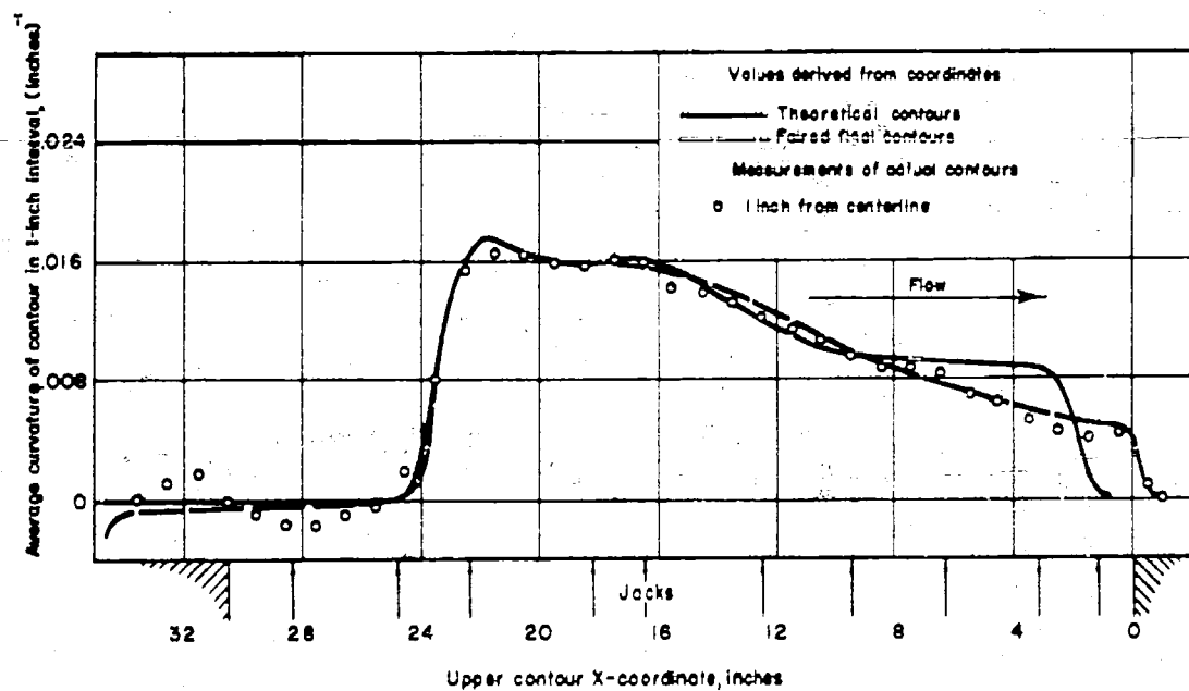
Fig. 2.6. Values of average curvatures in 1-inch intervals for theoretical and final upper contours.
