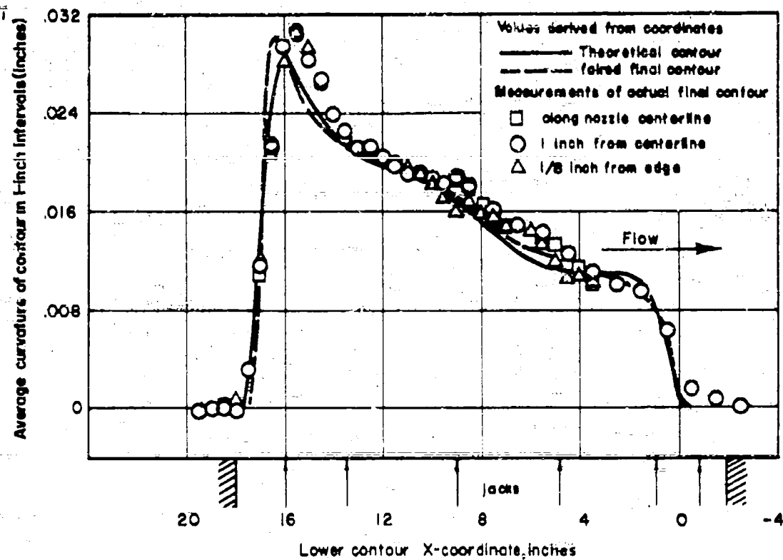
Fig. 2.5. Average curvature of lower contour in 1-inch intervals.
