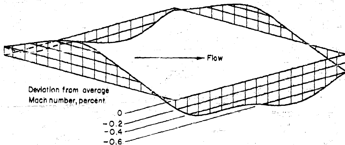
(a) Mach number
