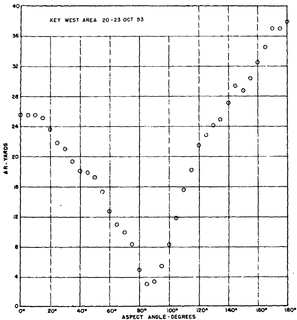
Fig. 5 - Average difference between range measured by Graphic Indicator and range to periscope as computed from Target Locator range as a function of aspect
