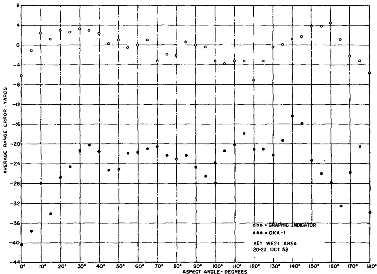
Fig. 15 - Aspect dependence of average-range error. Periscope range derived from Target Locator range as standard.
