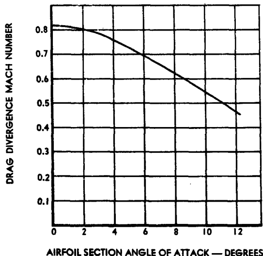
B-1 ASSUMED VARIATION OF BLADE AIRFOIL DRAG DIVERGENCE MACH NUMBER WITH SECTION ANGLE OF ATTACK
