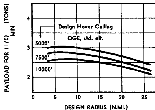
VIII-1 PAYLOAD FOR MINIMUM COST/TON N.M.I. VS. DESIGN RADIUS FOR VARIOUS DESIGN HOVER CEILINGS
