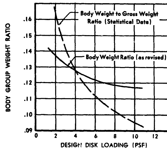
D-2 BODY WEIGHT TO GROSS WEIGHT RATIO VS. DESIGN DISK LOADING
