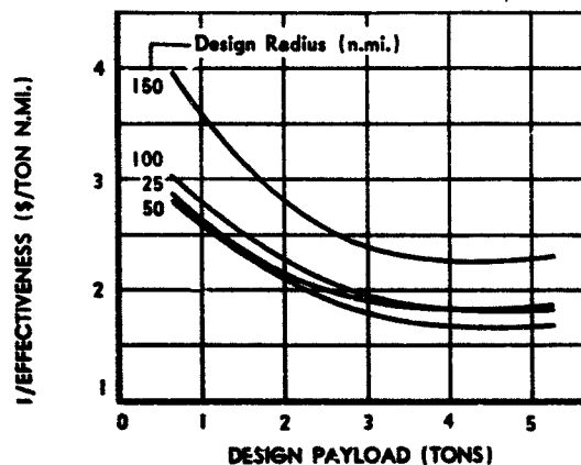
VII-8 COST/TON N.MI. VS. DESIGN PAYLOAD FOR VARIOUS DESIGN RADII
