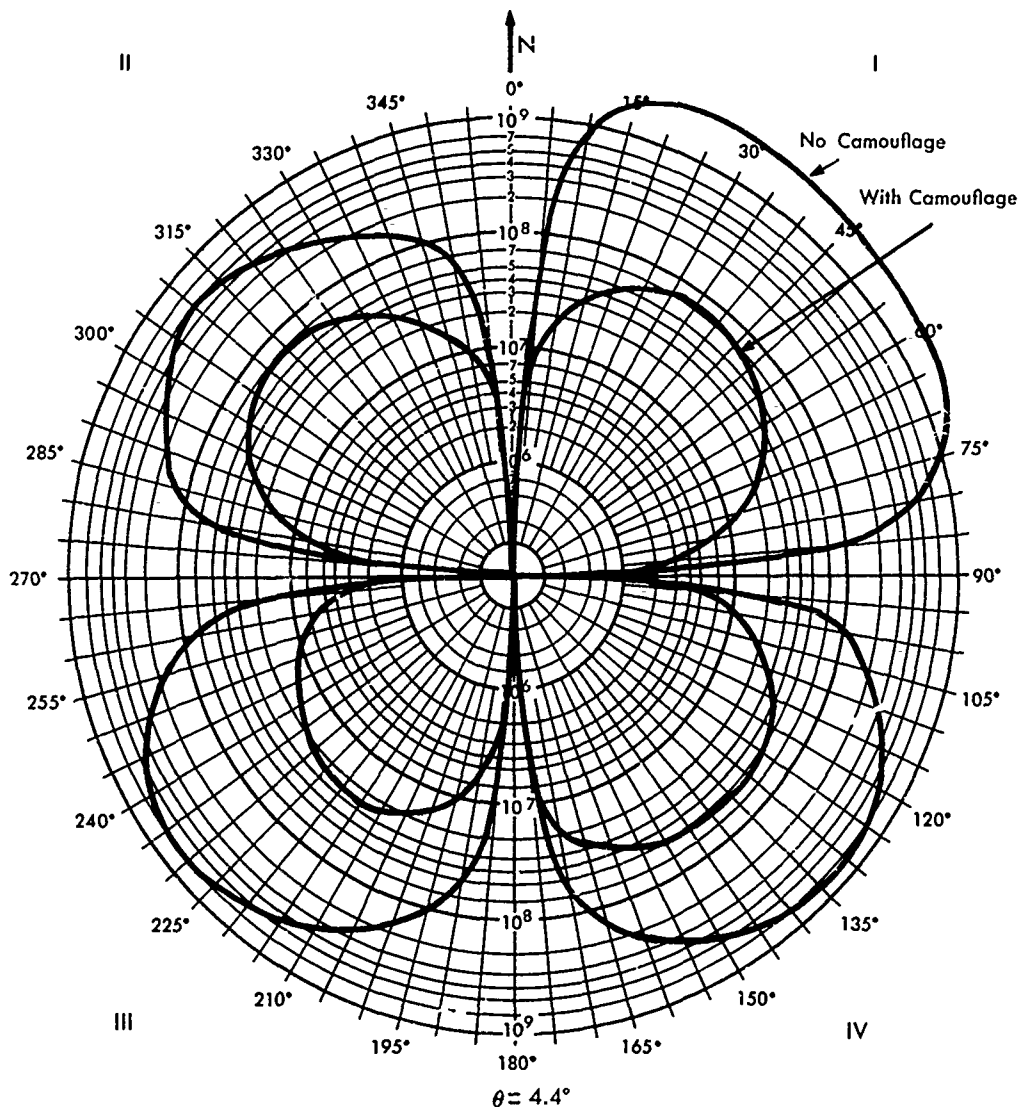
FIG. 3.8b RADAR CROSS-SECTION OF WIRC WITH PRINCIPAL TRIHEDRAL REFLECTORS CAMOUFLAGED; INFINITE CONDUCTIVITY (Compared with the "No Camouflage" case)
