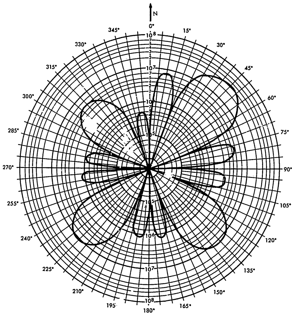
FIG. 3.7 RADAR CROSS-SECTION OF WIRC; DIELECTRIC CONSTANT \epsilon \approx 8 Cross-Section in Square Meters as a Function of Azimuth Angle \phi for \theta = 4.4^\circ and \lambda = 0.03 m.
