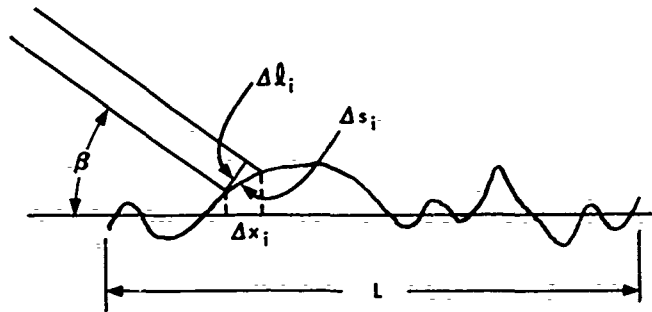
FIG. C-4 GEOMETRY FOR ROUGH SURFACE
