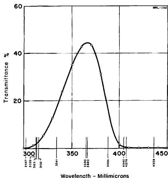
Figure 2. - Transmission of Corning 5840 Filter used to restrict the spectrum of the ultraviolet light adaption field to the 300-400 m \mu . range. Measurements were made with a Beckman Model DU Spectrophotometer. The principle mercury lines in this region are shown.
