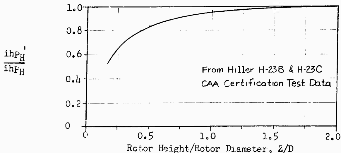
Figure 2-21: Ground Effect
