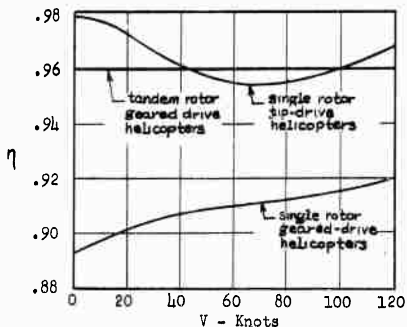
Figure 2-26: Propulsive Efficiency vs. V
