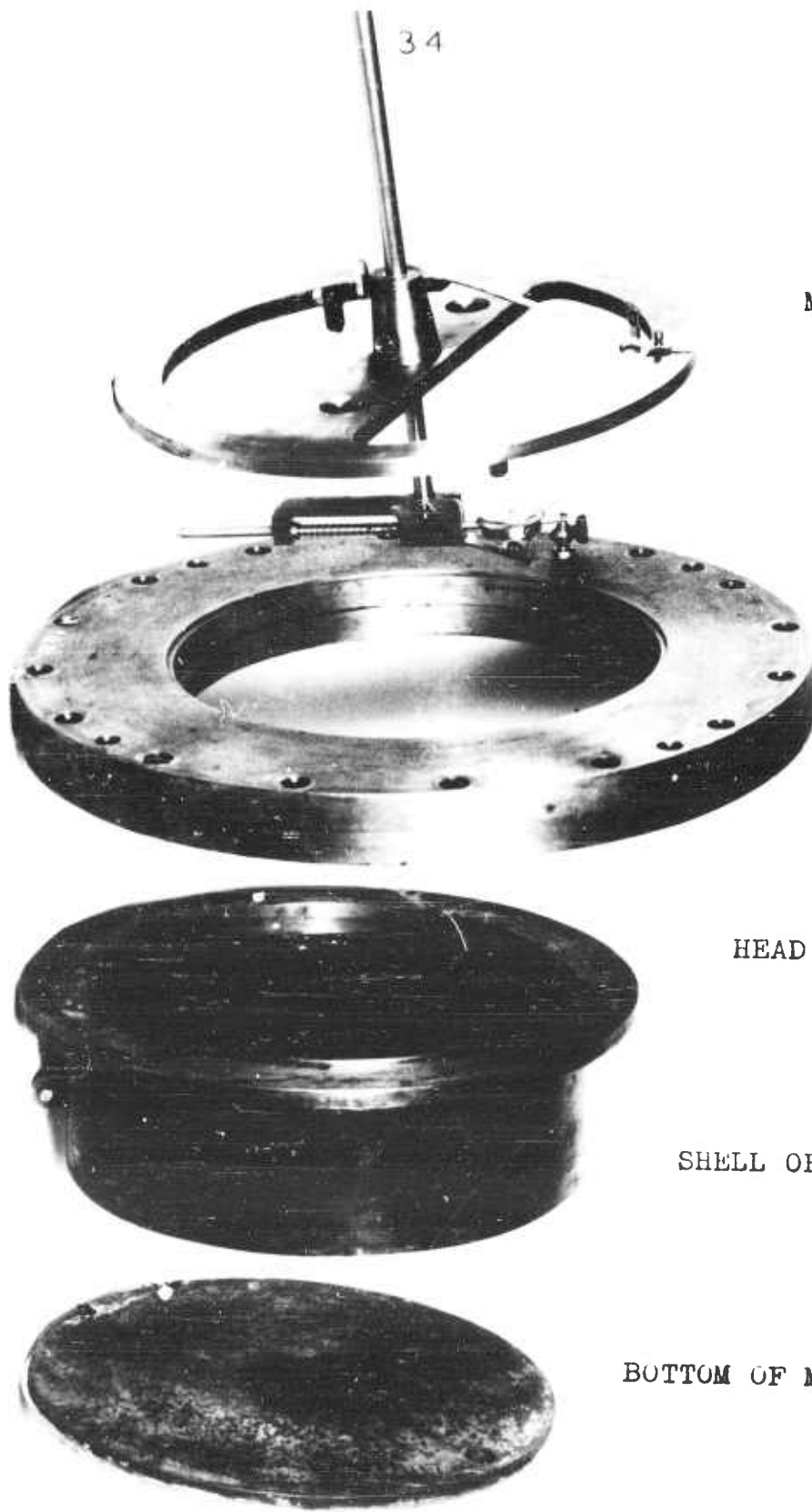
HEAD FOR COMPRESSION TANK.
