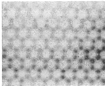
(b) V_{sw} = 0.67
