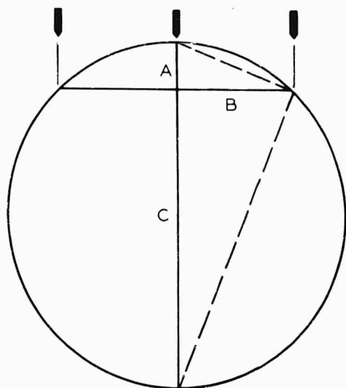
Figure 2. Method of Calculating Radius of Curvature. Geometrical construc- tion for determining average radius of curvature (using lensometer dial gauge) for the arc between the heavy arrows, right and left. Equations below are involved. A and B are known or meas- ured values.
