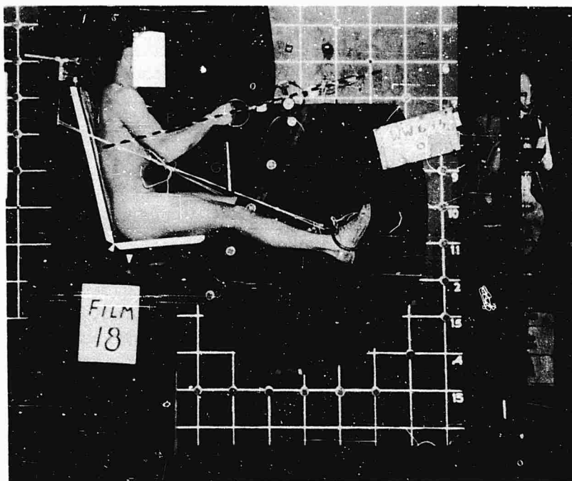
Figure 31. Sample Record for Hand-Pull Force-Vector Analyses. Side-view and a mirror-image front view of a subject pulling on a hand dynamometer in the force vector procedure. The vertical panel with a grid of 6-inch squares and with pulleys for dynamometer attachment is shown; foot stirrups and rope provide a bracing for the body.
