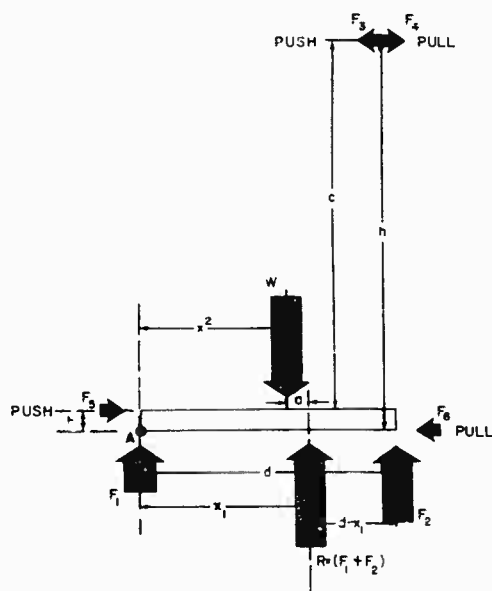
Figure 30. Diagram of force vectors and distances for moment analyses involving the location of whole body centers of gravity and points of effective seat contact.
