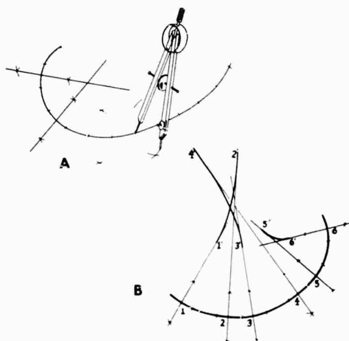
Figure 3. Curves Explanatory of Evolute Analysis.
