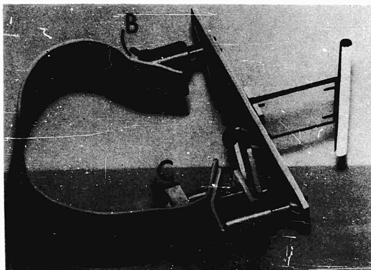
Figure 14. Device for Indicating Pelvic Tilt. Lead belt, formed individually to fit over the bony landmarks of the pelvic brim of a subject, and attached pelvic guide. Foot pieces, or pillars, of the guide, A and B, were adjusted to overlies the anterior superior iliac spines of the subject, and piece C was adjusted until the white guide at the right was vertical ( 0^\circ ) for the standing posture.
