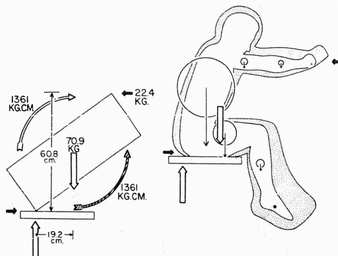
Figure 103. Balanced clockwise and counterclockwise moments are illustrated for a body-push position and for a block analogy. Circles and fine arrows on the sketch to the right represent the position and magnitude of segment-mass vectors which have as their resultant the broad downward arrow acting at the whole body center of gravity. The shaded halo about the figure shows the variability of the positions of body contours found in 10 repeated maximum pushes.
