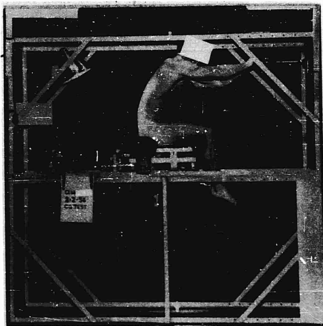
Figure 25. General Arrangements for a Hand-Push Test. Lettered parts are: A—welded support framework; B—seat supported by pressure gauges; C—cameras for recording seat forces; D—hand dynamometer for recording horizontal thrust; and E—hand grip with mirror and spirit level for assuring horizontality.
