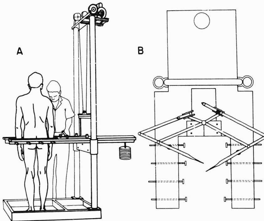
Figure 24. Equipment Used for Body Volume Determinations. Double planimeter mechanism for obtaining area-to-height data. A—The adjustable table surface is shown as set for a lower trunk level; the operator traced the body contour at this level with the pantograph tracer arm. B—Plan of table top and two pantographs on a common post.
