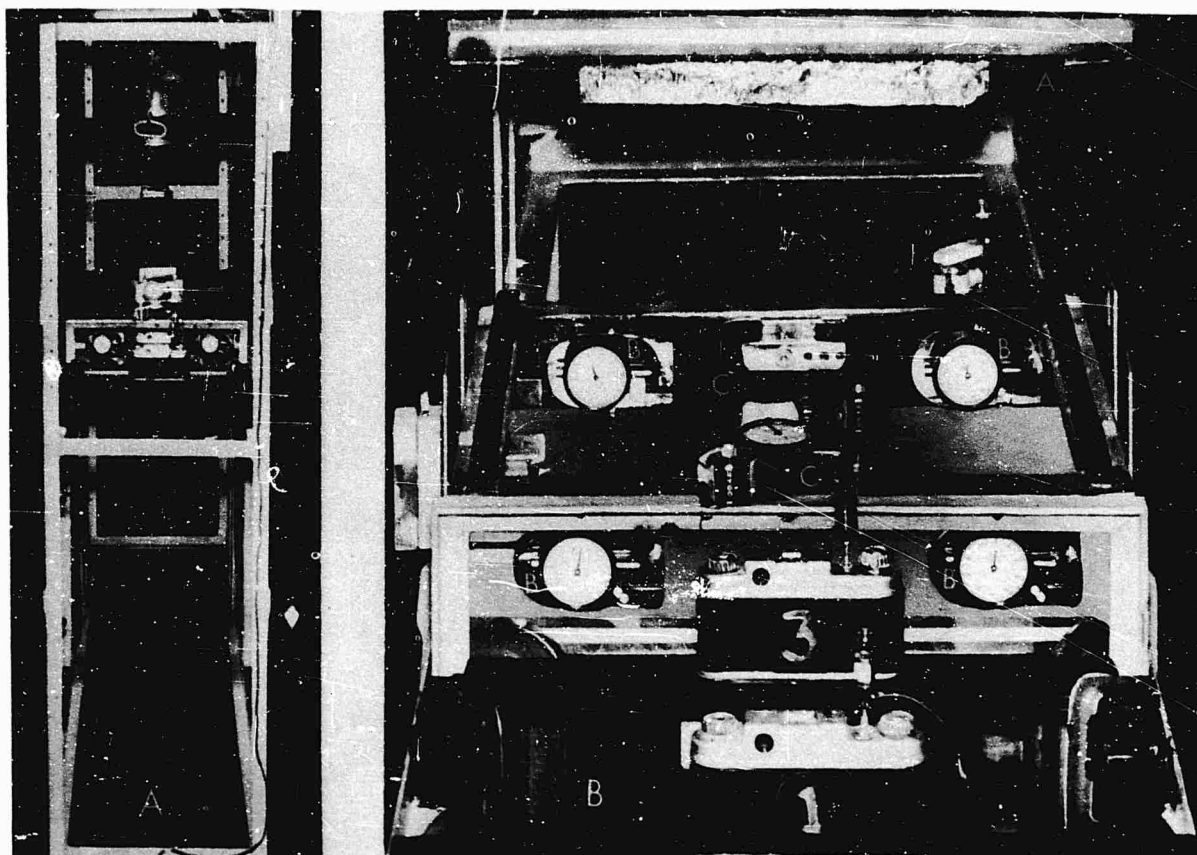
Figure 27. End and Detail Views of Hand-Force Apparatus. A—View of left hand end of welded support, pressure gauges, and camera. B—The seat (A) has been lifted to show a more detailed view of four pressure gauges (B) which bear the weight of the seat; in the middle of the area below the seat are gauges (C) which record fore-and-aft seat forces. Solenoid-operated cameras marked No. 3 and No. 1 are shown below. Note that a counter appears in the view of each camera.
