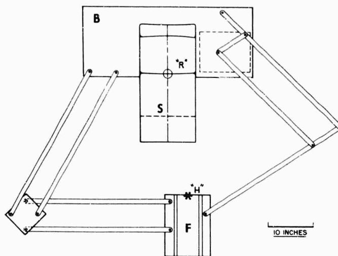
Figure 18. Floor Plan of Linkages for Foot-Range Determinations.
