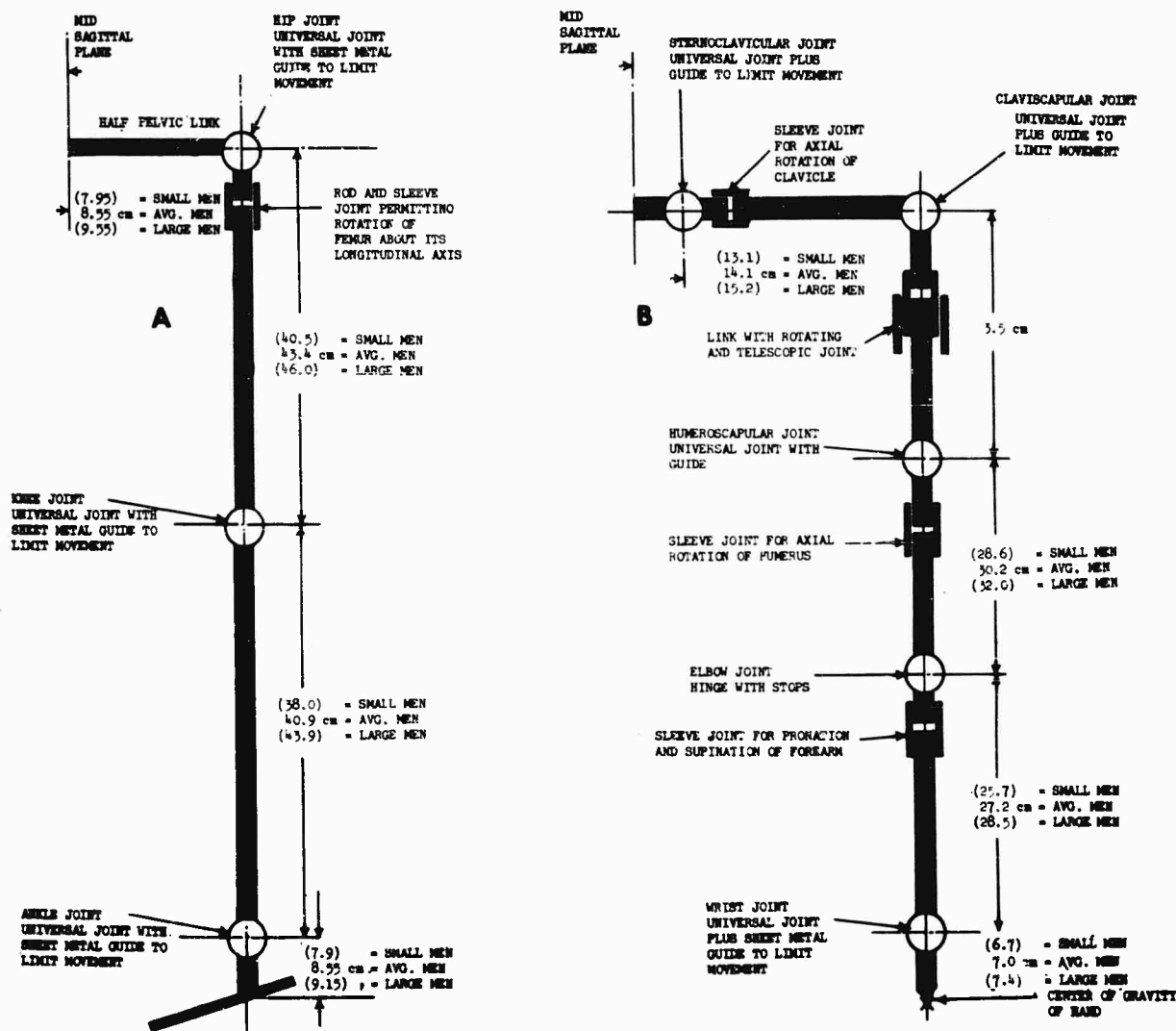
Figure 57. General plan of linkage assembly for the lower (A) and upper (B) limb systems.
