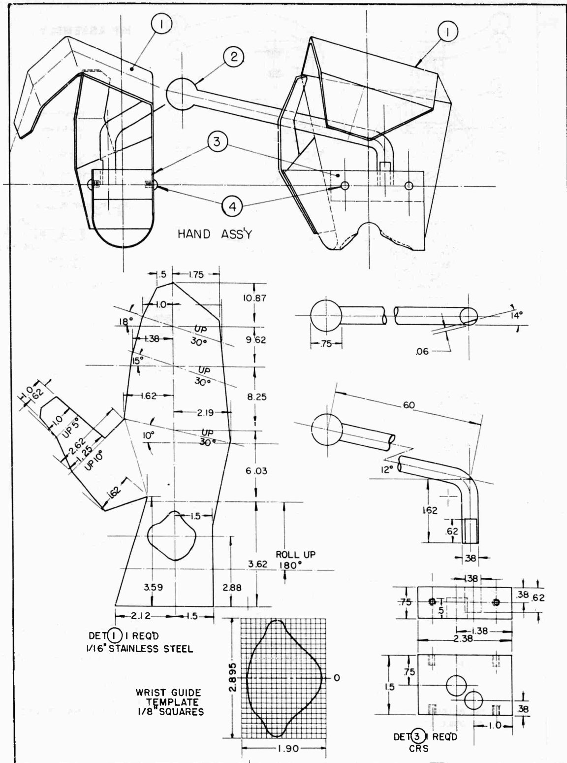
Figure 63. Details of plans for hand and wrist joint assemblies.
