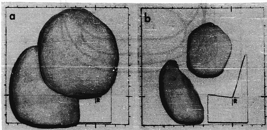
Figure 91. Models of side view of work space. A-Dimensions scaled to 95th percentile of hand and foot movements of muscular and medium subjects. B-Dimensions scaled to the 5th percentile. Tick marks are at 6-inch intervals relative to the seat "R" point.
