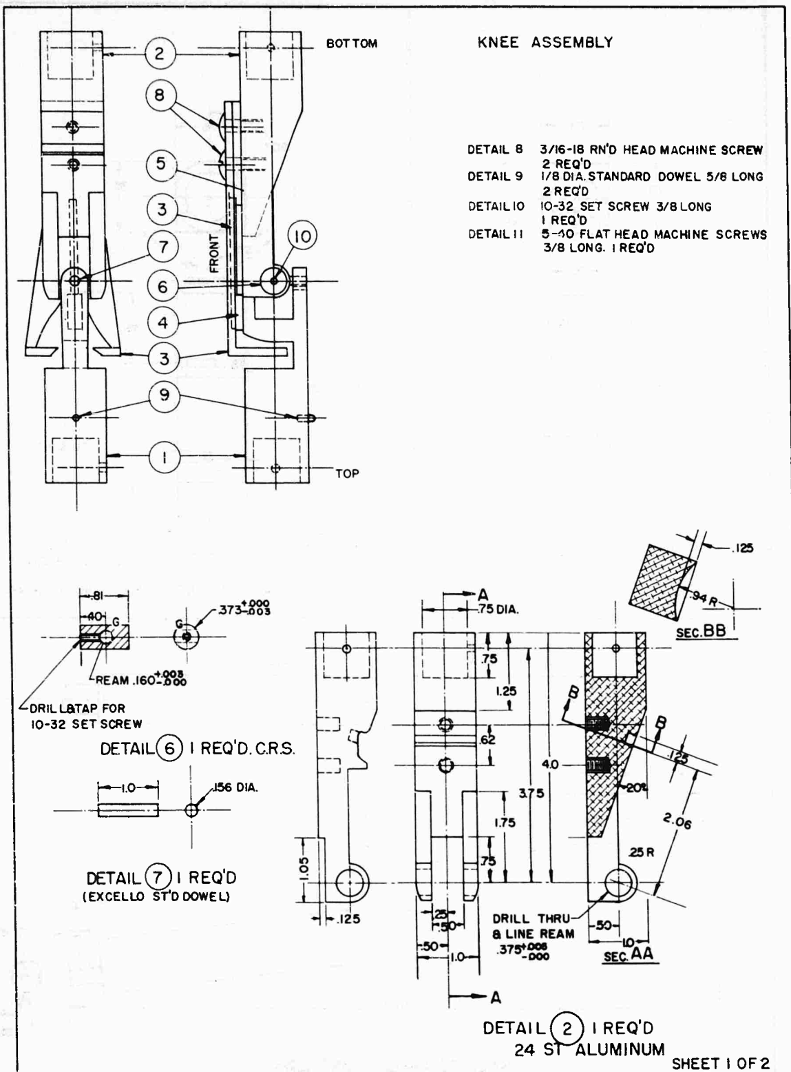
Figure 66. Plan for knee joint model.
