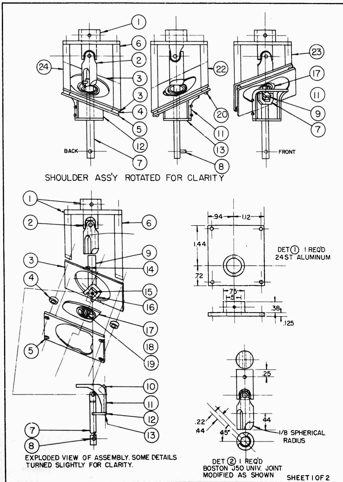
Figure 60. Plan for model of combined shoulder joints.
