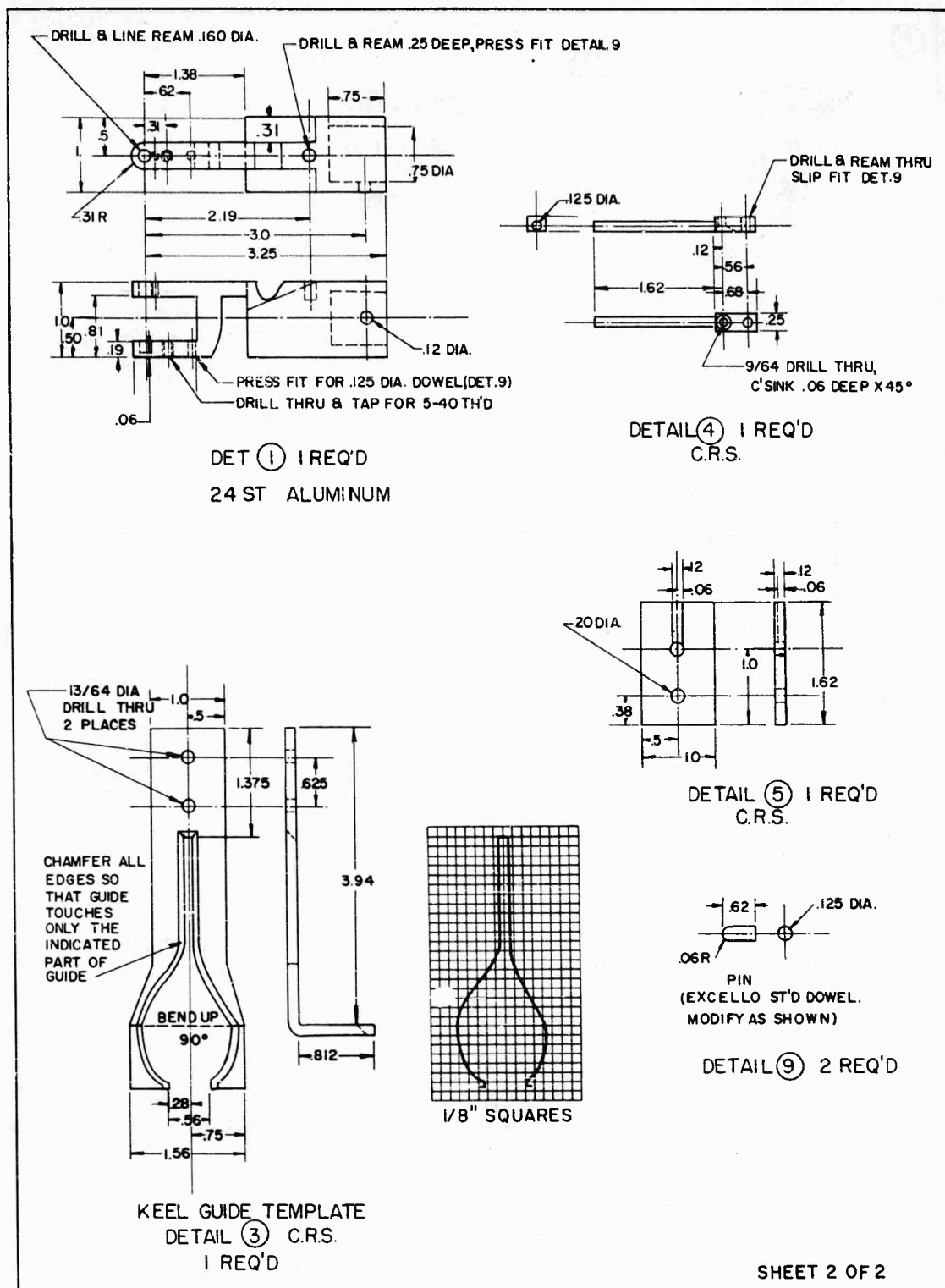
Figure 67. Details of plan for knee joint model.
