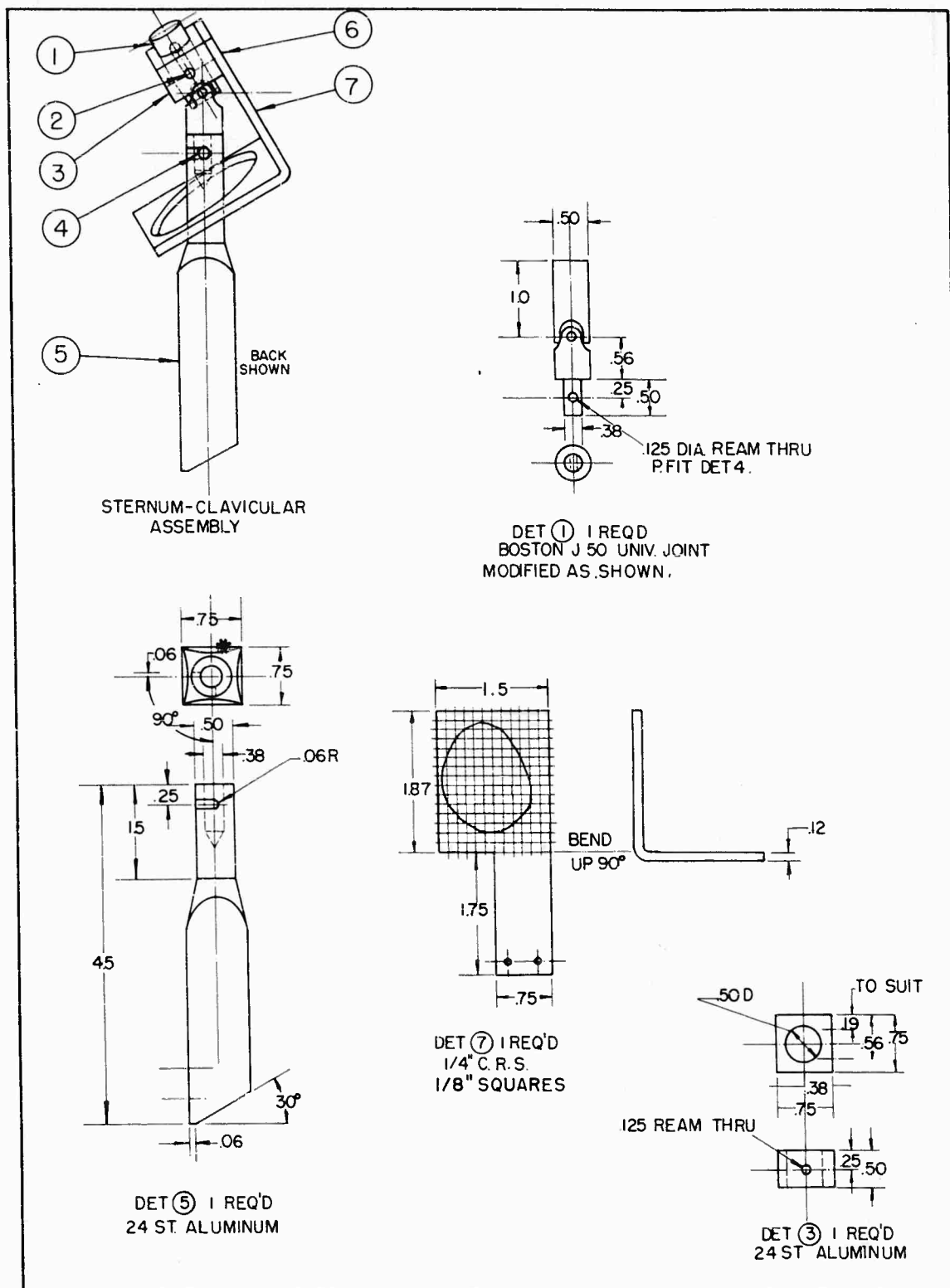
Figure 59. Plan for model of sternoclavicular joint.
