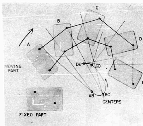
Figure 7. Method for Locating Instantaneous Centers. Reuleaux (1875) Method for locating instantaneous centers of rotation. The heavy lines representing successive phases of a movement show the relative motion of two points on the moving part. Mid-interval normals intersect at points AB, BC, etc. These points momentarily and in sequence are centers about which angular motions of the moving part occur.
