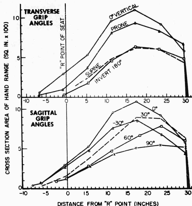
Figure 75. Plots showing frontal plane areas available to different orientations of the hand at various distances from the "R" point of the seat.
