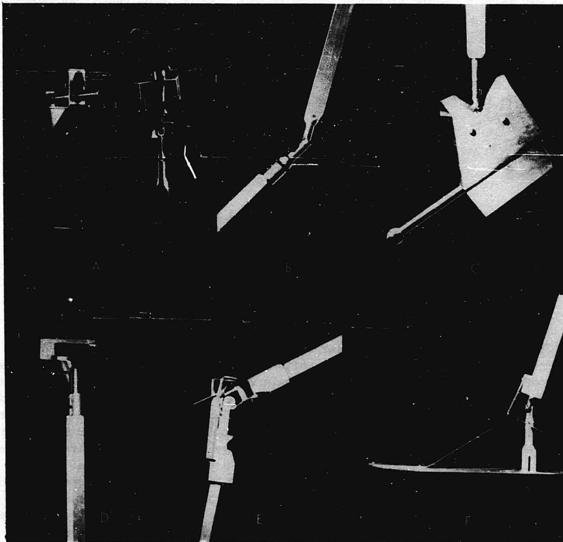
Figure 58. Photographs of machined joints of the upper and lower limbs. A-steroclavicular, claviscapular, and glenohumeral joints. B-elbow hinge and forearm sleeve joints. C-wrist universal joint with hand shape and grip axis. D-universal and sleeve joint of hip assembly. E-knee joint. F-ankle universal and foot assembly.
