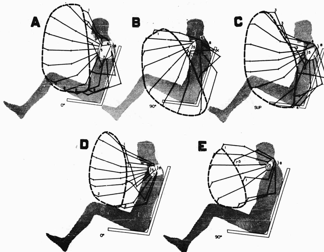
Figure 80. A link analysis of sagittal sections through kinetospheres based on motion picture records. At A, B, and C sections are at left shoulder level; at D and E midsagittal sections are represented.
