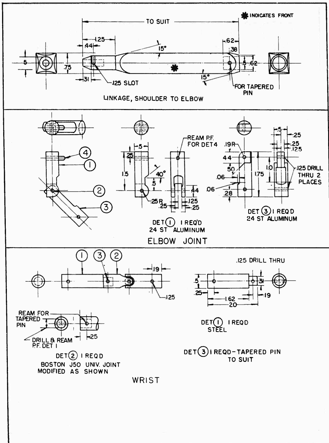
Figure 62. Plans for arm link and for elbow, forearm, and wrist joints.
