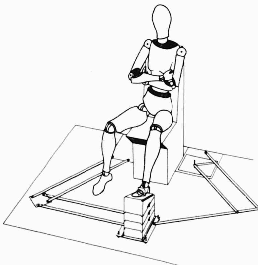
Figure 17. Setup for Determining Horizontal Foot Range. Arrangement of subject, seat, foot rest, and linkages for determining foot range at a given horizontal level relative to the floor. The linkage on the subject's right continually directs the foot forward; that on his left is a 1:5 pantograph. The blocks below the foot show that the heel is raised 9 inches and the foot is tilted 30^\circ above horizontal.
