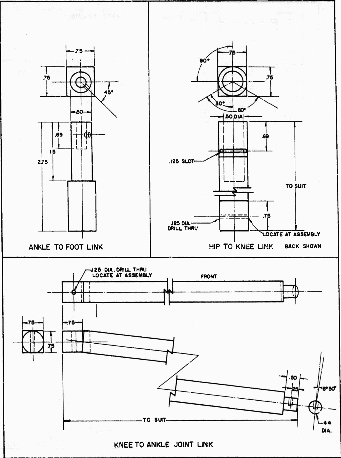
Figure 65. Plan of lower limb links for models.
