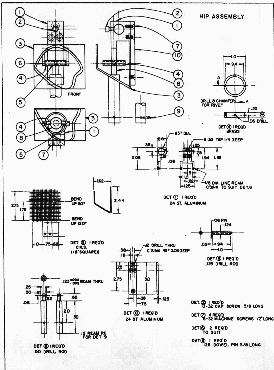
Figure 64. Plan for hip joint model.
