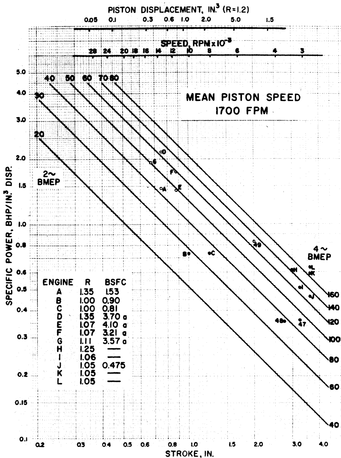
FIG.12 SPECIFIC POWER VS SIZE FOR VARIOUS VALUES OF BMEP AT CONSTANT PISTON SPEED
